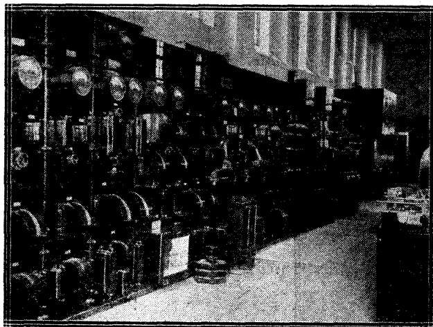
The low-tension switchboard in the valve room at the Rugby wireless station.
