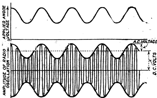
Fig. 8.—A form of modulation similar to that shown in Fig. 7. Here, however, the D.C. voltage is greater than the superimposed alternating potential.
