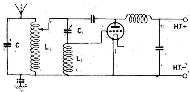
Fig. 6.—In this circuit, in which electrostatic reaction is operative, the condenser C_1 should have a small value.
