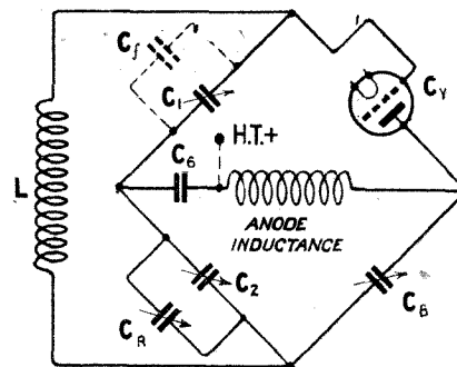
Fig. 5.—The circuit of Fig. 2 re-drawn in "bridge" form, to indicate the action of the method adopted for stabilisation.
