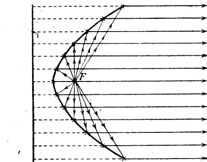
Fig. 1.—A sketch and plan diagram of one system adopted for beam transmission, vertical wires of equal length being hung round a parabolic support, with the transmitting apparatus at the focal point.
