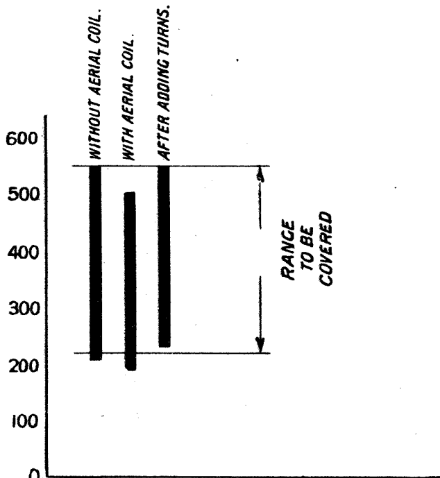
Fig. 1.—Showing the alterations effected in the tuning range of a receiver by changes in the aerial coil.
