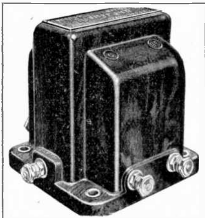
The redesigned Telsen "Radiogrand" transformer with its polished bakelite case and earthing terminal.
