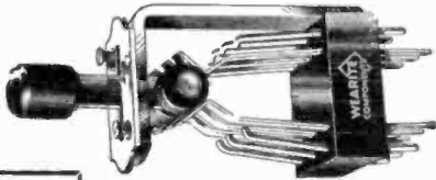
Wearite Anti-capacity Switches, 1 to 6 way as used in most popular sets. Can be supplied lever controlled or ganged.
