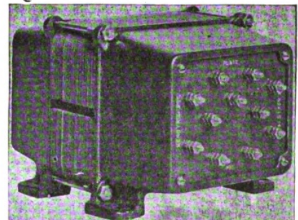
Figure 19—UP-1016 Amateur radio plate and filament transformer. Rear view showing the terminal board
