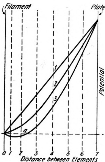
Figure 8—Potential distribution in the Kenotron under various filament temperatures
