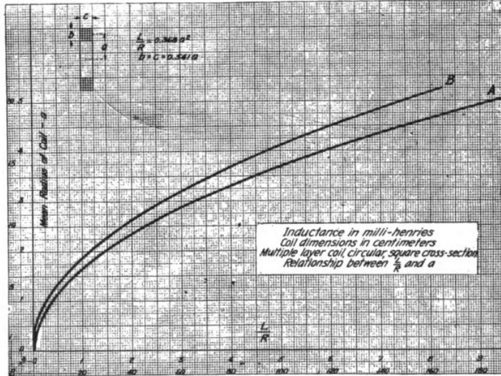
Figure 3—Graph for mean radius of coil
