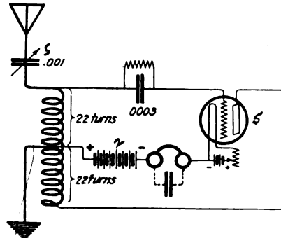
Figure 1—Receiving circuit that simplifies tuning
