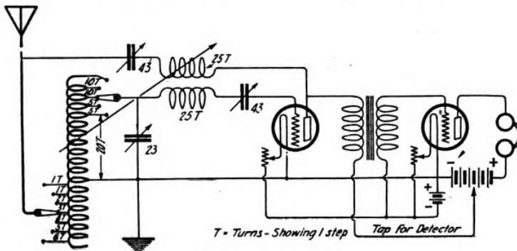
Hook-up of receiver
