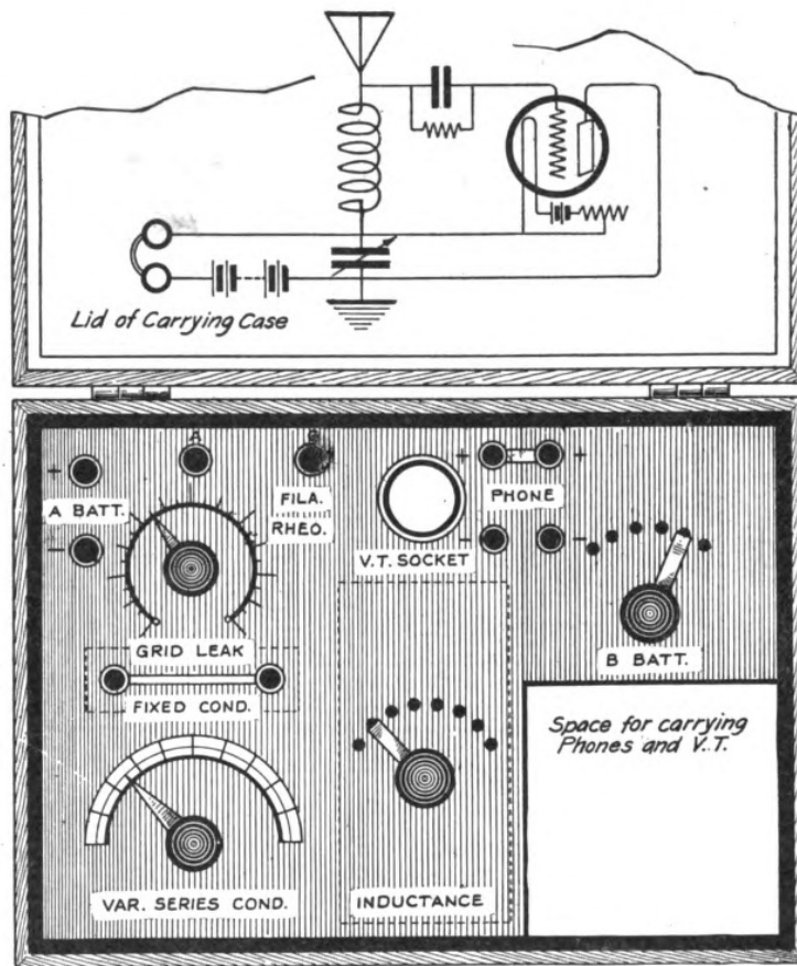
The portable radio set assembled
