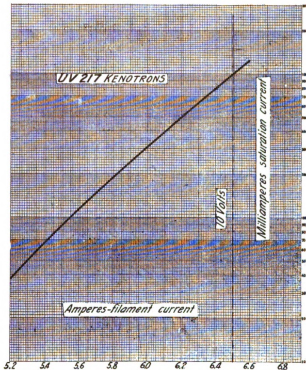
Figure 5—Saturation current graph
