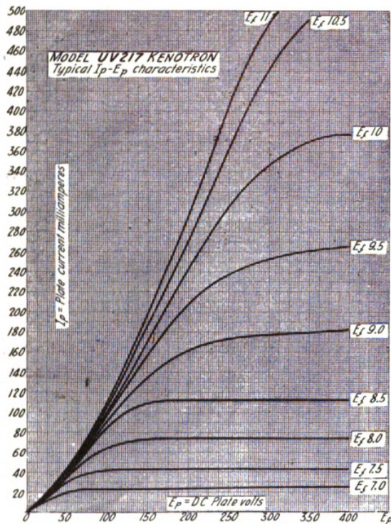
Figure 6—Volt ampere characteristics showing limitation of current due to temperature
