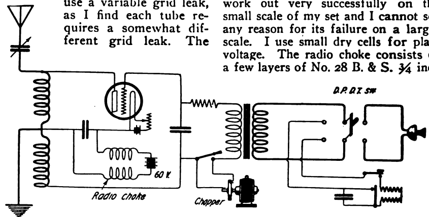
Figure 2—Hook-up for the transmitting set
