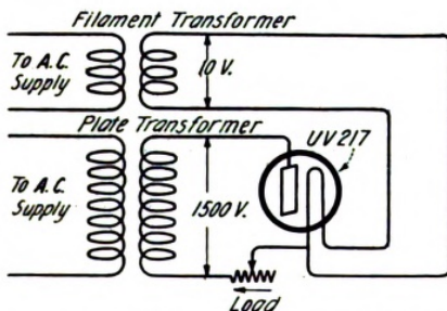
Figure 16—Circuit for half-wave rectification
