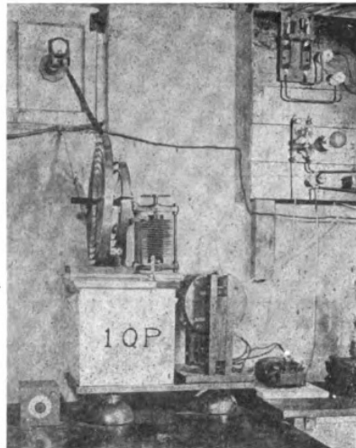
Quenched gap transmitter
