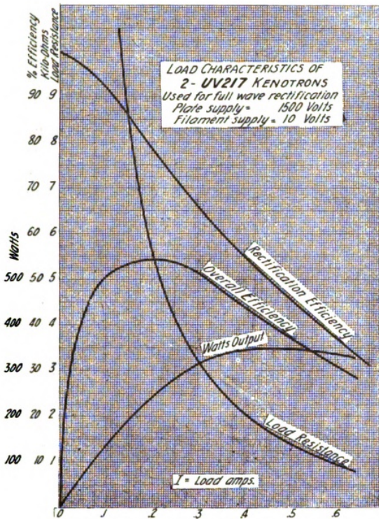
Figure 14—Load characteristics
