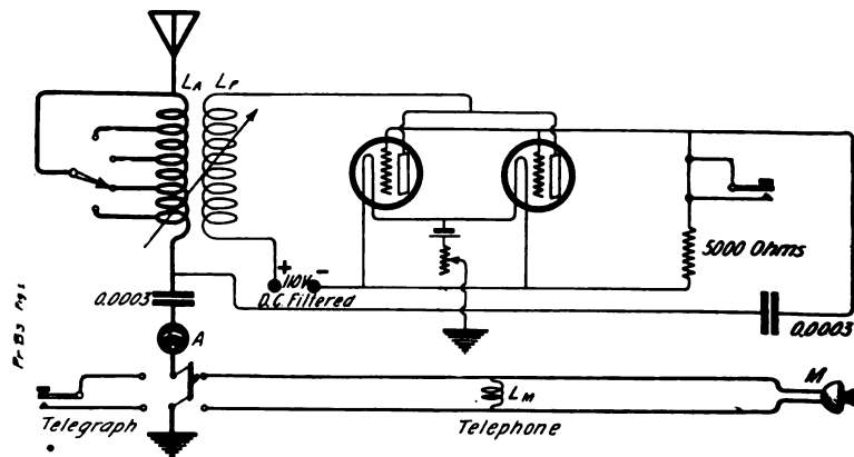
Figure 1—The complete transmitting circuit excluding the filter
