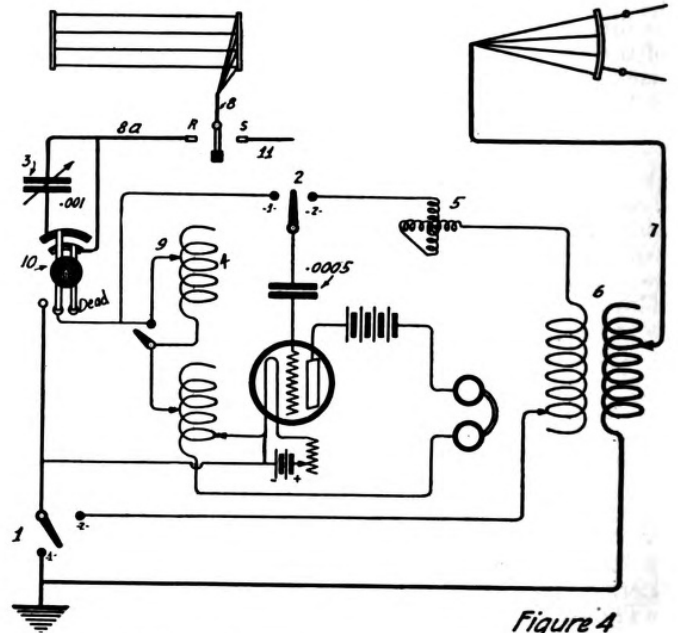
Various circuits for short, medium and long wave reception
