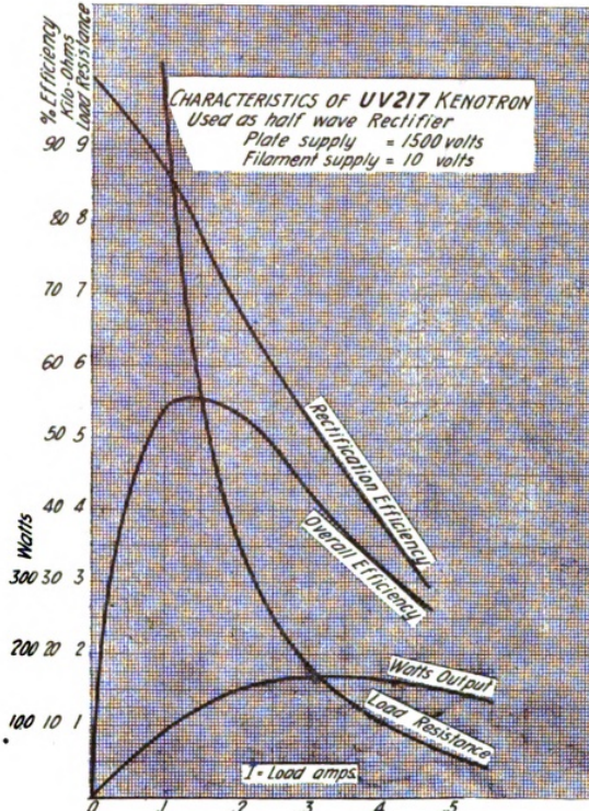
Figure 15—Load characteristics
