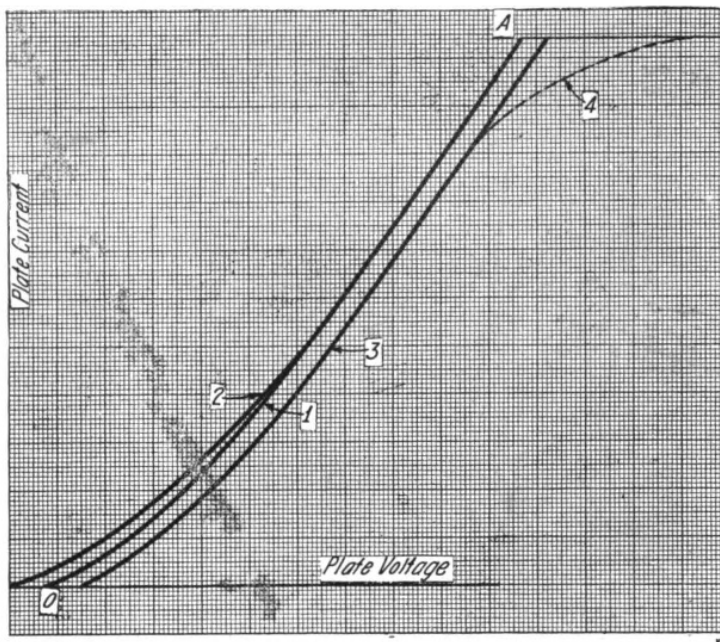
Figure 9—Modifying factors of the characteristic curve
