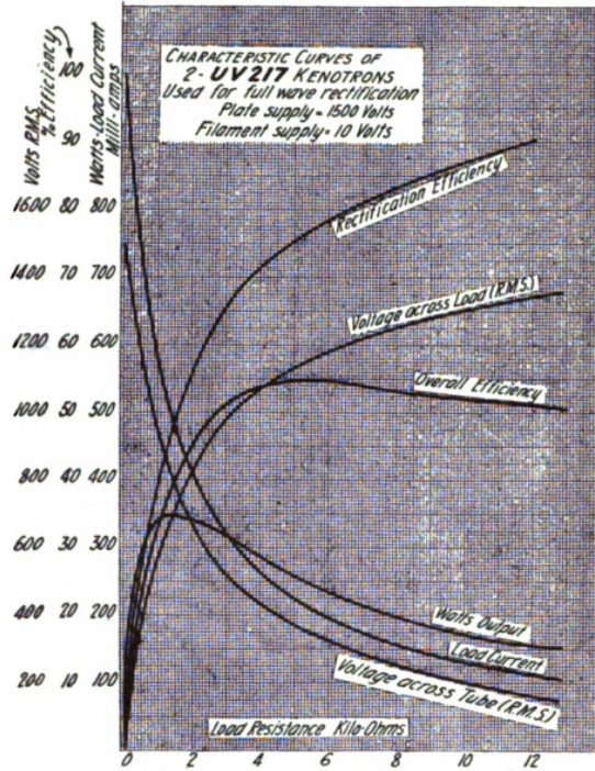
Figure 13—Load characteristics
