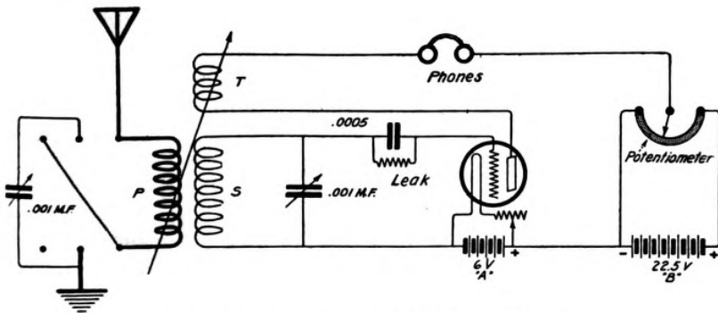
Figure 2—Hook-up for best results of vario-coupler
