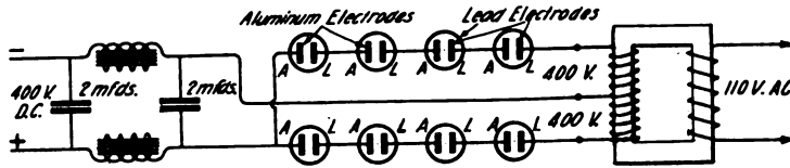
Figure 3—Hook-up of the electrolytic rectifier
