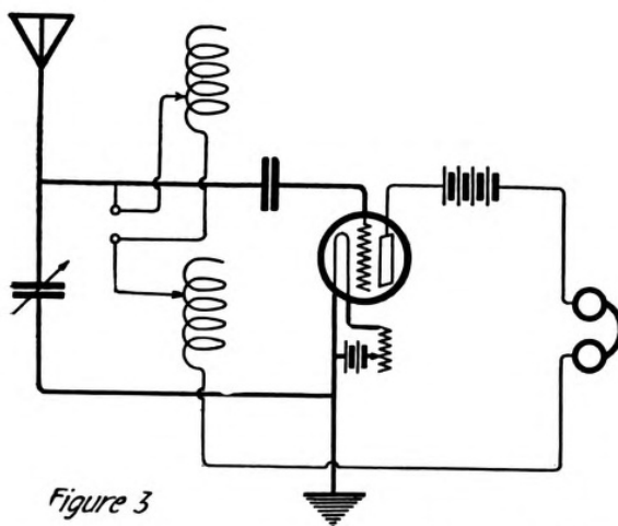
Various circuits for short, medium and long wave reception
