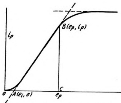
Figure 11—Section AB characteristics
