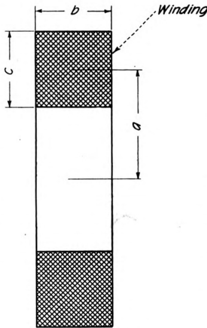
Figure 5—Coil design
