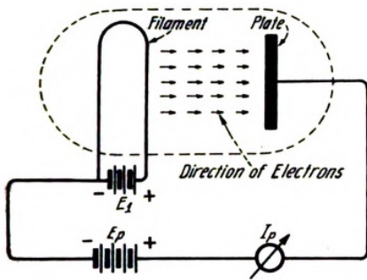
Figure 4—Circuit to determine relation between filament and plate currents
