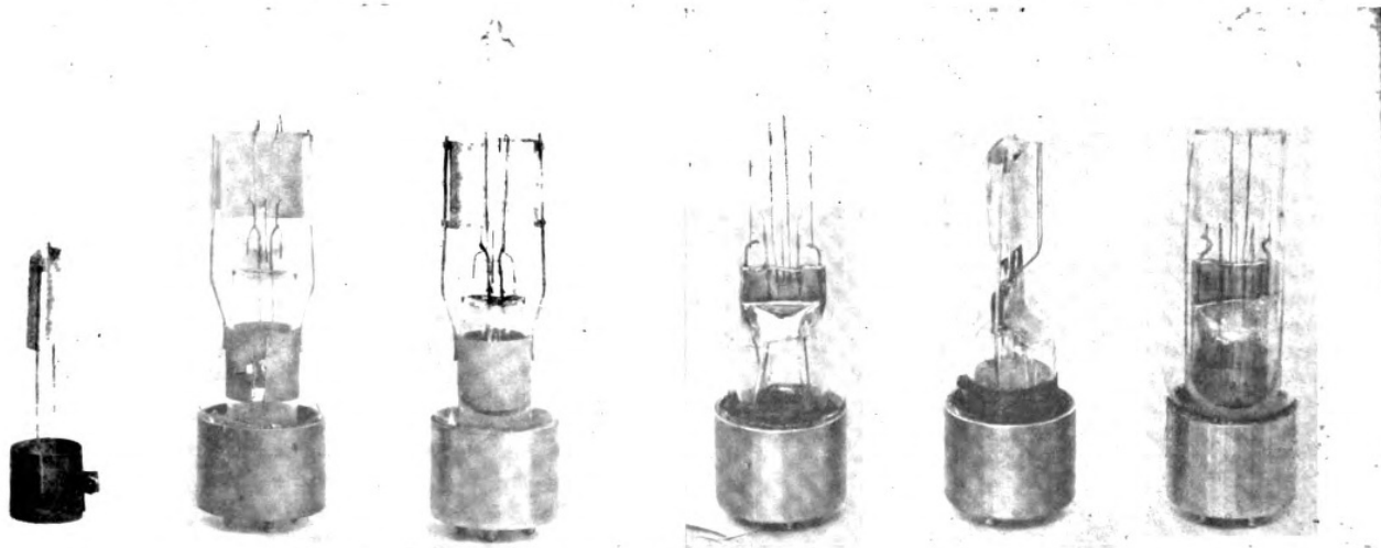
Figure 1—UV-217 Kenotron having a rated D. C. output of 150 watts at 1000 volts. Center view has one-half of plate cut away to show the filament
