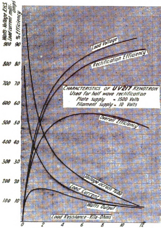
Figure 12—Load characteristics
