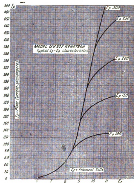
Figure 7—Volt ampere characteristics showing effect of space charge in limiting the electron current
