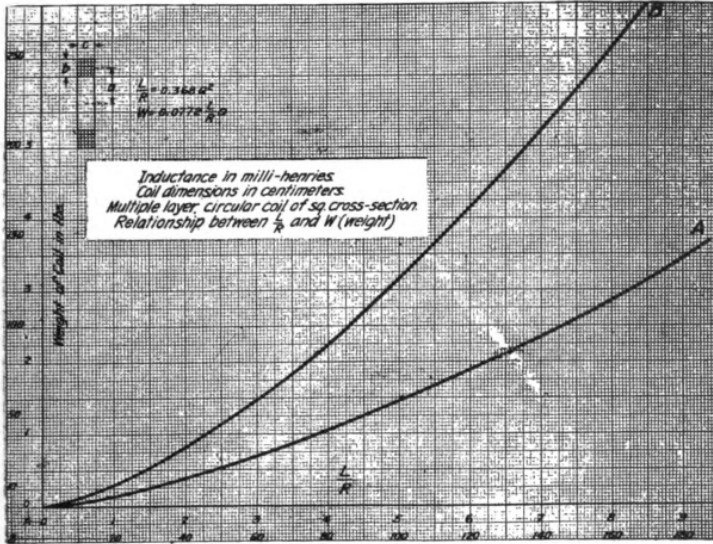
Figure 4—Graph for weight of coil in lbs.
