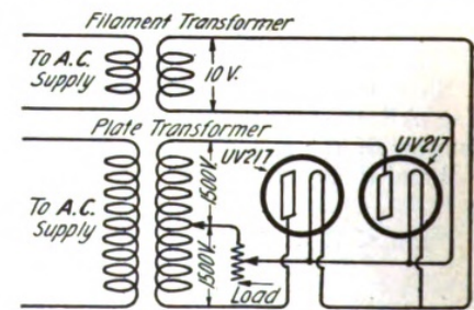
Figure 17—Circuit for full wave rectification
