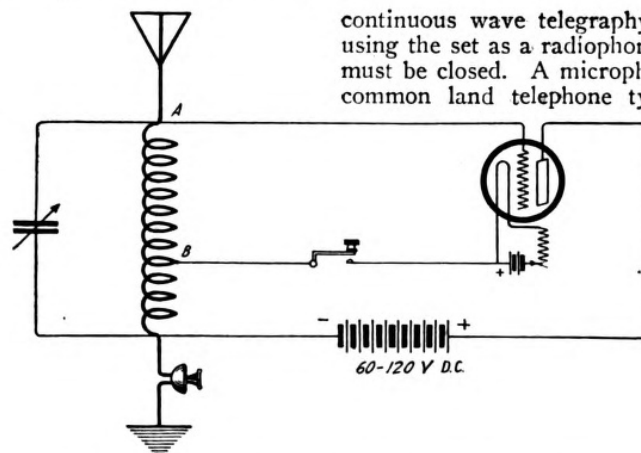
Figure 1—Circuit diagram of a simple CW transmitter
