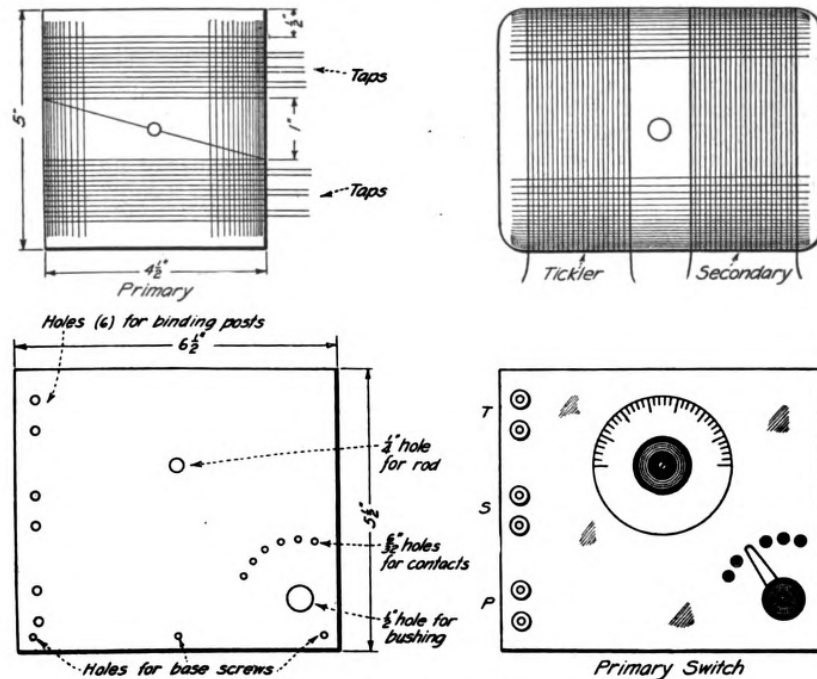
Figure 1—Constructional details of the vario-coupler
