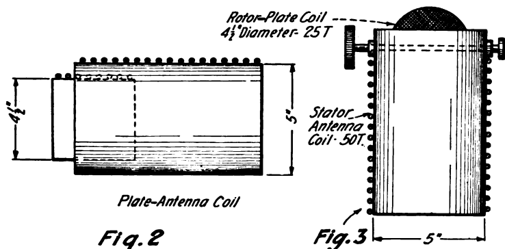
Constructional dimensions of two types of plate antenna coil
