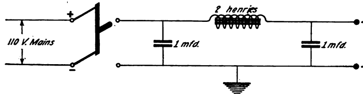
Figure 4—The filter circuit
