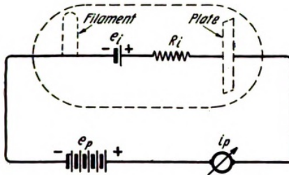
Figure 10—Circuit arranged with space charge effect equal to a counter-electromotive force
