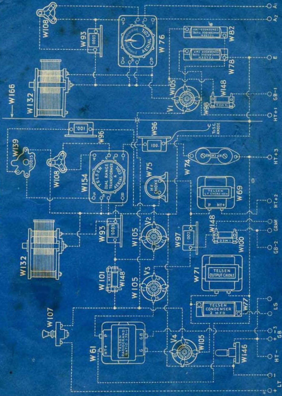
WIRING DIAGRAM
