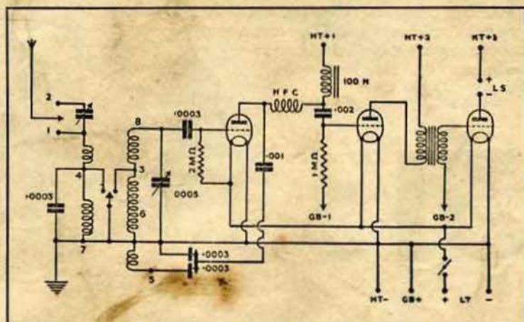
The theoretical circuit of the Telsen "Conqueror" 3.
