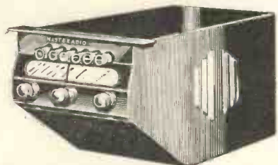
One of the new car radios built by Masteradio, which is an 8 stage all-wave superhet they have 11 stations press-button control, also motor wave changing, high-speed motor tuning and locked
