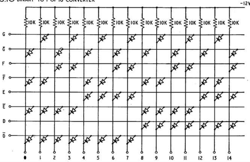
FIG. 10 BINARY TO 1 OF 16 CONVERTER
