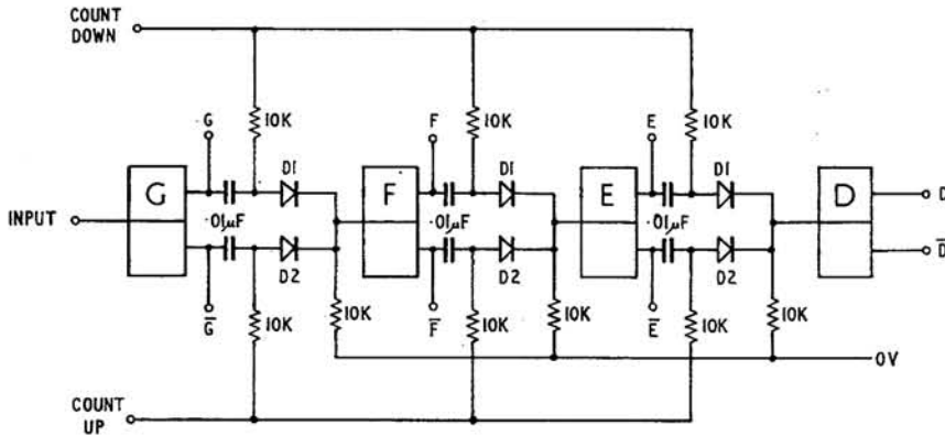
FIG. 9 COUNTER WITH DIRECTION CONTROL
