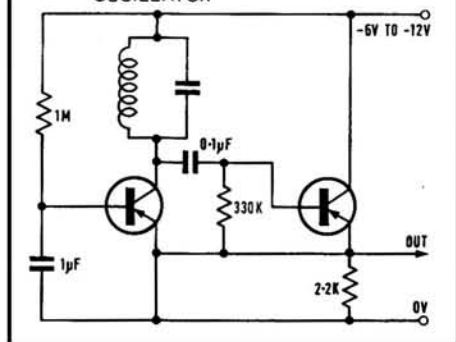
FIG. 3 EMITTER-COUPLED SINE-WAVE OSCILLATOR
