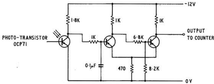
FIG. 13 PHOTO-TRANSISTOR AND SCHMITT TRIGGER
