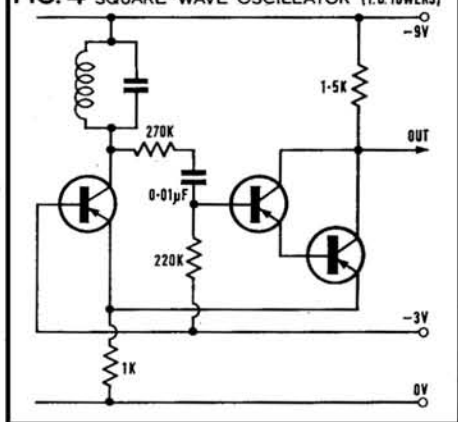
FIG. 4 SQUARE-WAVE OSCILLATOR (I.D. TOWERS)
