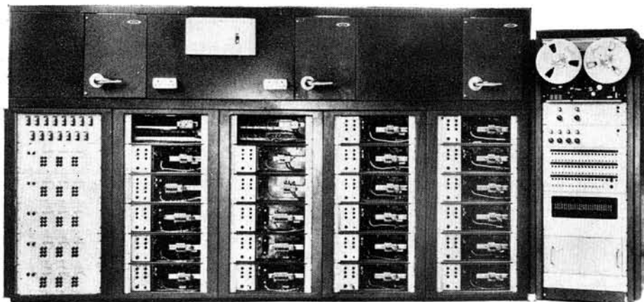
Four-track TRD tape-recorder feeds an automatic programmed unit at Caernarvon Castle. See 'Caernarvon Son et Lumière'
