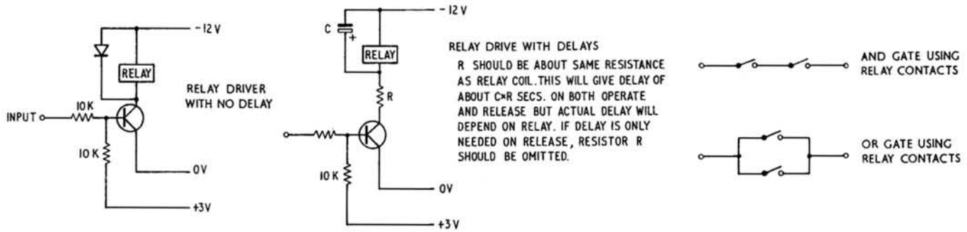
FIG. 16 EXAMPLES OF RELAY LOGIC
