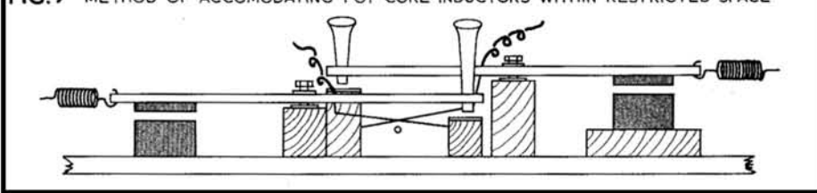
FIG. 7 METHOD OF ACCOMODATING POT CORE INDUCTORS WITHIN RESTRICTED SPACE
