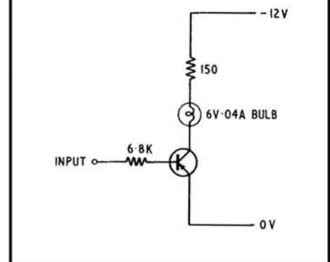
FIG. 17 INDICATOR CIRCUIT
