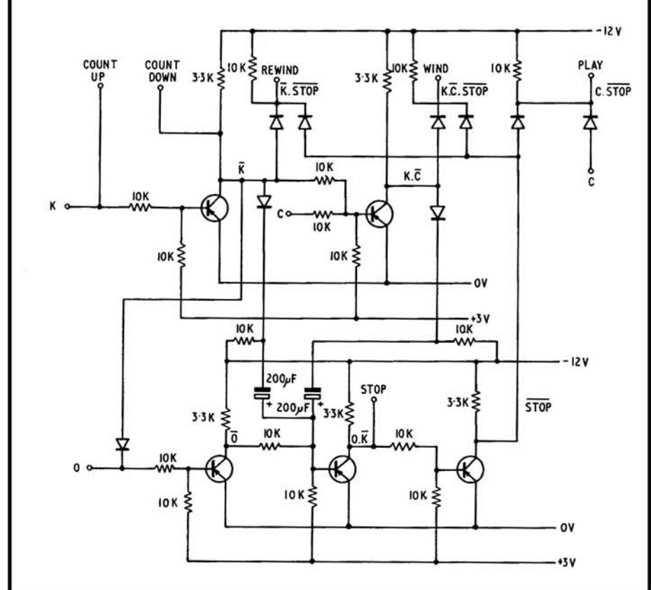
FIG. 15 TAPE DECK CONTROL CIRCUIT (WITH DELAYS)
