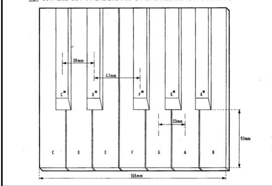
FIG. 6 STANDARD KEYBOARD DIMENSIONS FOR ONE OCTAVE. CONVENTIONAL KEYBOARDS ARE NOT SUITABLE BUT DIMENSIONS AND SPACIAL RELATIONSHIPS MATTER.
