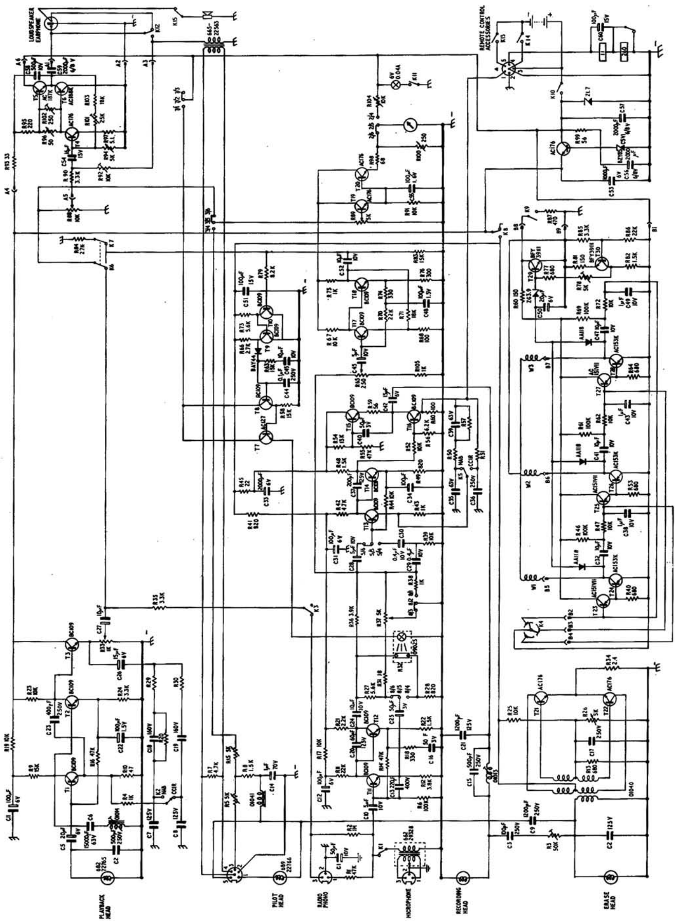
FIG. 1 UHER 1000 PILOT CIRCUIT DIAGRAM
