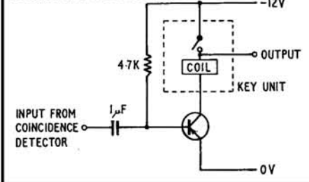
FIG. 12 KEY PRESSED AND COINCIDENCE DETECTORS
