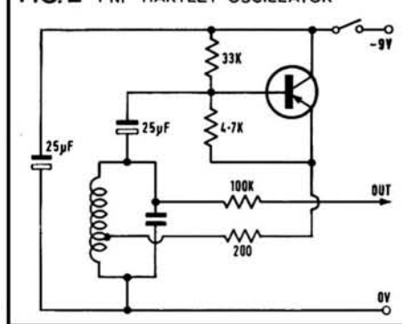
FIG. 2 PNP HARTLEY OSCILLATOR
