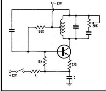
FIG. 8 METHOD OF ARRANGING TUNER ADJUSTMENT OF LC OSCILLATOR WHEN IT IS INCONVENIENT TO VARY INDUCTANCE.
