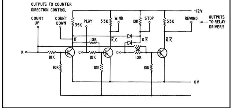
FIG. 14 TAPE DECK CONTROL CIRCUIT (WITH NO DELAYS)
