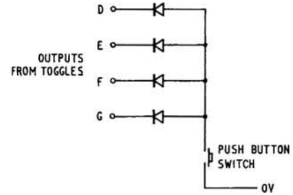
COUNTER RESET CIRCUIT
