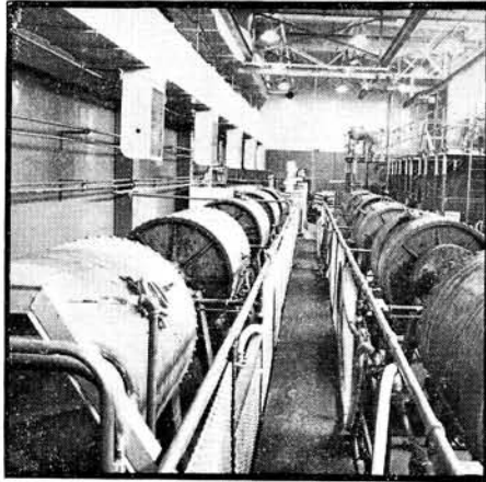
Ball mills
