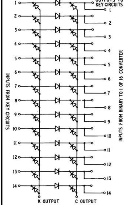
FIG. 12 KEY PRESSED AND COINCIDENCE DETECTORS
