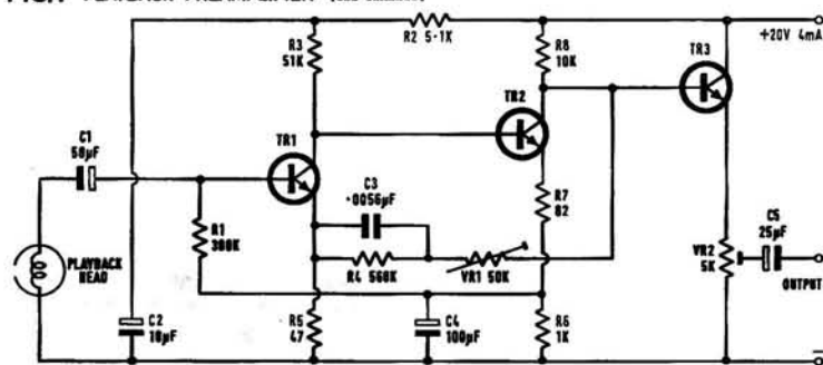
FIG.1 PLAYBACK PREAMPLIFIER (ONE CHANNEL)
