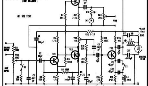
FIG.2 RECORD AMPLIFIER (ONE CHANNEL)
