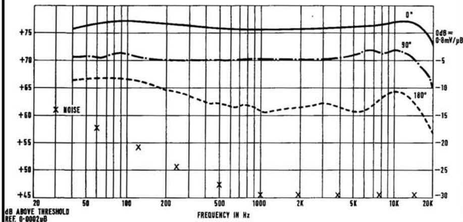
FIG. 2 FI-CORD FC650 CAPACITOR MICROPHONE (200 OHMS IMPEDANCE)
