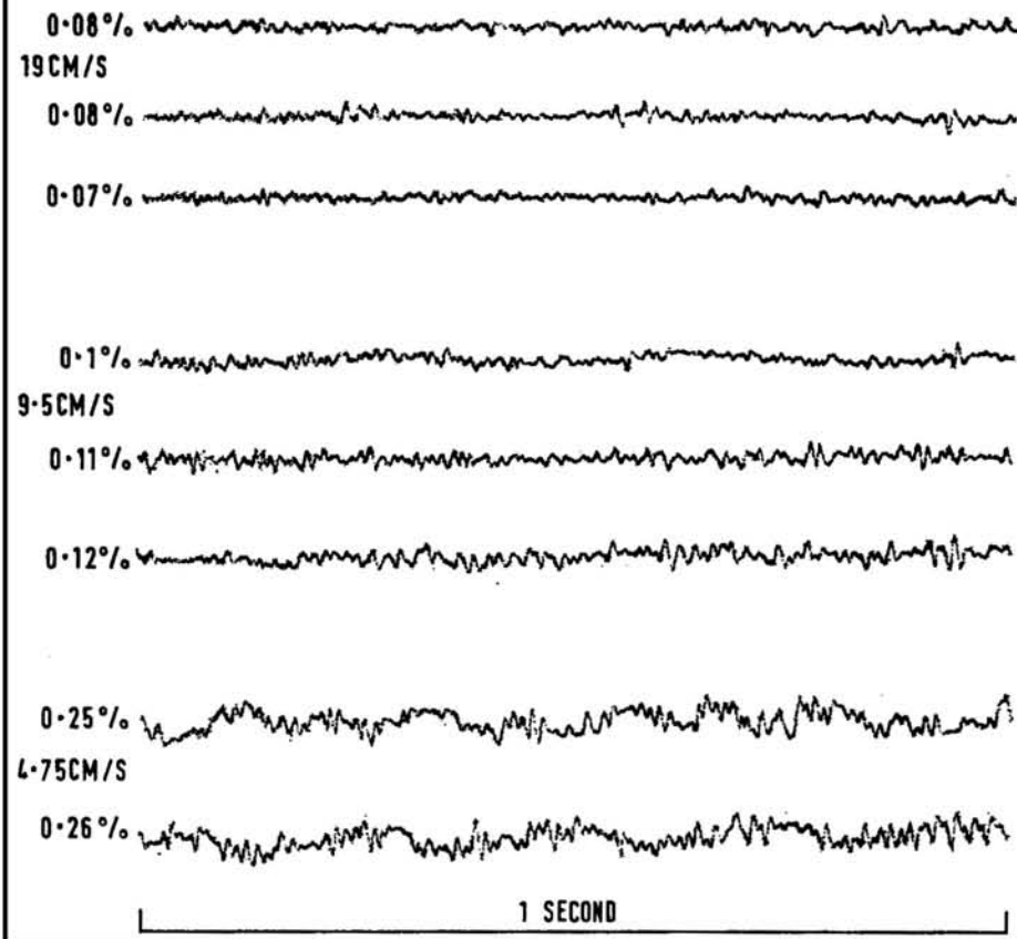
FIG. 2 TRUVOX PD202 RECORD / PLAY WOW AND FLUTTER
