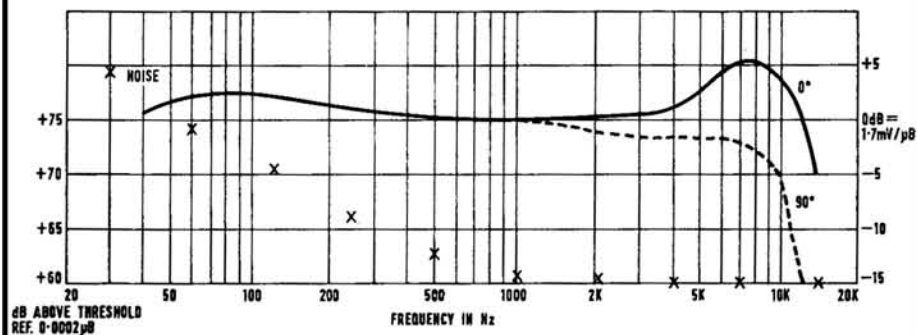
FIG. 2 FI-CORD FC650 CAPACITOR MICROPHONE (200 OHMS IMPEDANCE)
