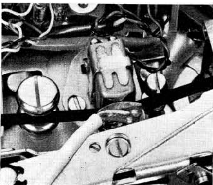
Close-up of the Tandberg 6X cross-field system. Bias head in foreground.
