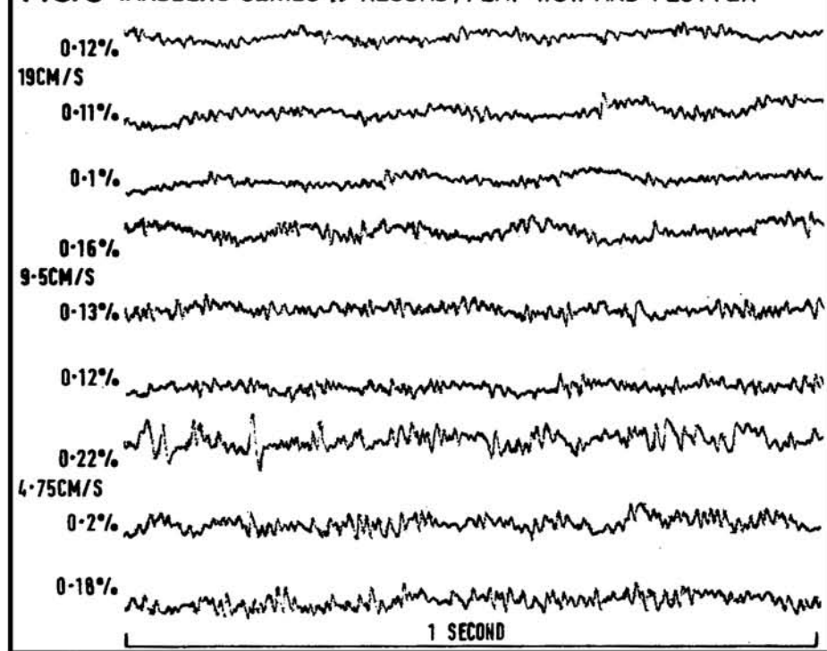
FIG. 3 TANDBERG SERIES II RECORD/PLAY WOW AND FLUTTER
