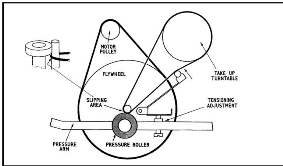
Fig. 4. Telefunken belt drive.
