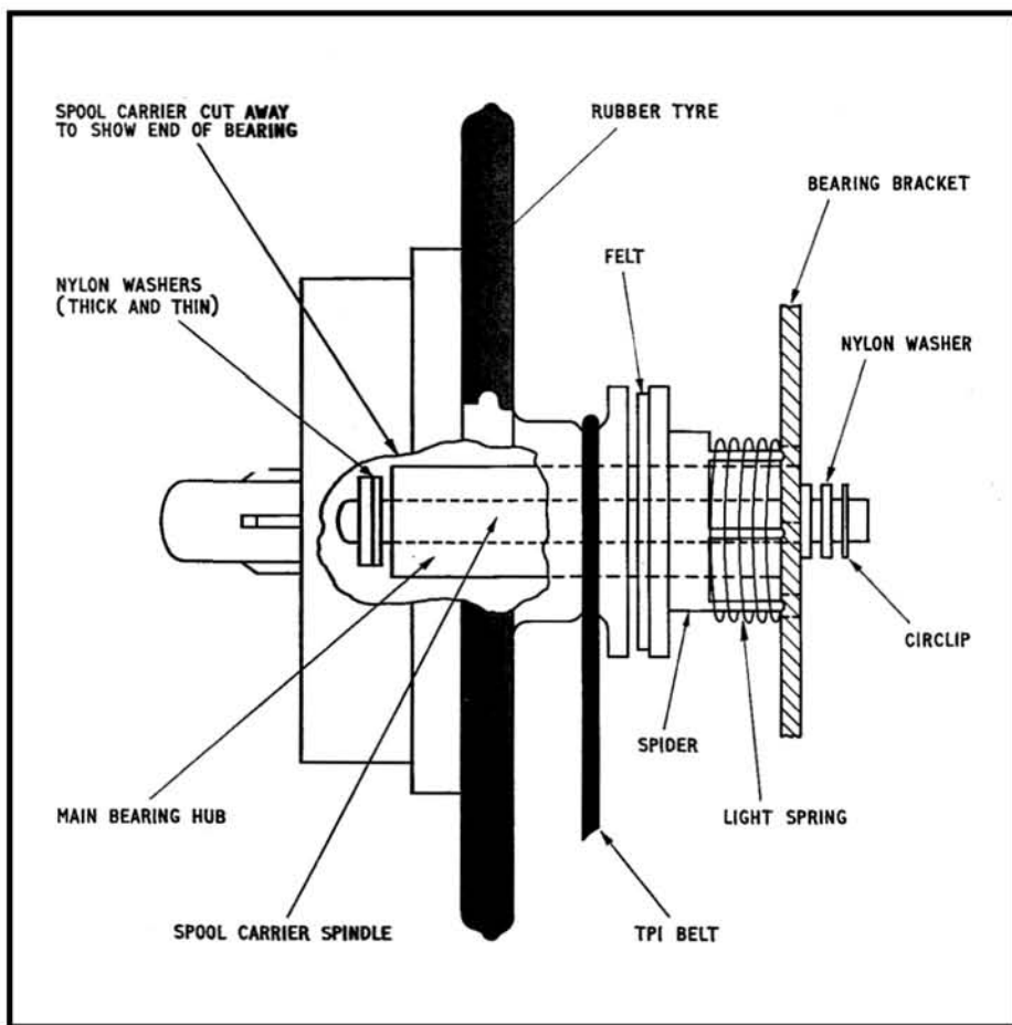
Fig. 5. Van der Molen vertical take-up clutch.
