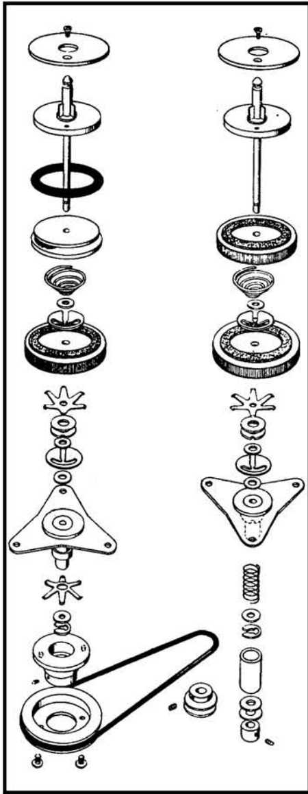
Fig. 6. Exploded view of Akai clutch.
