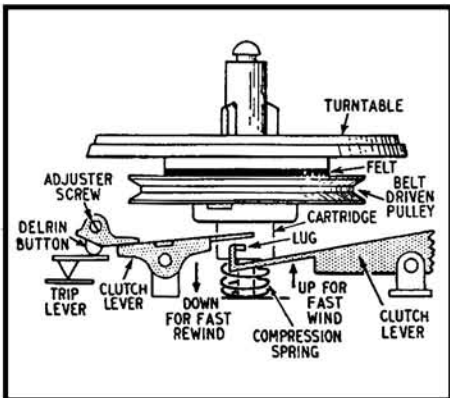
Fig. 7. Tandberg clutch system.
