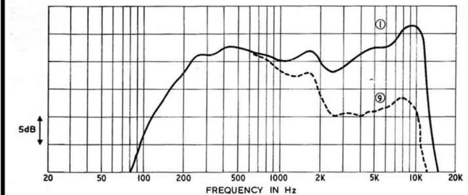
FIG. 5 GRUNDIG GDM 312 MICROPHONE (HIGH-Z)
