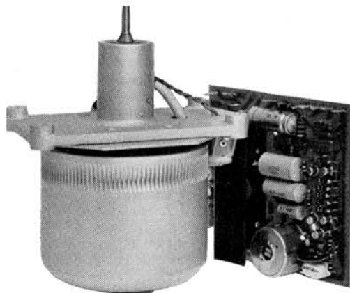
Fig. 1. Capstan motor and control circuit board. The tachometer head mounting, though not the head itself, is visible on the right of the rotor.
