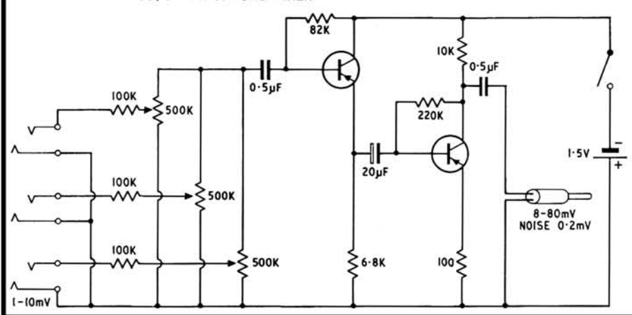
FIG. 1 GRAMPIAN 20/3 MICROPHONE MIXER
