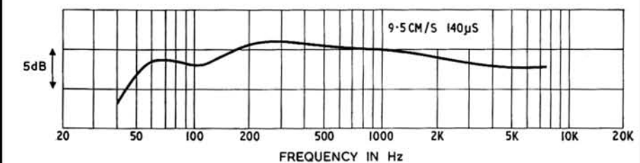
FIG. 3 GRUNDIG TKI45 RECORD/PLAY RESPONSE (LINE IN TO LINE OUTPUT)
