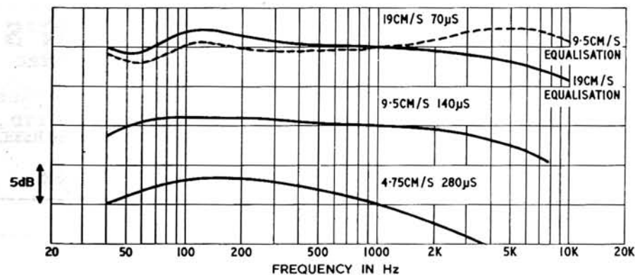
FIG. 2 AMPEX 753 PLAY-ONLY RESPONSE (TEST TAPE TO LINE OUTPUT)
