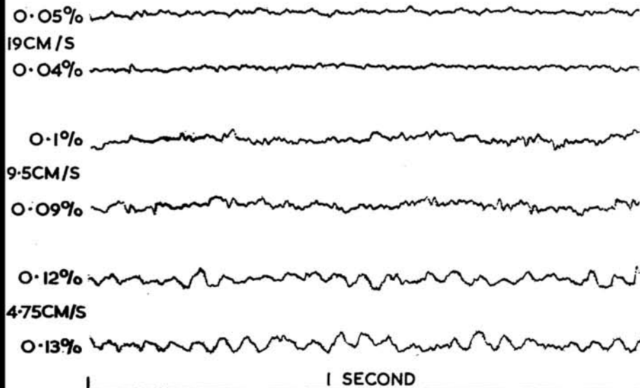
FIG. 1 AMPEX 753 RECORD / PLAY WOBBLE
