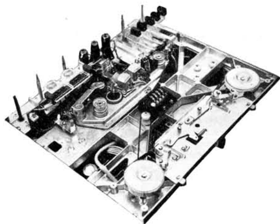
Fig. 3. Upper view of mechanism with deck covers removed. Solenoid switch levers can be seen at top corner. Braking is similar to the 736 steel bands acting on cloth. The pinch wheel bracket is mounted away from the head channel to give greater access when editing.
