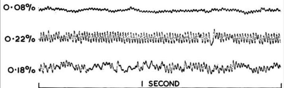
FIG. 2 GRUNDIG TKI45 PLAY-ONLY RESPONSE (TEST TAPE TO LINE OUTPUT)
