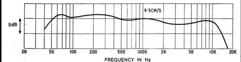
FIG. 4 GRUNDIG TKI45 ACOUSTIC RESPONSE (WHITE NOISE ON SPEAKER AXIS)
