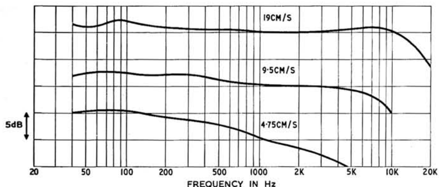
FIG. 3 AMPEX 753 RECORD / PLAY RESPONSE (LINE IN TO LINE OUTPUT)
