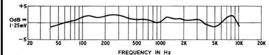
FIG. 5 GRUNDIG GDM 312 MICROPHONE (HIGH-Z)
