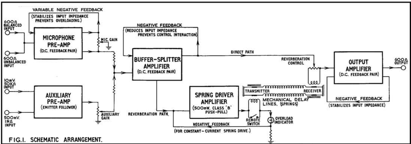
FIG. 1. SCHEMATIC ARRANGEMENT.
