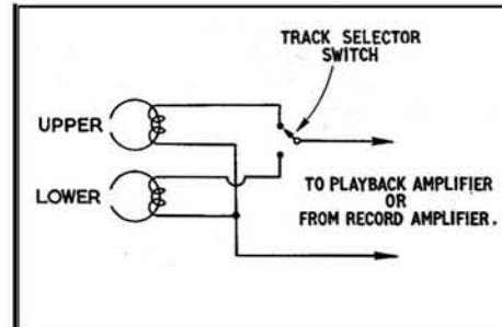
Fig. 6. Typical \frac{1}{2} -track head switching arrangement.
