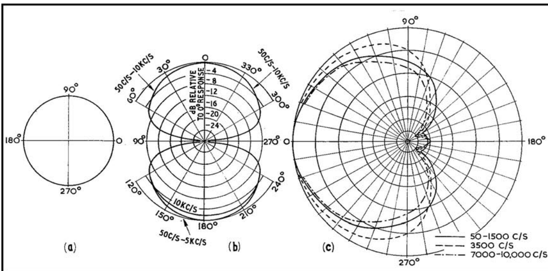
Fig. 1: (left) shows the polar response of an omnidirectional (a) bi-directional (b) and cardioid (c) microphone. Note that response varies slightly with frequency.
