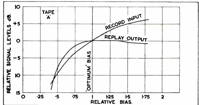
Fig. 2. Shows how change of bias also changes tape sensitivity.
