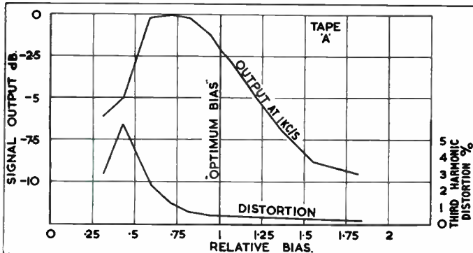
Fig. 1. Displays "optimum bias". The lower curve shows the third harmonic distortion factor, and the upper curve shows the output, as bias is altered.
