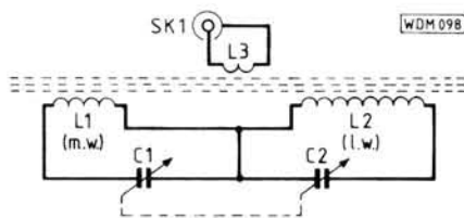
Fig. 2: Circuit diagram of antenna
