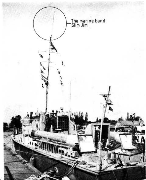
Fig. 1.3: Close up of Marine band "Slim Jim". The split metal sleeve a third of the way up the antenna, serves as an adjustable matching capacitor
