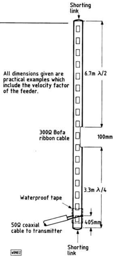
Fig. 3: "J-match" vertical for 21MHz band. Antenna can be supported in the same manner as 5\lambda/8 antenna
