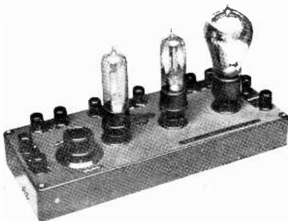
FIG. 34. IGRANIC 3-VALVE RESISTANCE CAPACITY AMPLIFIER
