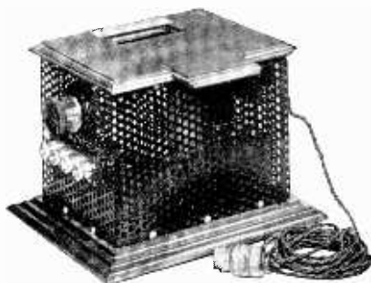
FIG. 2. THE ELVEN MAINS H.T. SUPPLY UNIT
