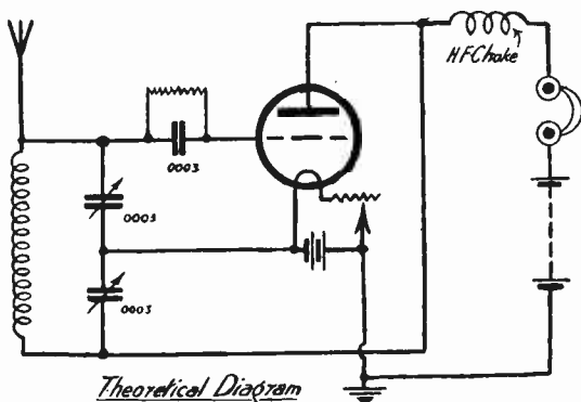
FIG. 5. COLPITTS ONE-VALVE CIRCUIT
