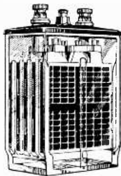
FIG. 9. THE TUNGSTONE ACCUMULATOR
