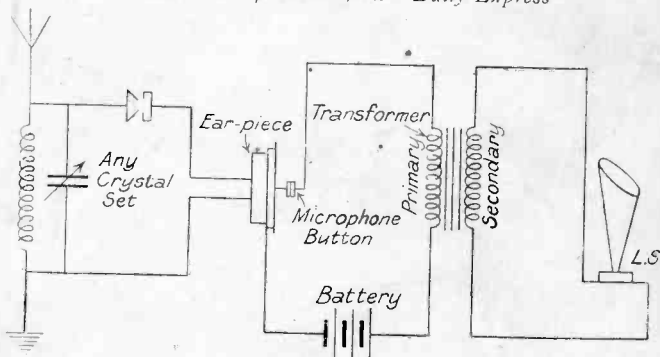
Loud Speaker Crystal Circuit
