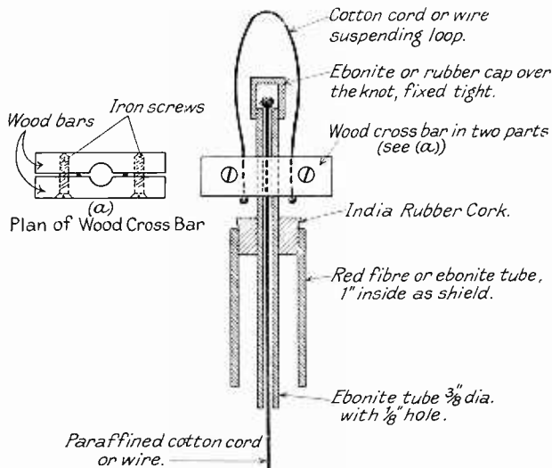
FIG. 1. SECTION OF AN AERIAL INSULATOR. (FLEMING)
