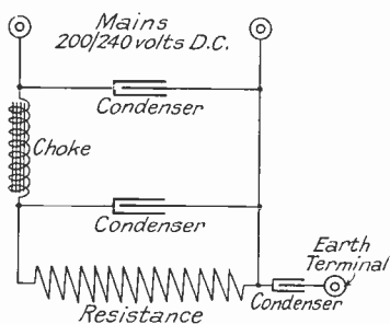
FIG. 4. RADIAC HIGH-TENSION MAINS UNIT DIAGRAM OF CONNECTIONS
