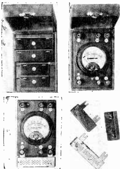
FIG. 24. THE "ONEMETER" Made by Messrs. Leslie Dixon & Co., Ltd.
