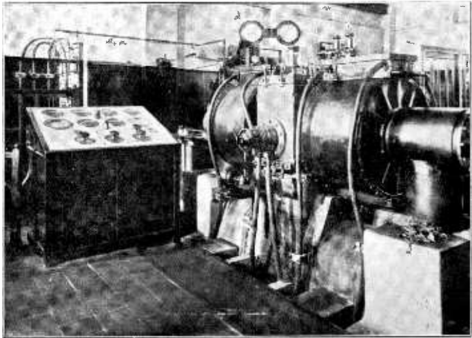
FIG. 4. AN ARC TRANSMITTER AT THE OXFORD STATION
