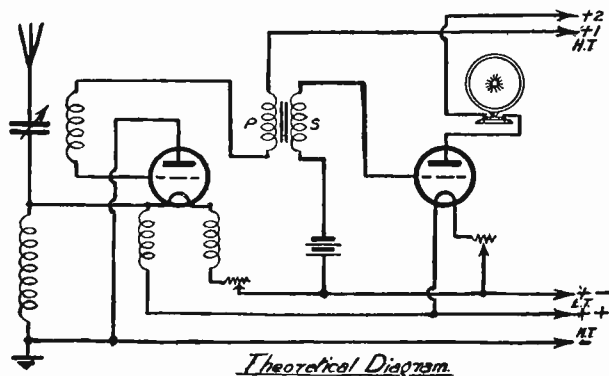
FIG. 3. FILADYNE TWO-VALVE CIRCUIT
