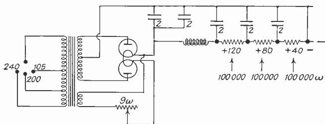
FIG. 3. INTERNAL WIRING OF THE ELVEN MAINS HIGH-TENSION UNIT
