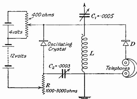
FIG. 7. A PRACTICAL OSCILLATING CRYSTAL CIRCUIT
