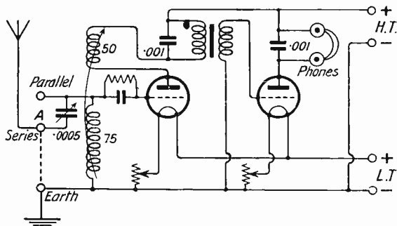
FIG. 1. DETECTOR AND L.F. CIRCUIT FOR 'PHONE D.X. RECEPTION
