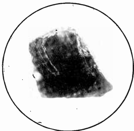
FIG. 1. A ZINCITE CRYSTAL POSSESSING GOOD OSCILLATING PROPERTIES
