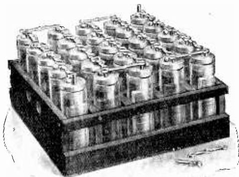
FIG. 10. C.A.V. 60 VOLT, 2 AMP. HIGH-TENSION ACCUMULATOR
