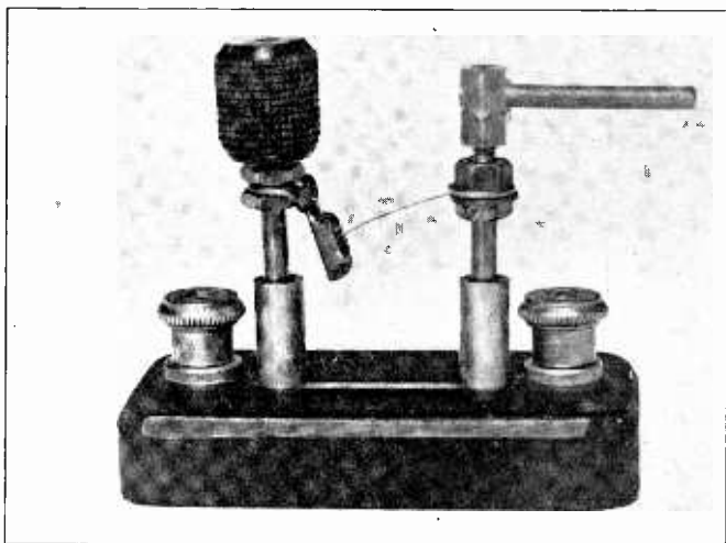
FIG. 2. THE "MILLER" CRYSTAL OSCILLATOR. (PAT. 17767)
