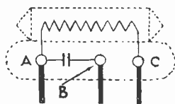
FIG. 29. CONNECTIONS OF THE T.C.C. SERIES—PARALLEL CONDENSER
