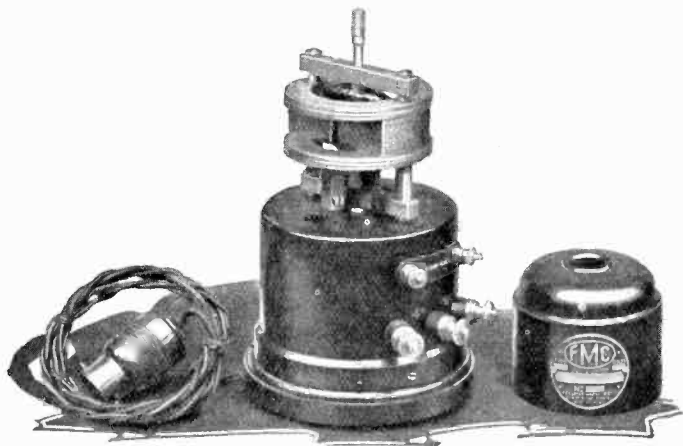
FIG. 6. THE FELLOWS RECTIFIER FOR CHARGING ACCUMULATORS FROM A.C. MAINS
