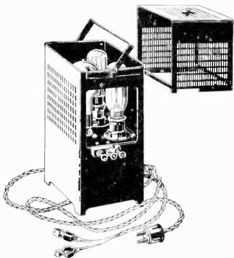
FIG. 7. THE PHILIPS RECTIFIER FOR BATTERY CHARGING
