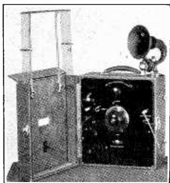
FIG. 38. VIEW OF THE "INCLUSIVE THREE" OPENED READY FOR USE
