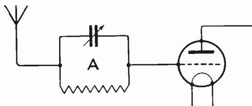
FIG. 4. LODGE "N" CIRCUIT. THEORETICAL DIAGRAM Showing the Oscillator A connected to an aerial and to the grid of a valve, the plate-filament circuit of which may be used in the ordinary way
