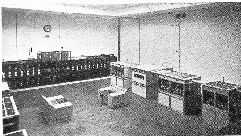
An interesting general view of the transmitter hall at the West Regional Station of the British Broadcasting Corporation, containing two of the high-power transmitters (Type P.B.) constructed by the Marconi Company.
