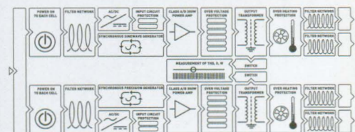
ABOVE & BELOW: Interior photograph and schematic of IsoTek EVO3 Genesis
