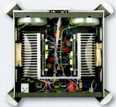
ABOVE & BELOW: Interior photograph and schematic of IsoTek EVO3 Genesis
