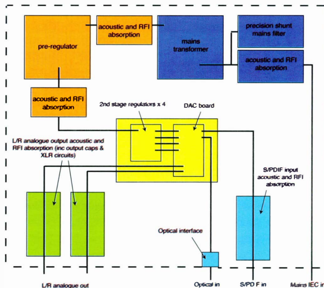
figure 1. Aletheia dac-1 topology
