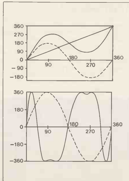
Figure 2a. FM waveform example with modulation frequency = carrier frequency.
