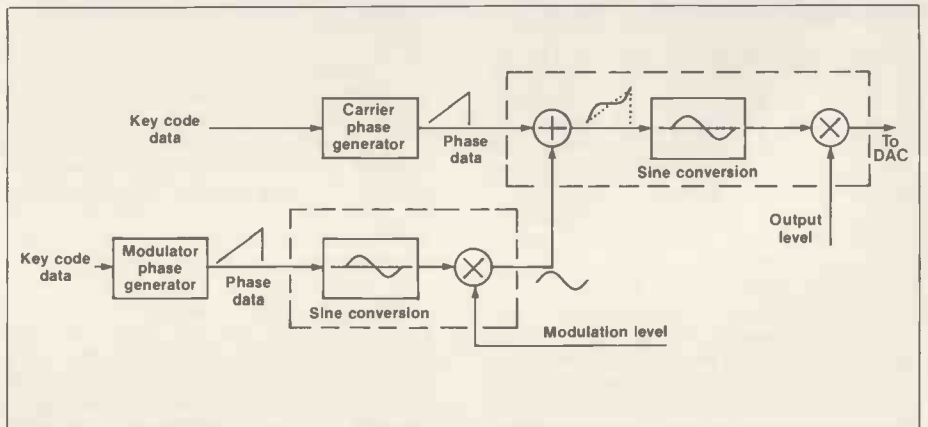
Figure 1. Simplified block diagram of one FM circuit.
