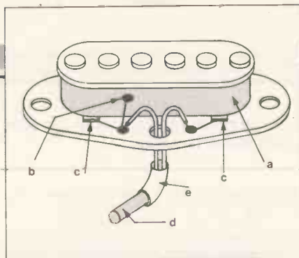
Figure 1. Screening a Stratocaster pickup: a) brass shim wound round the coil; b) earth connection; c) tape over the coil wires to prevent damage by the shim; d) screening braid held in place by heat-shrink sleeving (e).
