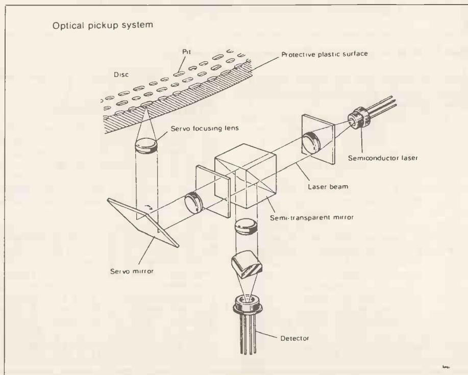
Figure 1. The optical system of the Compact Digital Audio Disc.
