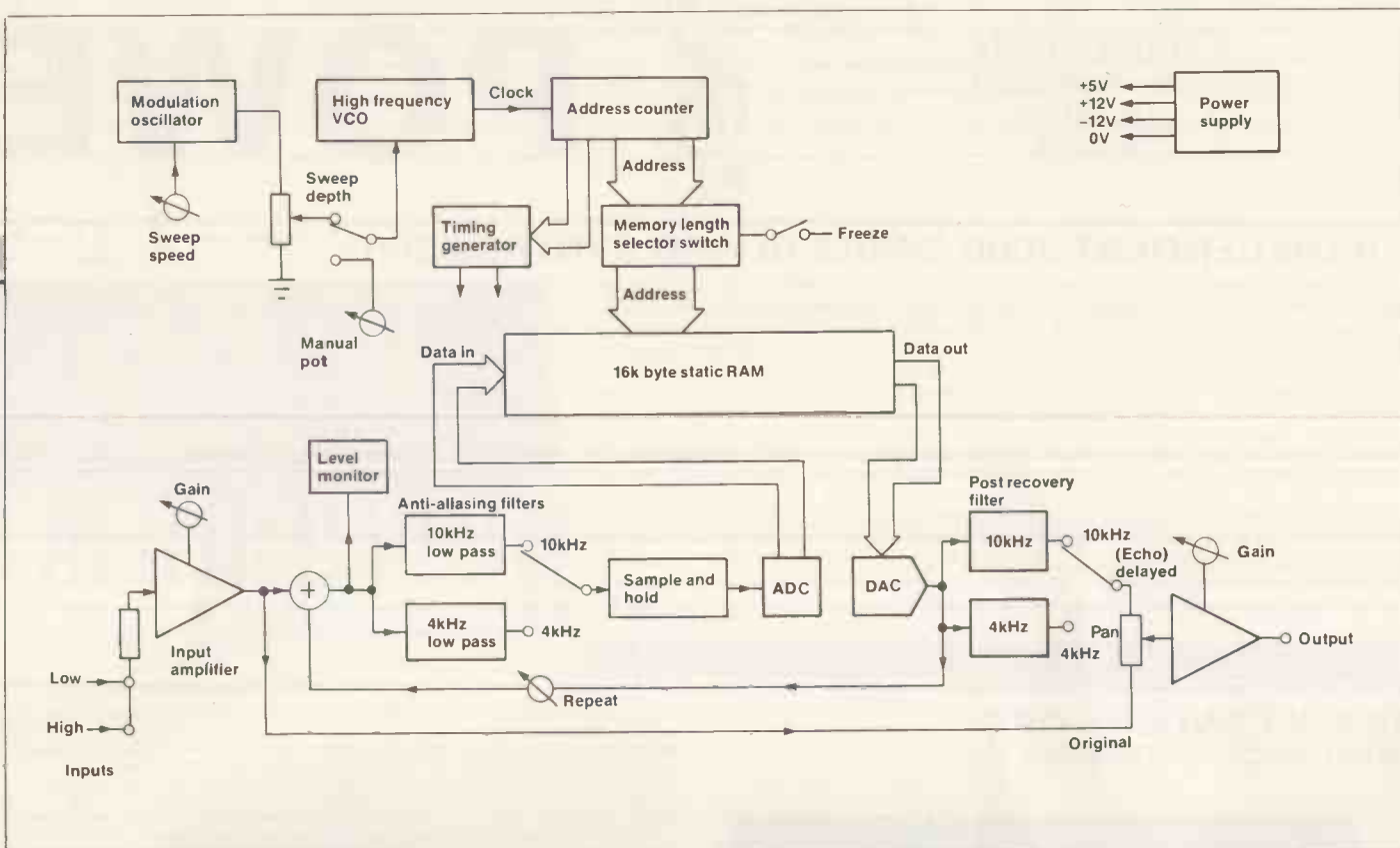
Figure 2. Block diagram of the digital delay line.
