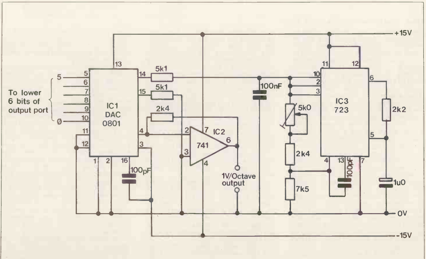
Figure 1. A six bit digital to analogue converter for driving synthesiser control voltage inputs.
