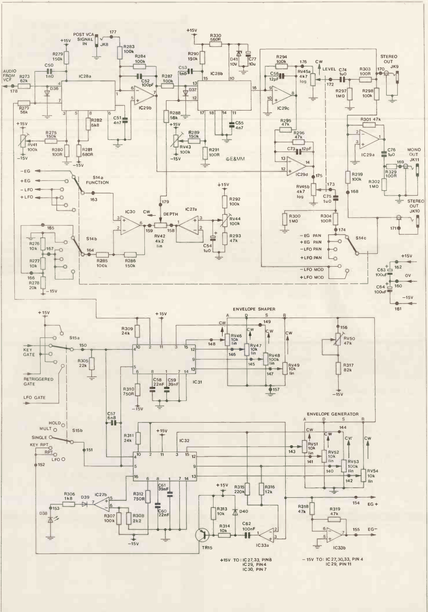
Figure 17. VCAs and envelope generators circuit diagram.
