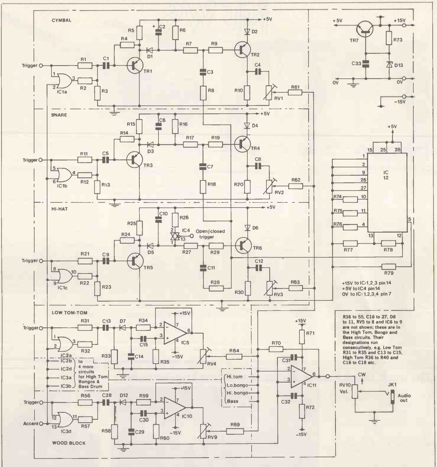
Circuit diagram of the Percussion Sound Generator Board. The circuits for High Tom-Tom, Bongos and Bass Drum are the same as those shown for Block and Low Tom-Tom.
