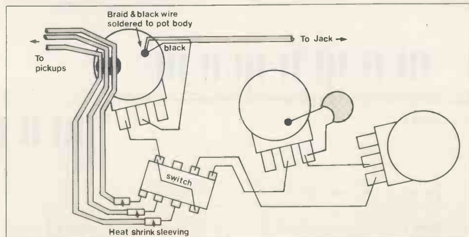
Figure 2. Wiring of the controls. The short wires to the tone controls need not be screened, since they are inside the control cavity.
