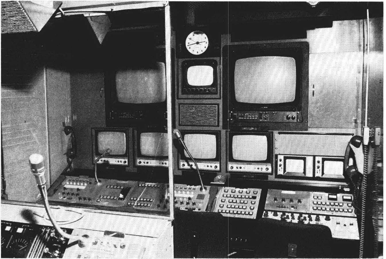
Fig. 4 Monitors and control disk of the two-channel news colour OB unit
