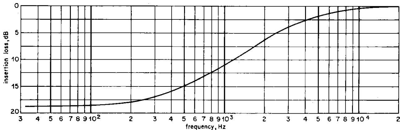
Fig. 2 CCITT pre-emphasis characteristic as used in the simulator
