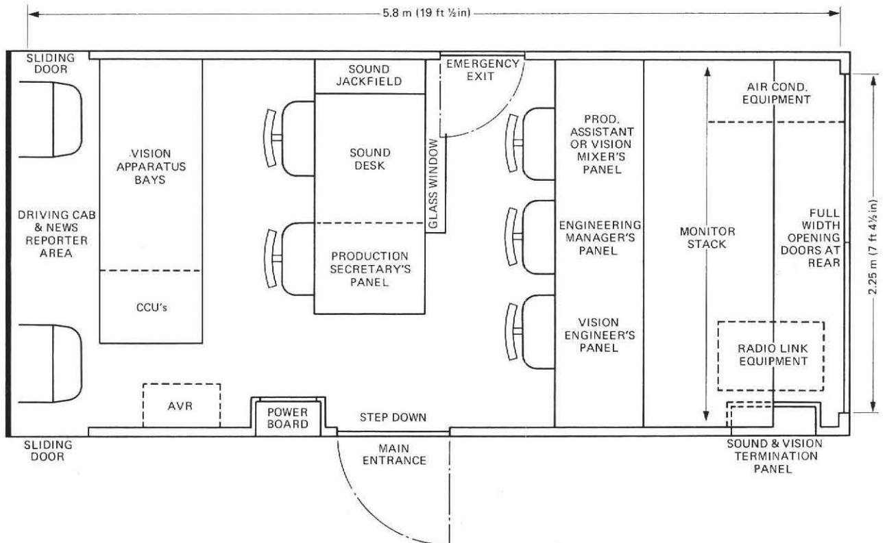
Fig. 5 Layout of the two-channel news colour OB unit
