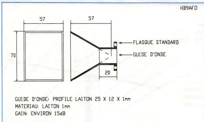
Figure 5 : Antenne cornet.
