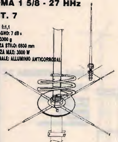
ROMA 1 5/8 - 27 MHz
