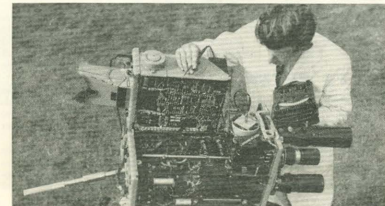
A hint of the complexity of the internal workings of a TV camera is given in this photo of one of the BBC's outdoor units. It contains 41 valves, 190 resistors, 120 condensers, and its own cooling plant. It is built on a unit principle, and whole sections can be removed and quickly replaced in the event of a fault during operation. The heart of all TV cameras is the image orthicon pick-up tube, which converts the received picture into electrical impulses for transmission.
