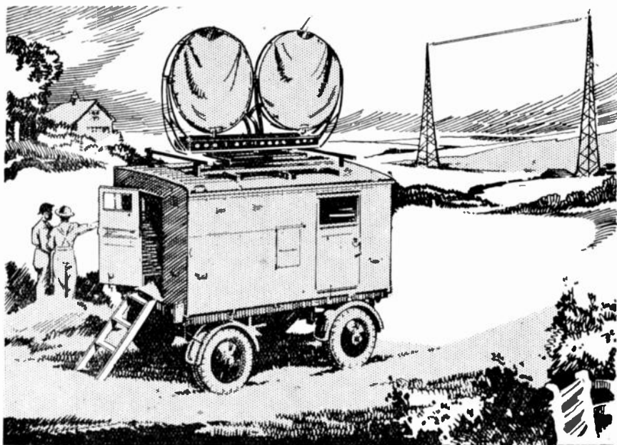
The "No. 10 Set" uses centimetric waves for telephonic communications. Its "bowl-fire" aerials and reflectors are in marked contrast to the long wave aerials.
