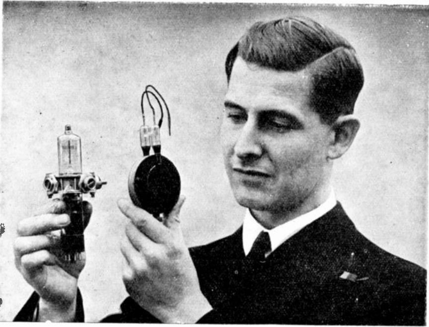
Two valves developed to a high pitch of perfection by British scientists during the war, making centimetre radar possible. Left, the Reflex Klystron and, right, the air-cooled Magnetron.
