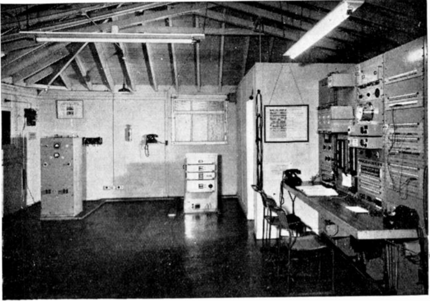
The control room of a typical "Group H" station, showing the transmitter and the control desk.
