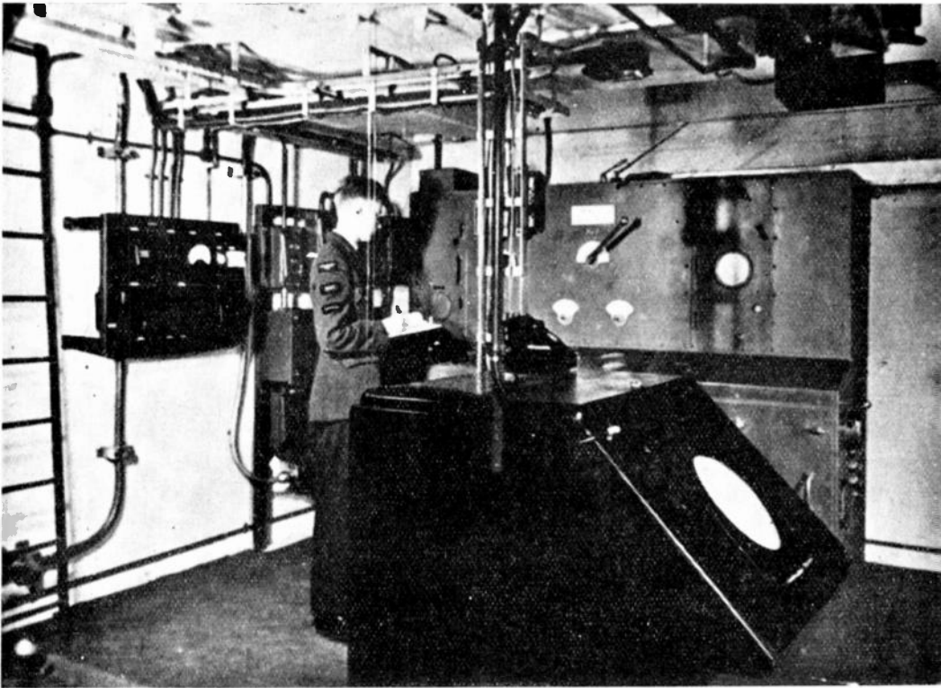
G.C.I. (Ground Controlled Interception) radar stations made it possible for men on the ground to follow, on the cathode-ray tubes, the position of raiders, and to direct our fighters towards them by telephone until the pilots "made contact". This picture shows an underground G.C.I. transmitter and receiver.
