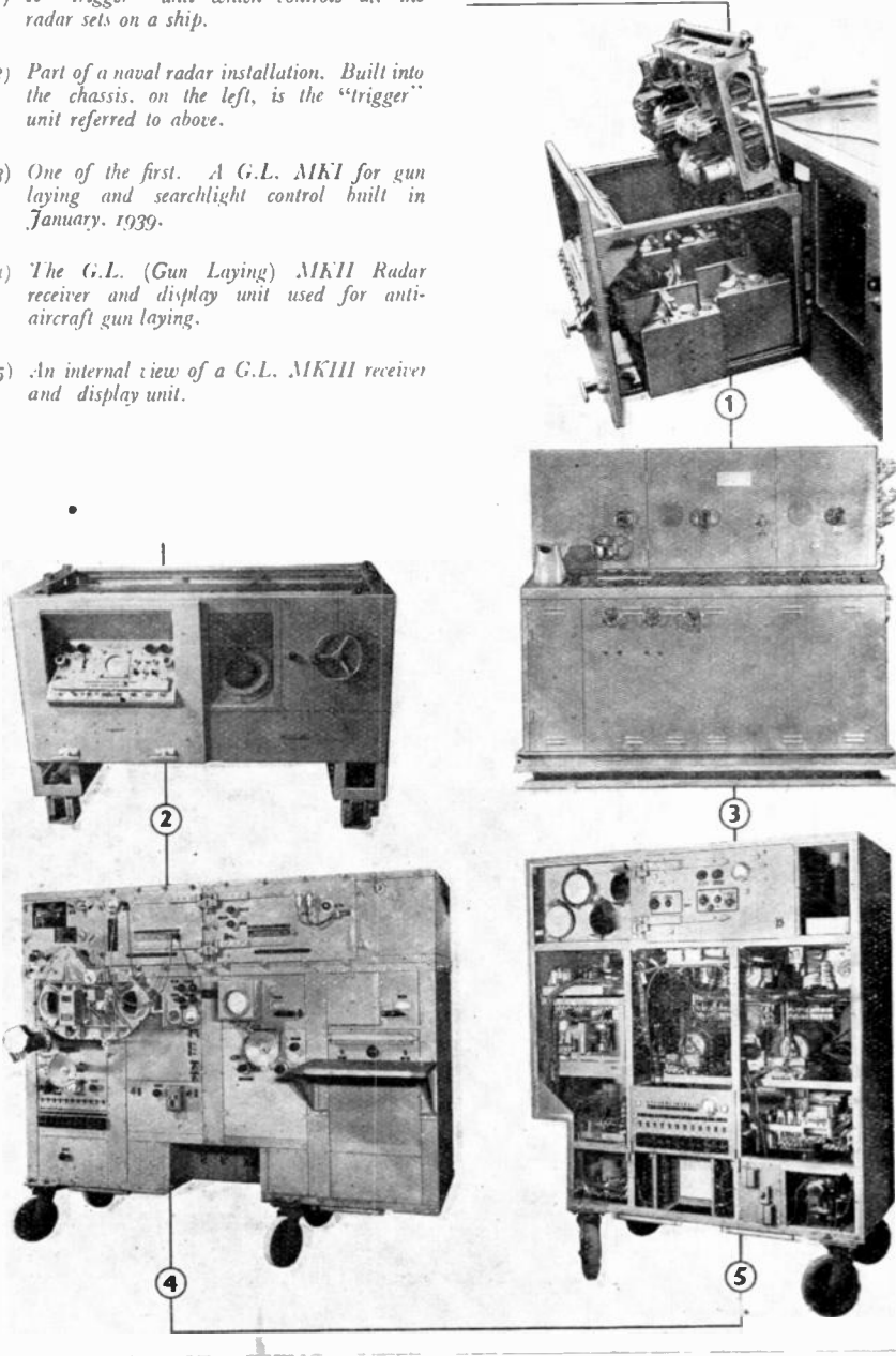
Some of the radar apparatus used in the war was not only highly complex, but weighed several hundredweights. Here are five views of some of the big fellows.
