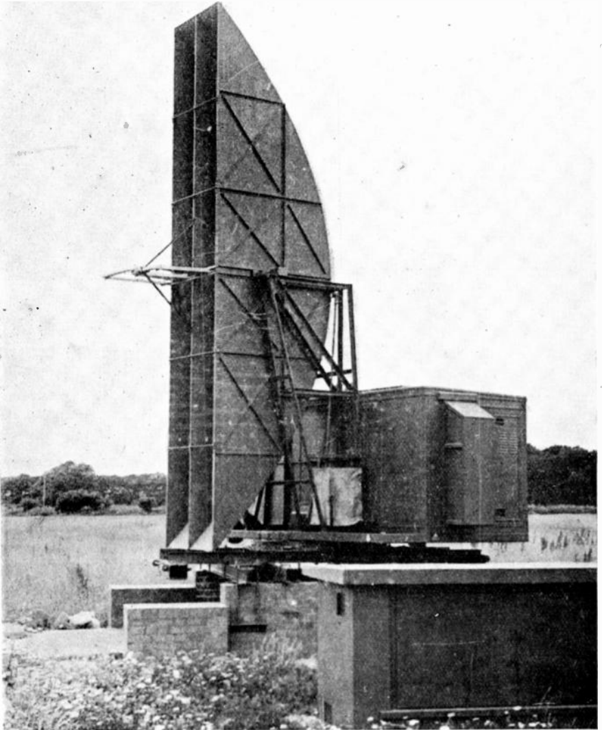
Like a giant slice of cheese, this is the aerial and reflector of the latest British centimetric radar height-finding equipment. It is swivelled by remote control until it points in the direction of an approaching aircraft, and tilted up and down until returning radar echoes indicate the target.
