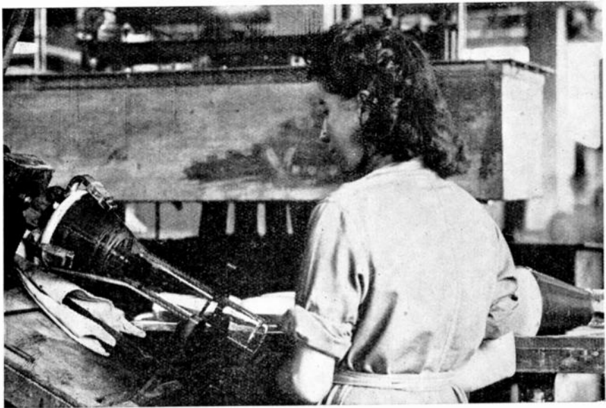
Cathode-ray tube—heart of the radar set. Scores of thousands were made in Britain for equipment of every type. This girl worker is applying a special coating to the inside of a tube.
