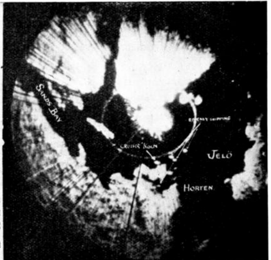
The work of H2S—radar's magic eye—described in this chapter. The map on the left is part of a chart showing Oslo Fiord, with Sands Bay just cutting the circle in the North-East corner. The picture on the right is what the navigator saw on the screen of his cathode-ray tube at night. Enemy shipping, including a large blob caused by the cruiser "Koln," is clearly visible to the observer.
