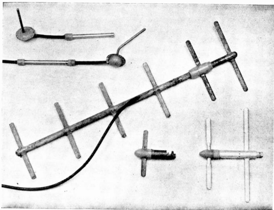
Most secret. Each of these little radar aerials could have told a useful story to the enemy if he had been able to obtain advance details of them.
