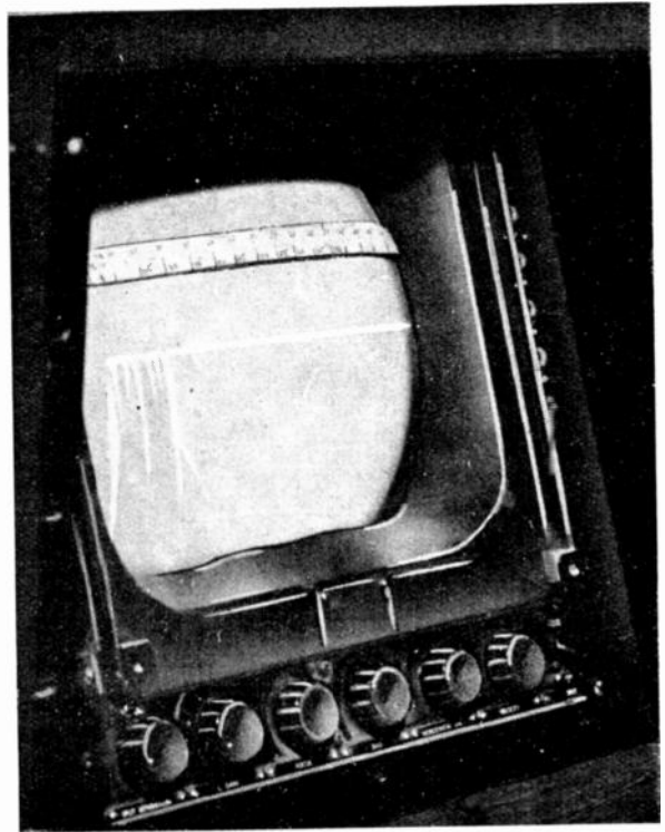
Far more advanced than the apparatus used by Sir Edward Appleton, this piece of R.A.F. radar equipment none the less employs virtually the same principle. It is an "electric tape measure". The line of light on the cathode-ray tube shows "kicks" when an echo is received. The spacing of the "kicks" is measured off in miles on the scale.
