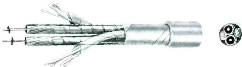
Photograph showing interior construction of coaxial cable used in television line transmission. Cross-section on right shows arrangement of essential parts. (Courtesy Bell Telephone Laboratories.)
