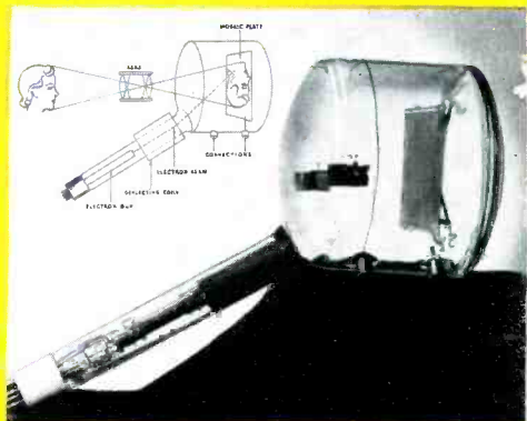
Iconoscope, the "electric eye" of the television camera. Diagram shows how lens focuses image on mosaic plate.
