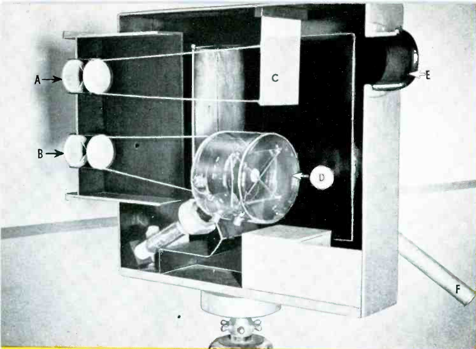
Simplified cutaway model of television studio camera, indicating principal parts. A—Focusing lens for ground-glass. B—Lens which focuses image on Iconoscope plate. C—Ground glass. D—Iconoscope. E—Viewing aperture which permits operator to see the ground-glass image. F—Focusing handle.
