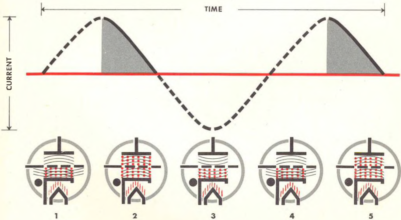
THE GRID ACTION OF A GAS-FILLED TUBE— 1. Grid prevents flow of electrons—completely cancels effect of anode. 2. When less than a minimum voltage is applied to grid, full flow of electrons is suddenly released. 3. Anode is negative and does not attract electrons. 4-5. Cycle repeats.
