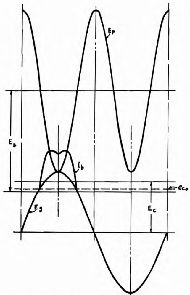
Figure 1. Current-Voltage Oscillagrams for Doubler.
