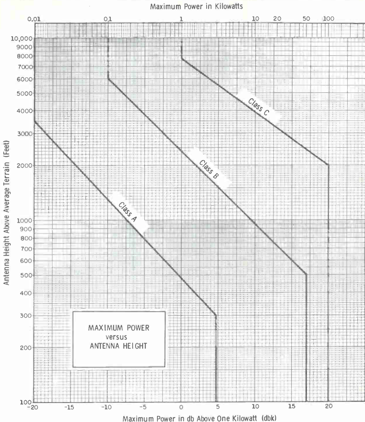
Fig. 3-9. FM antenna height vs power chart.
