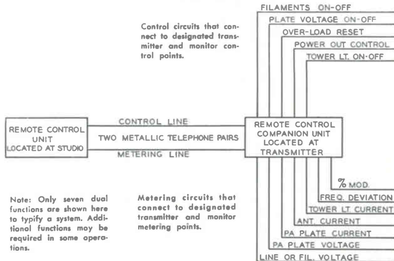
Fig. 9-1. Block diagram of a typical remote control system. Two telephone lines are used between the studio and transmitter, one for control, the other for monitoring.
