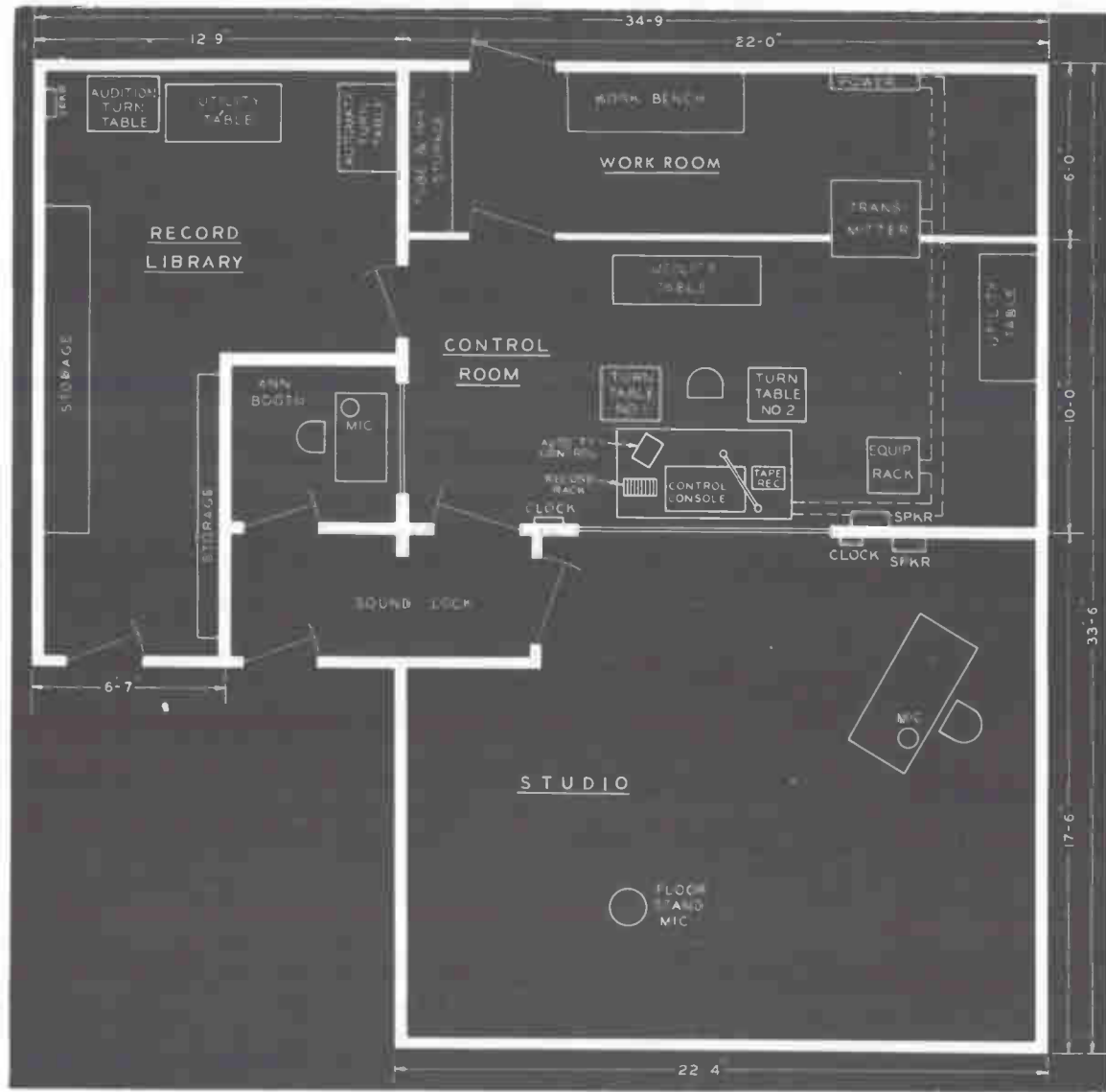
Fig. 4-7. Basic layout for a "Plan 2" facility.
