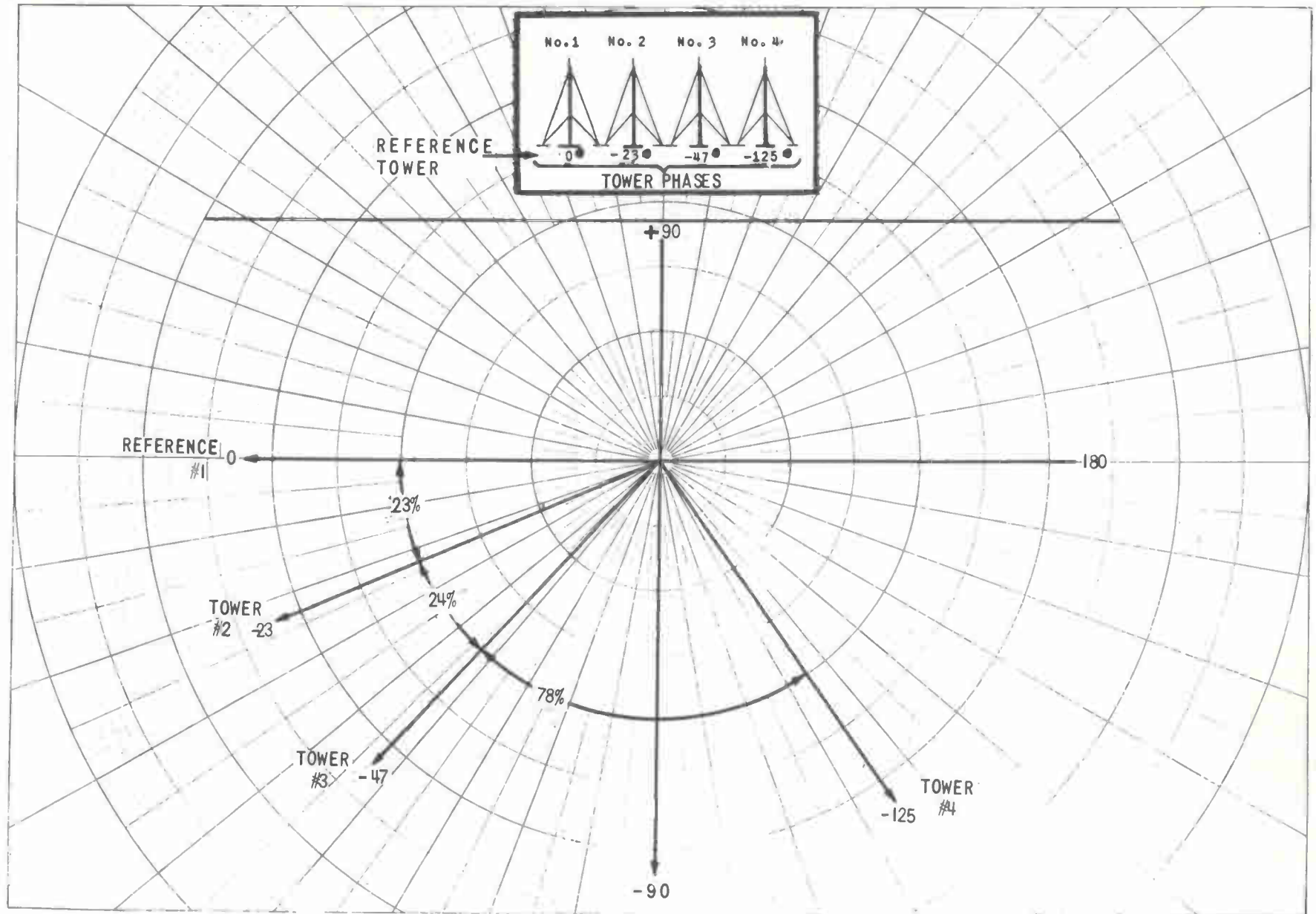
Fig. 7-18. Typical phase-angle vector diagram of a four-tower in-line directional antenna array.
