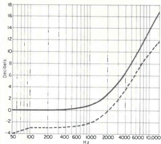
Fig. 15-12. Standard pre-emphasis curves.
