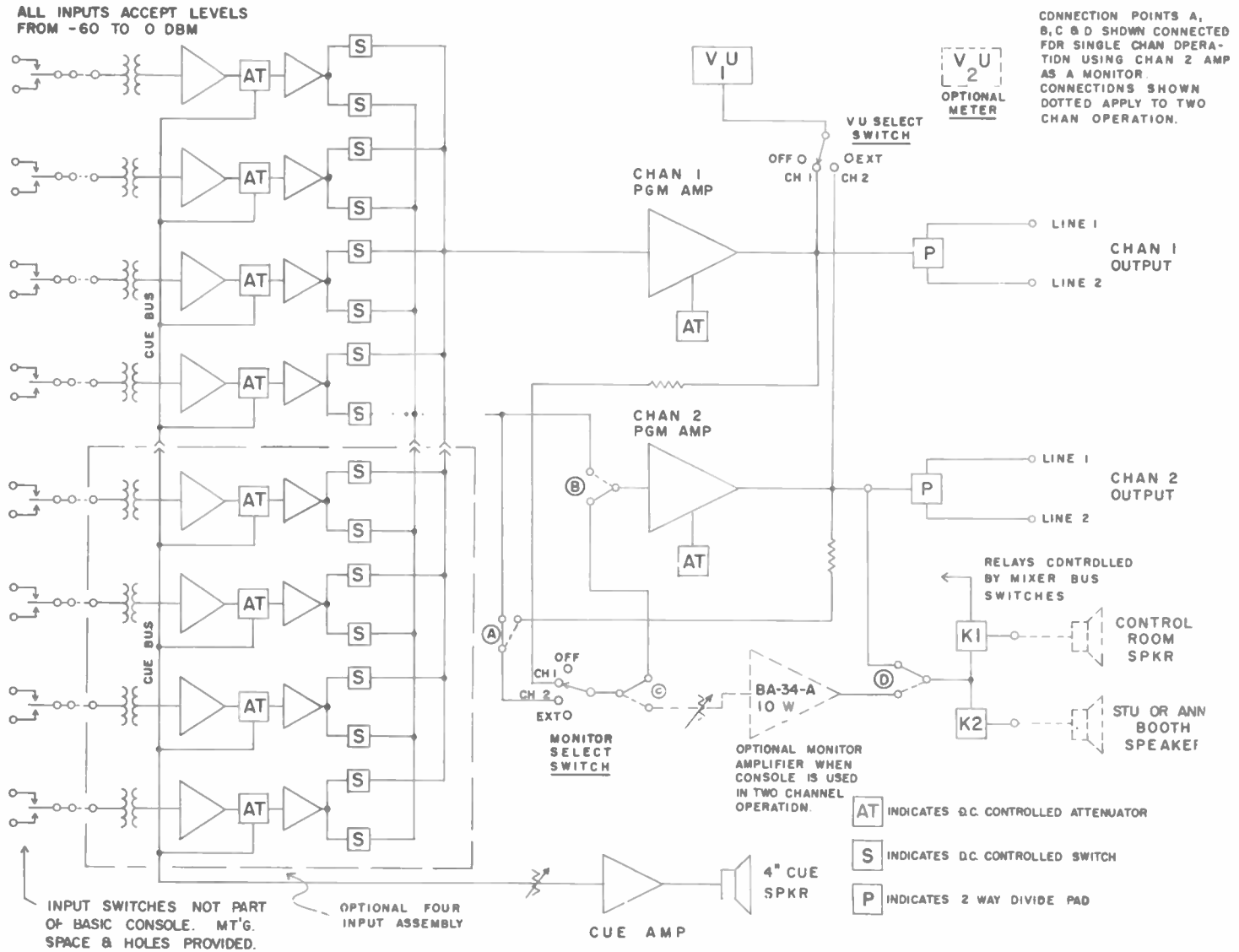
Fig. 6-4. Block diagram of a broadcast station layout using solid-state equipment.
