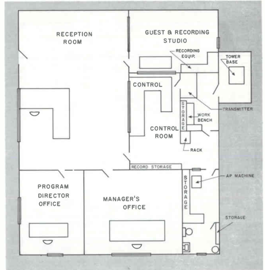
Fig. 16-18. Floor plan for WPHC's plant.
