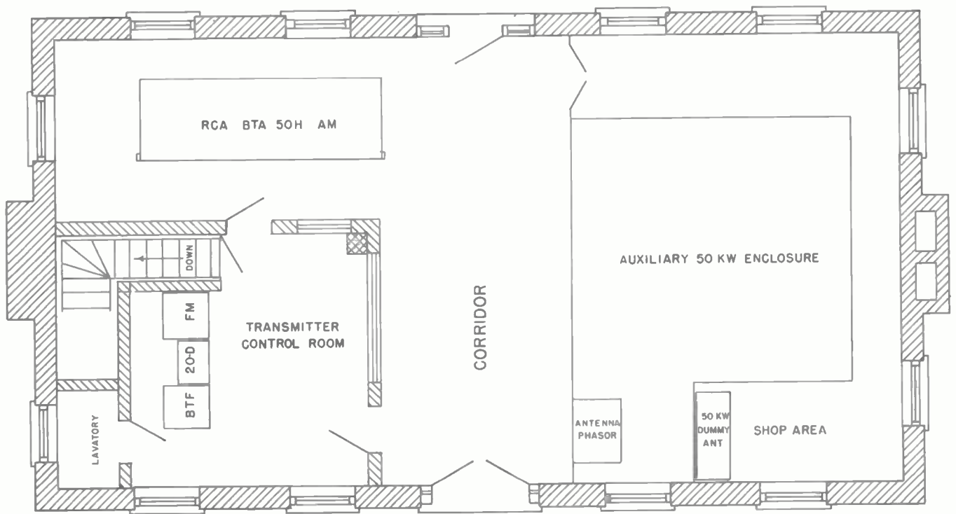
Fig. 16-20. WRVA radio transmitter building floor plan.
