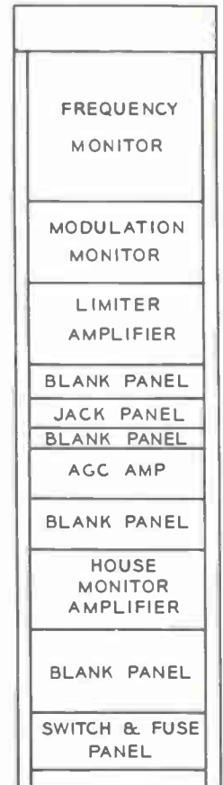
Fig. 4-8. This "Plan 2" rack layout includes a house monitoring amplifier.
