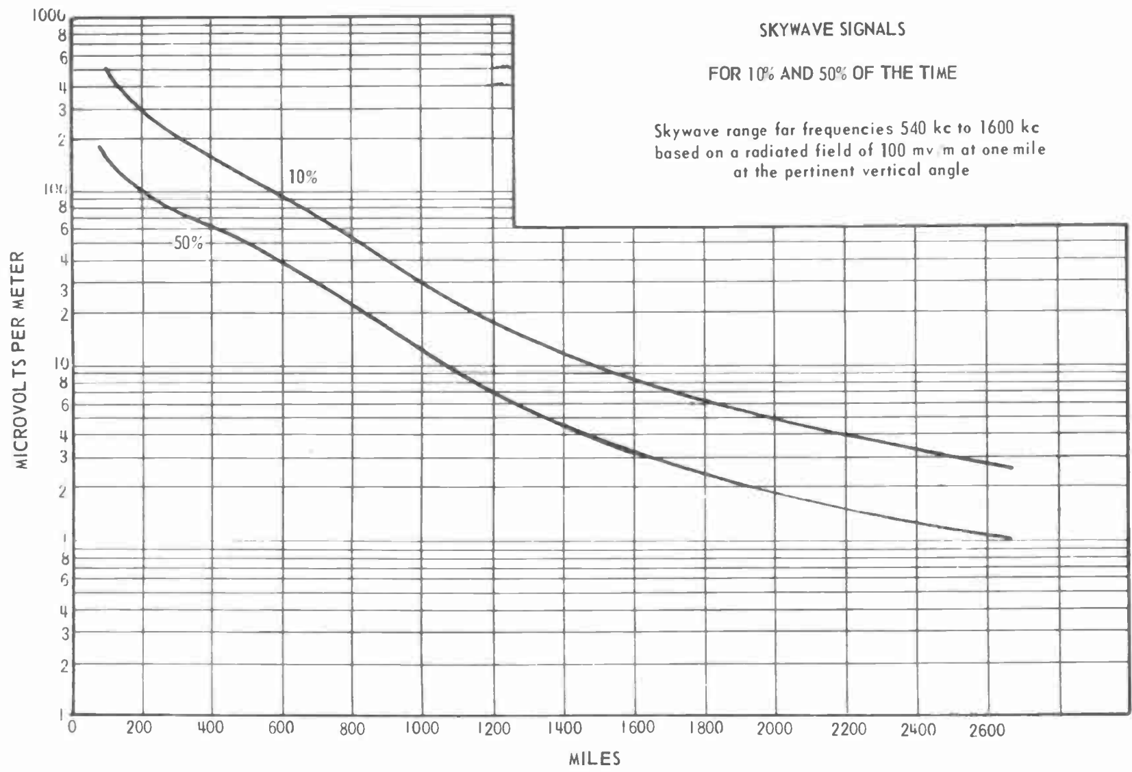
Fig. 2-5. Skywave signals for 10% and 50% of the time.
