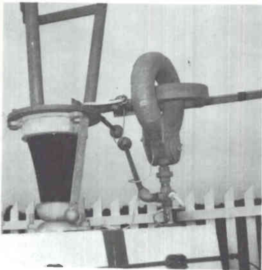
Fig. 7-6. Typical installation of a lighting transformer to isolate the AC circuit from RF.
