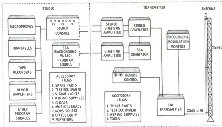
Fig. 6-7. Block diagram of a typical stereo equipment layout.
