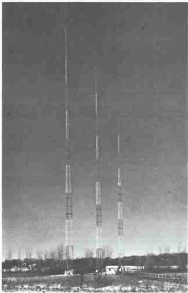
Fig. 7-10. A typical three-tower directional antenna array using self-supporting towers.
