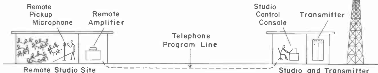
Fig. 1-5. Another variation in separate studio and transmitter facilities: Pickup and control equipment installed in public meeting places provides additional program sources.
