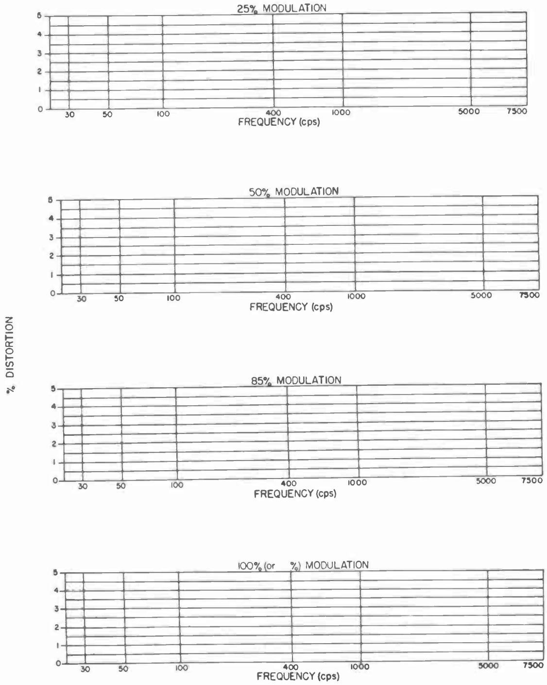
Fig. 15-5. Form AFP-3: Audio frequency harmonic content data and curves.
