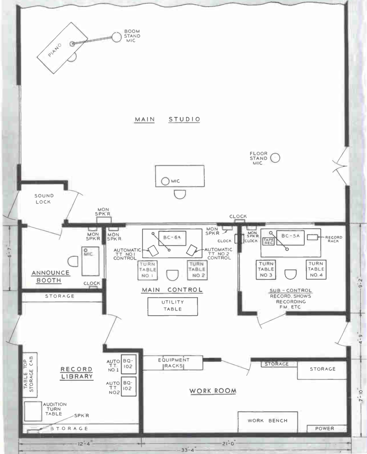
Fig. 4-13. Floor plan suitable for a larger operation.
