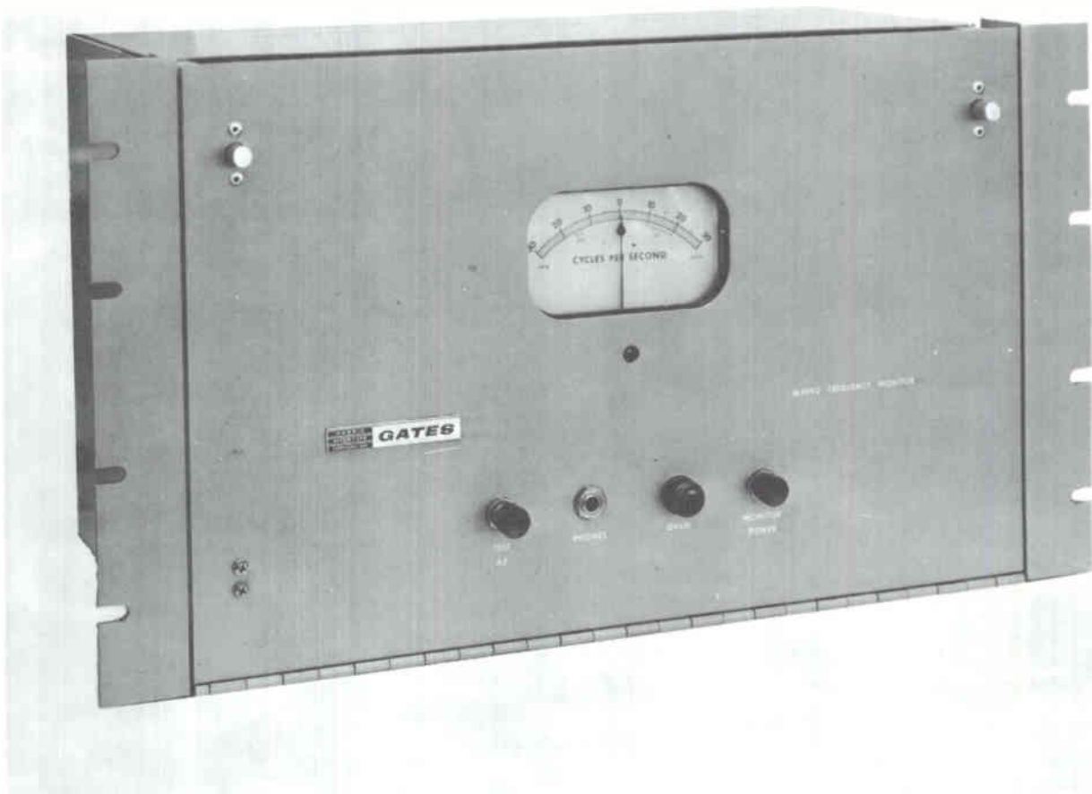
Fig. 10-18. AM frequency monitor.
