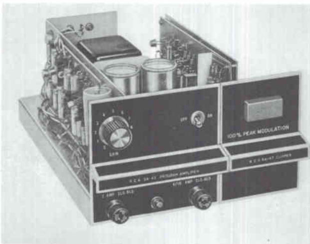
Fig. 10-14. A peak clipper amplifier.
