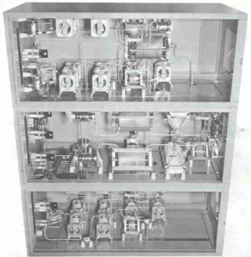
Fig. 7-11. Phasing equipment such as this is required for a directional antenna system.
