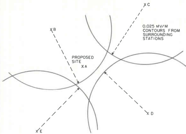
Fig. 2-1. Plot for proposed Station A. Stations B, C, D, and E are co-channel, same-frequency stations.
