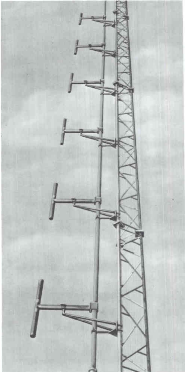
Fig. 8-4. Radiating element of a typical vertically-polarized FM antenna.
