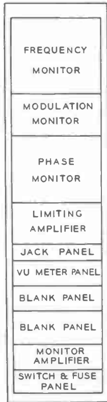
Fig. 5-4. Layout of a typical transmitter monitoring equipment rack.
