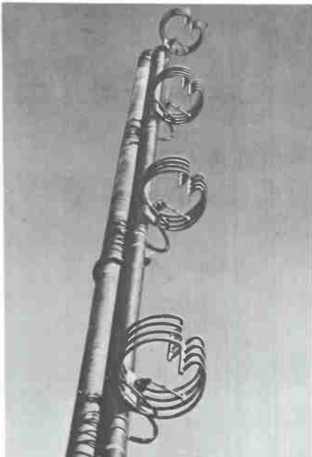
Fig. 8-11. A four-bay horizontally-polarized FM antenna array.
