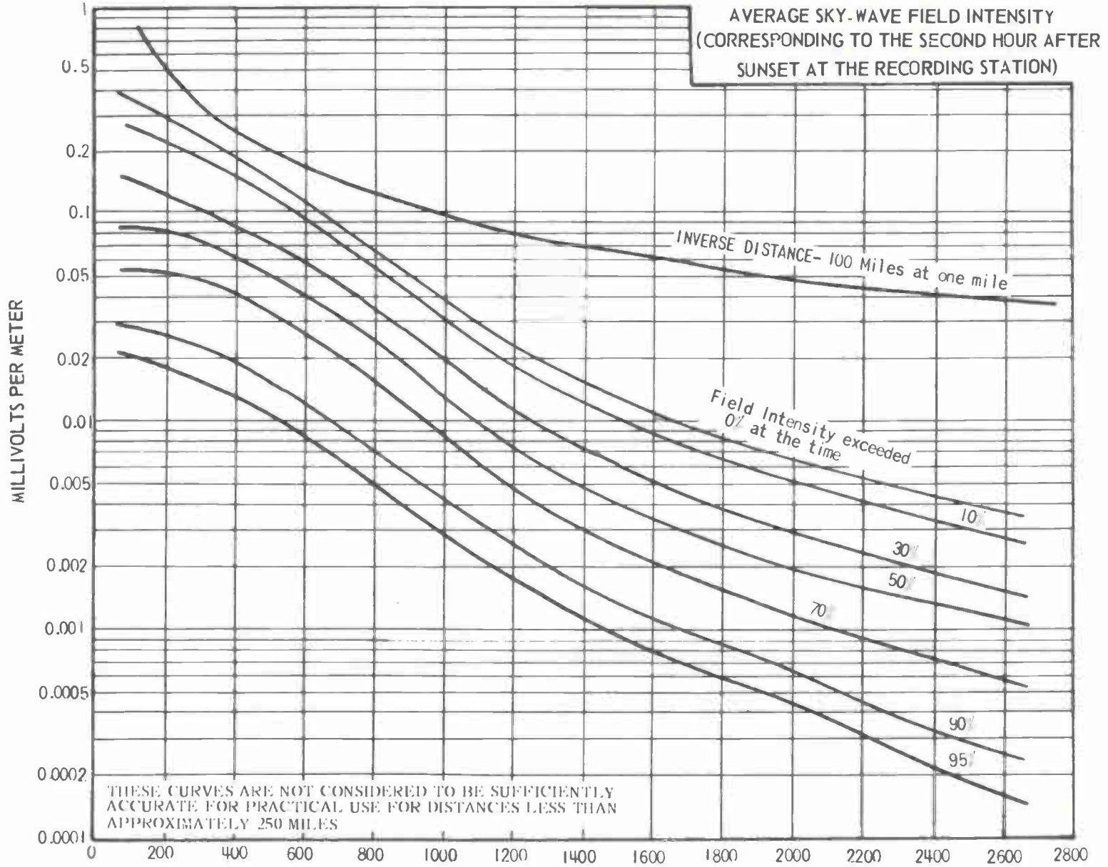
Fig. 2-4. Average skywave field intensity chart.
