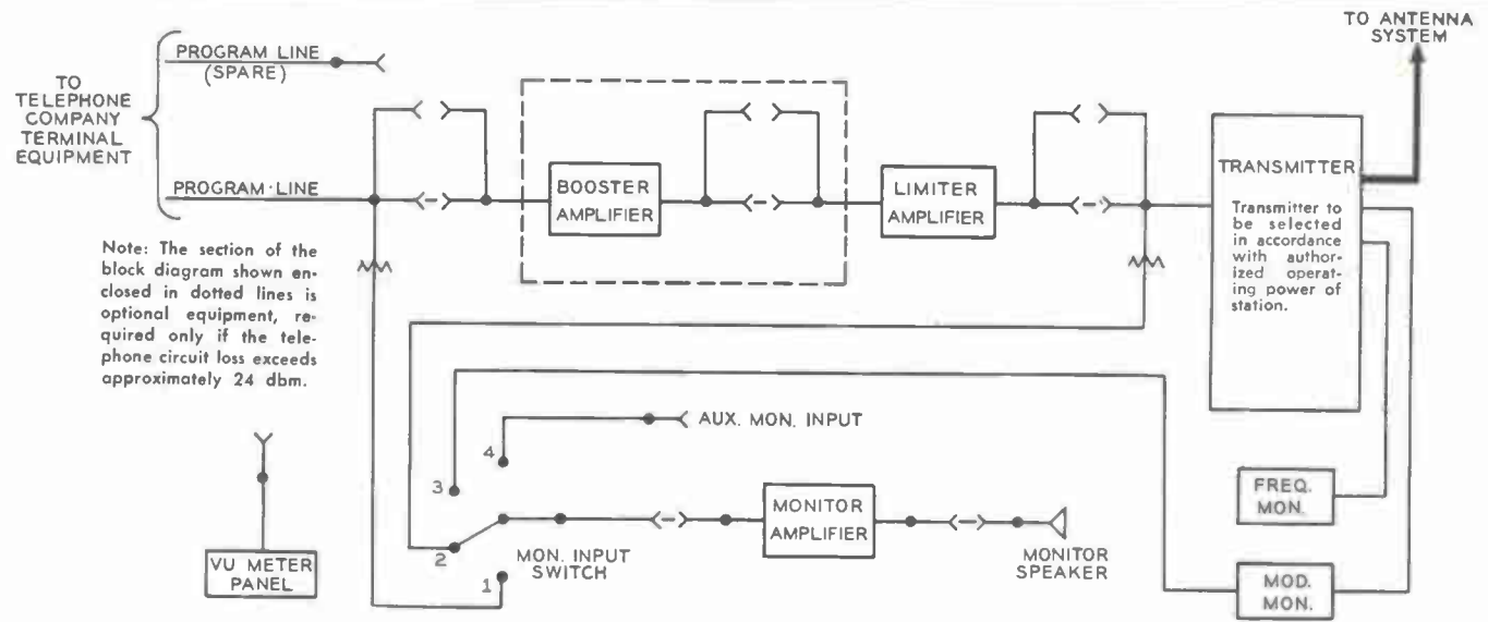
Fig. 5-5. Block diagram showing monitoring equipment interconnections (see Fig. 5-4).
