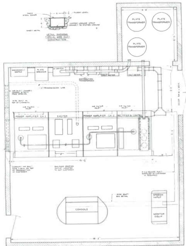
Fig. 5-7. A typical 50-KW AM transmitter floor plan installation, wiring basic wiring details.
