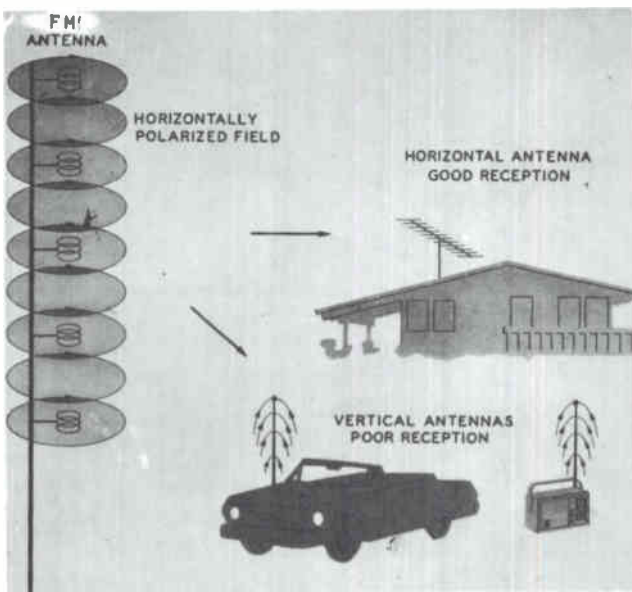
Fig. 8-1. Horizontally-polarized transmission provides good reception for homes but tends to serve autos and portables poorly.
