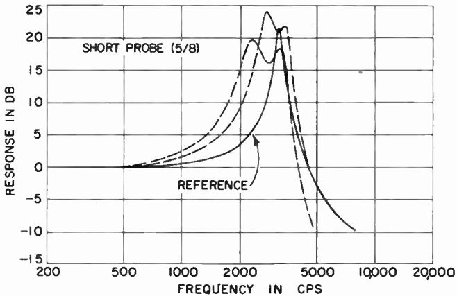
Figure 13-2. Frequency response of vibration pickup mounted on hand-held short (5/8-inch) probe. Several sample responses are shown.
