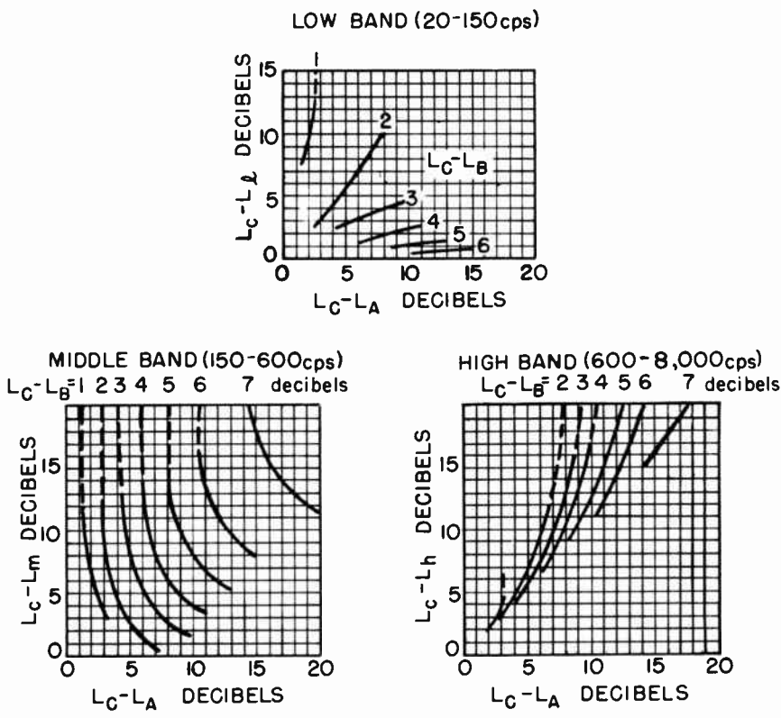
Figure 6-3. Curves for calculating an approximate frequency analysis in three bands from level readings taken using the three weighting networks. Enter the abscissa of each graph with the measured value L_C - L_A . Then proceed vertically to the curve labeled with the measured value of L_C - L_B , then horizontally to the ordinate value for each of the three bands corresponding to the difference between the individual band levels and the over-all level. (This method of analysis was developed by J. R. Cox, Jr.)
