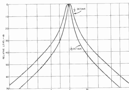
Band-pass characteristics of the analyzer.
