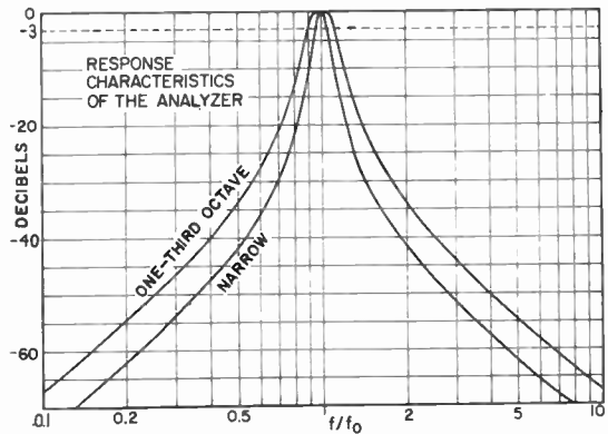
Figure 11-7. Selectivity characteristics of the Type 1564-A Sound and Vibration Analyzer.
