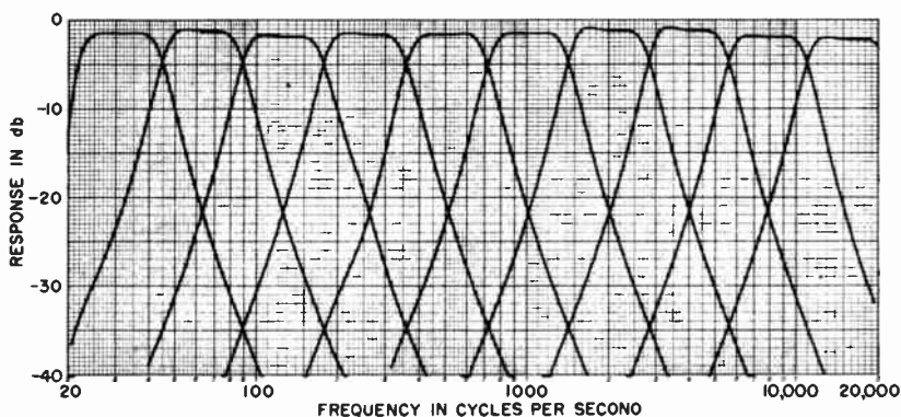
Figure 6-4. Typical response characteristics, Type 1558-AP Octave-Band Noise Analyzer.
