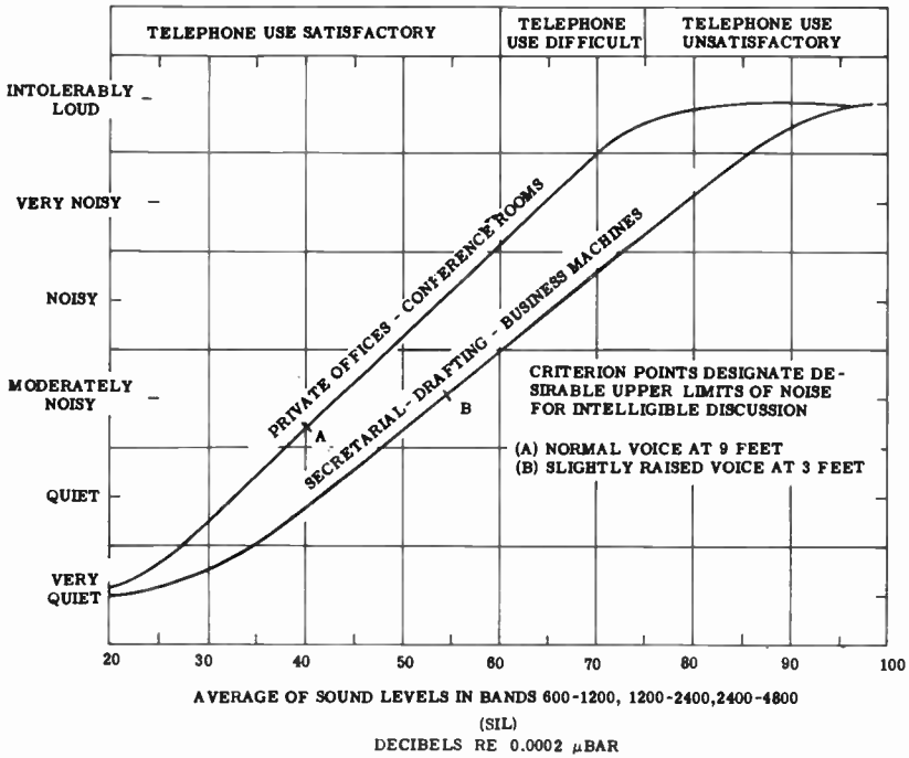
Figure 8-3. Rating chart for office noises. Data were determined by an octave-band analysis and correlated with subjective tests. (Courtesy Beranek and Newman.)
