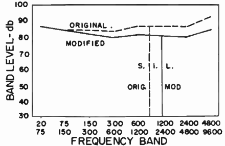
Figures 9-1 through 9-4. Examples to illustrate the possible noise reduction effects of some noise control measures.
