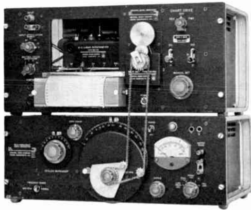
Figure 4-11. The Type 1521-A Graphic Level Recorder and the Type 1304-B Beat-Frequency Oscillator comprise a convenient system for plotting frequency response.
