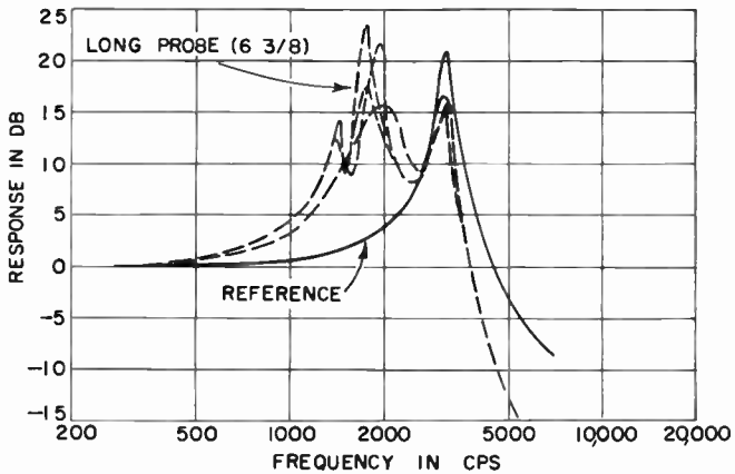
Figure 13-1. Frequency response of vibration pickup mounted on hand-held long (6 3/8-inch) probe. Several sample responses are shown.
