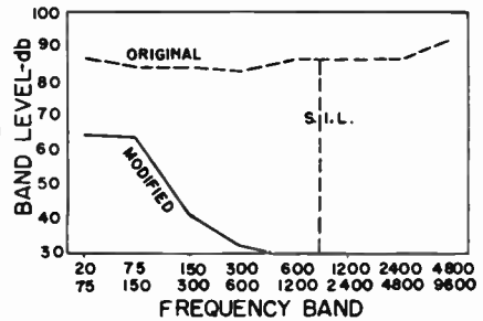
Figures 9-5 through 9-8. Examples to illustrate the noise reduction possible by the use of enclosures.
