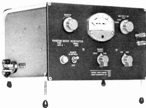
Figure 4-12. The Type 1390-B Random-Noise Generator.
