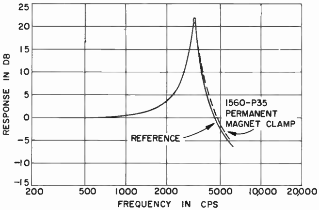
Figure 13-5. Frequency response of vibration pickup attached by Type 1560-P35 Permanent-Magnet Clamp.
