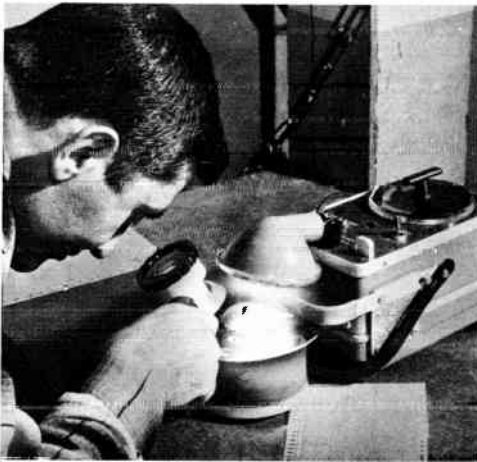
Figure 12-4. Acoustic Research, Inc. studies acoustic-radiator diaphragms with the Type 1531-A Strobotac® electronic stroboscope. A band of fine flock fiber is applied to the radiator's surface. Under stroboscopic light, nodal points and radiator break-up zones are pinpointed by the degree of fiber vibration along the band of flock. Former methods limited measurements to 1 kc. The high intensity, short-duration flash of this new stroboscope extends these measurements to 20 kc.
