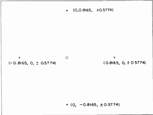
Figure 7-3. Plan view of eight points uniformly distributed on a sphere of unit radius. Coordinates are given in terms of distances from center along three mutually perpendicular axes ( x, y, z ). The "±" refers to the existence of two points, one above the x - y reference plane and one below. When measurements are to be made on a hemisphere, only the four points above the plane are used.
