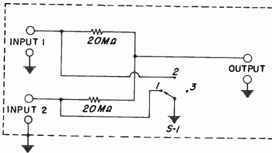
Figure 13-7. A convenient arrangement of the summing circuits of Figure 13-6.
