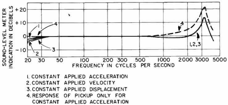
Figure 11-6. Over-all frequency response of Type 1560-P11B Vibration Pickup System and sound-level meter for constant applied acceleration, displacement, and velocity.
