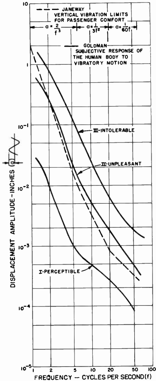
Figure 14-1. Subjective response of the human body to vibratory motion as a function of frequency.
