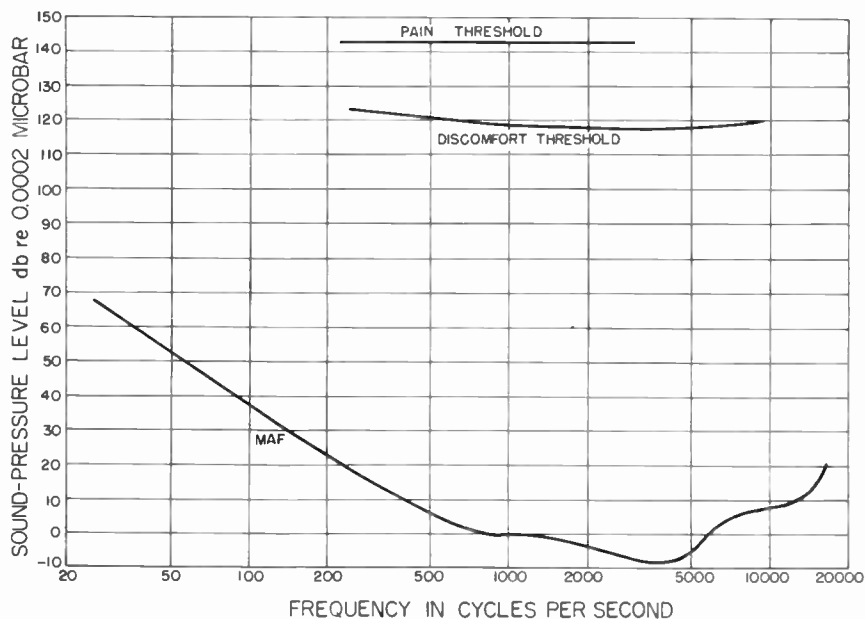
Figure 3-1. Thresholds of hearing and tolerance.
