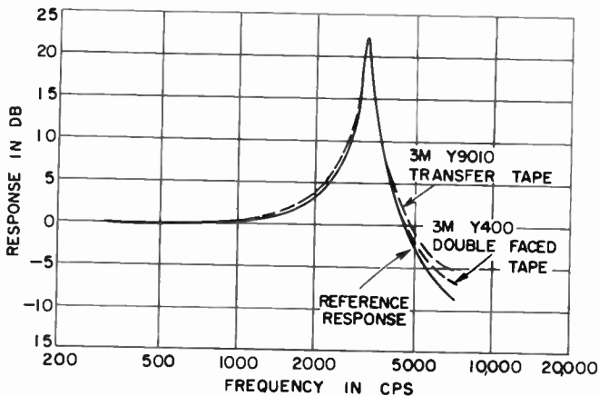
Figure 13-3. Frequency response of vibration pickup attached by means of Minnesota Mining Types Y9010 and Y400 tapes.
