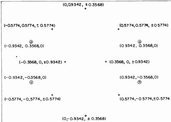
Figure 7-5. Plan view of 20 points uniformly distributed on a sphere of unit radius. Coordinates are given as in Figure 7-3. When measurements are to be made on a hemisphere, 12 points are used, eight above the reference plane and four in the plane ( Z = 0 , shown encircled). The four in the plane are weighted by a factor of 1/2 in power (see text).
