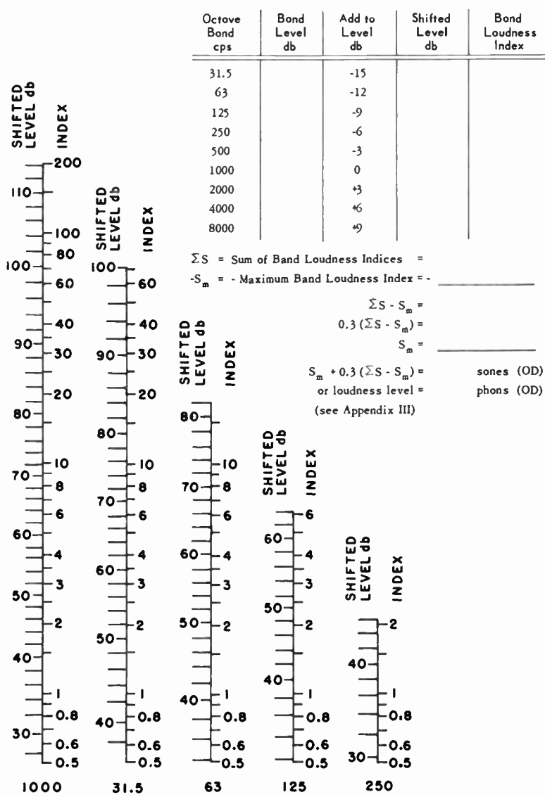
Figure 8-2. Chart for calculating loudness from an analysis of the noise in octave bands centered at 31.5, 63, 125, 250, 500, 1000, 2000, 4000, and 8000 cps. For each of the four lower octave bands, enter the shifted level in the appropriate line chart to obtain the loudness index. For levels outside the range of these charts, and for all other octave bands, use the left-hand line chart to obtain loudness indexes. The noise is assumed to be coming at the listener from many directions (diffuse field).
