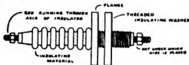
FIG. 26.—Leading-in insulator.
