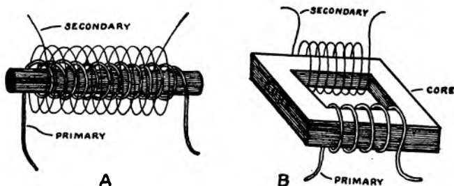
FIG. 39.—Open and closed core transformers.
