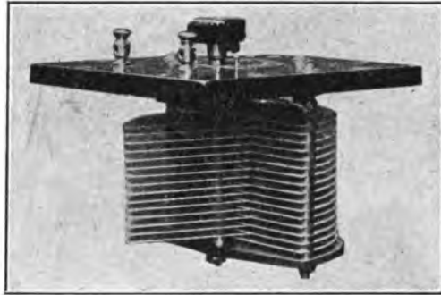
FIG. 82.—Interior of rotary variable condenser showing construction.
