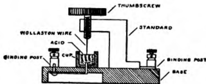
FIG. 72.—Electrolytic detector.
