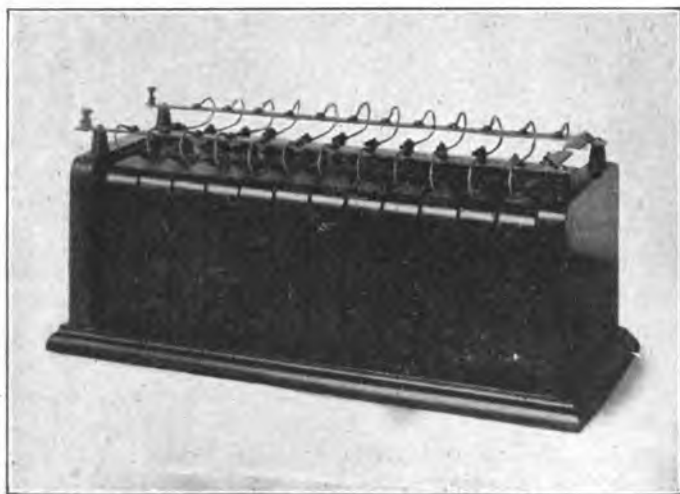
FIG. 95.—Transmitting condenser (molded dielectric).
