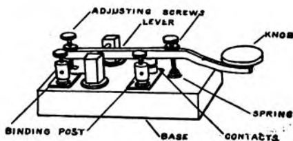
FIG. 57.—Wireless key.
