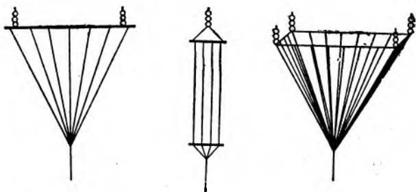
FIG. 15.—Vertical aerials of the “grid,” “fan” and “inverted pyramid” types.
