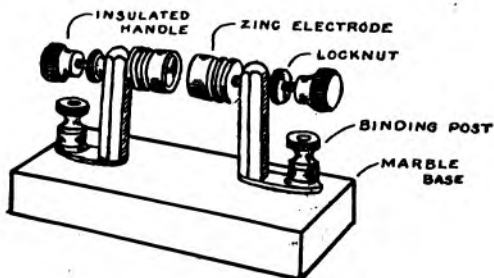
FIG. 50.—Spark gap.
