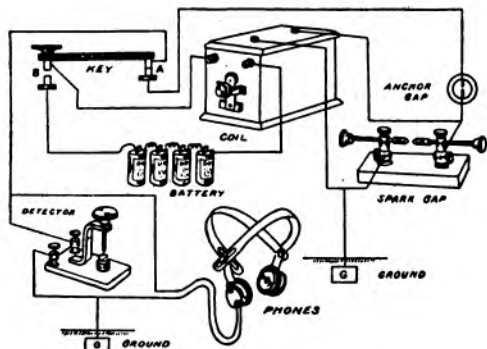
FIG. 118.—Breaking-in system.
