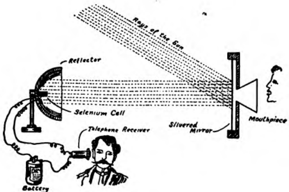
FIG. 133.—The photophone.
