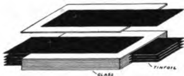
FIG. 46.—Diagram showing construction of condenser.
