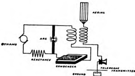
FIG. 146.—Diagram showing how a wireless telephone transmitting system is arranged.
