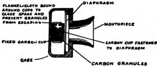
FIG. 131.—Diagram of a telephone transmitter.
