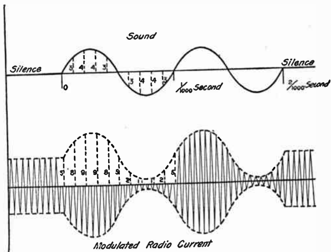
FIG. 49: How the Antenna Current Varies in Radio-Telephony. — The 1,000-cycle pure tone current, indicated along the upper line, will add its values to, and subtract them from, the average strength of the 20,000-cycle radio current shown below. When the radio current remains of constant intensity, no sounds are transmitted.
