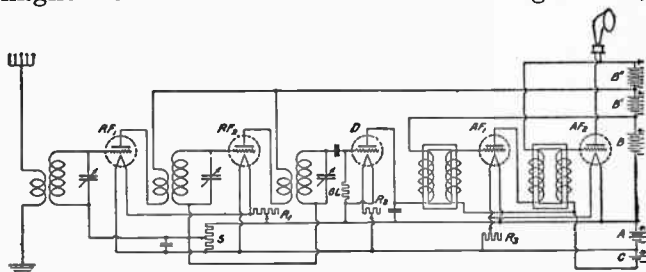
FIG. 62: A Complete Five-Tube Receiver of the Tuned Radio-Frequency Type. — There are several points of interest in this arrangement. Since the resistor GL fixes the potential of the detector grid by direct connection to the positive-filament terminal, the lower plates of the three tuning condensers may be wired directly to the moving contact of the potentiometer S . The three condensers may therefore be replaced by a triple-unit multiple condenser having its common shaft so connected, for single-control tuning. The B battery is divided into three parts so that the most favorable plate potentials may be chosen. Only three rheostats are used, R_1 controlling both radio-frequency tubes RF_1 and RF_2 , R_2 providing adjustment for the detector, and R_3 being associated with both audio amplifiers AF_1 and AF_2 .
