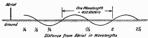
FIG. 34: Curve of Field Strength. — This shows the observations of Fig. 33 in curve form and continued for a distance of 2\frac{1}{2} wavelengths (1,000 meters or 3,280 feet) from the aërial. The distance of the curve from the horizontal line represents the instantaneous intensity of the electric field at the point of measurement.
