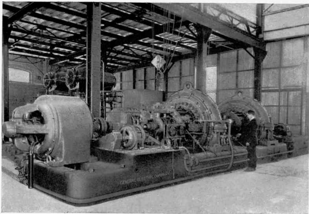
A 200-KILOWATT RADIO-FREQUENCY ALTERNATOR
