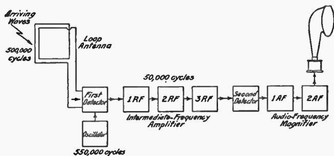
FIG. 67: Illustrative Diagram of Super-heterodyne Receiver. — The arrows represent the path of the signal currents and local oscillations through the system. Three general values of frequency are utilized: (1) a high radio frequency in the first-detector circuits; (2) a medium radio frequency in the intermediate amplifier; and (3) the audible or relatively low frequencies after the second detector.
