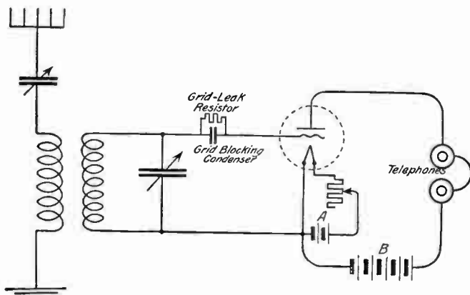
FIG. 51: An Audion Detector in the Two-Circuit Tuner. — Here we have replaced the crystal detector of Fig. 45 by an audion connected through the leak resistor and blocking condenser shown in the grid (or input) circuit. The A and B batteries, and the filament rheostat of Fig. 50, are also included. A pair of head-telephone receivers is included in place of the indicating meter used in Fig. 50. Note the square-sided zigzag symbol for resistance units, with the arrow-headed contact representing variability; also remember the symbols used for batteries and head-telephones.
