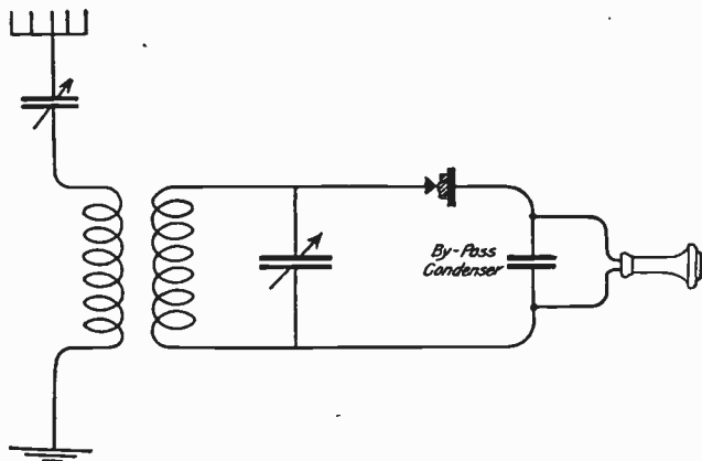
FIG. 46: How the By-Pass Condenser Is Used. — Except for the additional condenser in shunt to the telephones, this is the same as Fig. 45. Note that the arrow drawn through the parallel line symbol means that the condenser is variable . Here the by-pass condenser is of fixed (or constant) capacitance, and the arrow is omitted.
