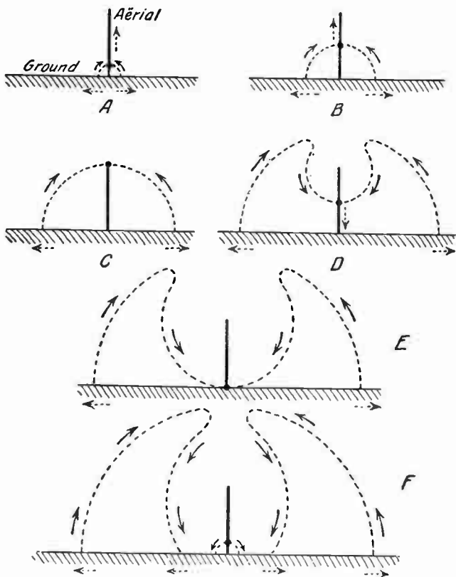
FIG. 23: Lines of Electrostatic Force around an Aërial. — We may imagine the feet of the lines of force to extend outward from the base of the aërial, as indicated by the dotted arrows; while the force-lines themselves follow the electric charge up and down the vertical wire. As suggested in A to E, the up-and-down cycle of charge movement creates a loop of electric force in the space surrounding the aërial. At F is indicated the casting-off of the first loop and the beginning of another. The act of freeing the first loop represents the creation of a radio wave. The solid arrows indicate the direction in which an electron would be urged by the electrostatic force whose intensity is traced by the dashed lines.
