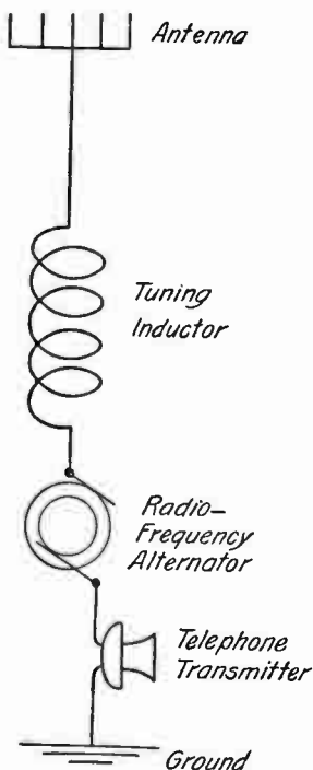
FIG. 31: A Simple Radio-Telephone Transmitter. — This is identical with the telegraph transmitter of Fig. 24, except that a microphone, or telephone transmitter, is substituted for the sending key. Instead of breaking up the continuous stream of current produced by the alternator, into dots and dashes, the microphone modulates it without interrupting its continuity.
