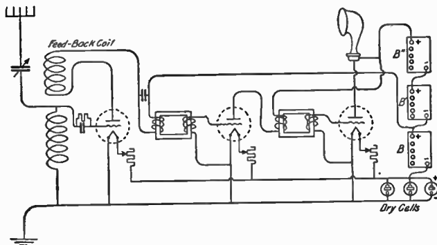
Fig. 66: Regenerator with Two-Stage Audio Amplifier. — This is the simple circuit of Fig. 65, combined with the amplifier of Fig. 56, which has been modified by eliminating the 6-volt storage battery A and using three WD-11 or three WD-12 "dry-cell tubes." Note the three dry cells connected in parallel to supply filament current to all three tubes. By placing the three dry cells in series and substituting 30-ohm rheostats, UV-199 tubes may be used.
