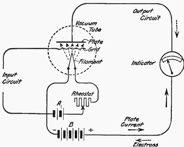
FIG. 50: Fundamental Circuits of the Audion. — The filament is heated by current from the battery marked A ; and its temperature controlled by the rheostat shown, as in Fig. 18. The plate-circuit battery B has its positive terminal connected to the plate, and its negative terminal to the filament, thus completing the output circuit containing the indicating device. The current in this output (or plate) circuit is made up of electrons that flow across the space from filament to plate within the vacuum tube, as indicated by the dashed arrows. The direction of electron flow is opposite to that conventionally assumed for electric "current" (positive to negative), as is shown by the solid arrows. By varying the potential applied to the grid by way of the input circuit, the amount of current flowing in the plate circuit (and registered on the indicating meter shown) can be controlled.
