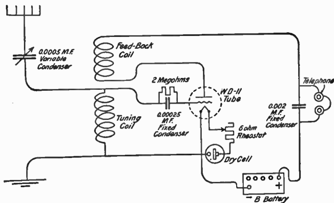
FIG. 65: The Simple Inductively-coupled Regenerator. — This easily built and adjusted circuit is giving excellent results in the hands of thousands of radio novices, and is a good one to begin with. The WD-12 tube, which fits a standard socket, may be substituted for the WD-11 tube shown. By suitably modifying the filament battery and rheostat, any other tube may be used.
