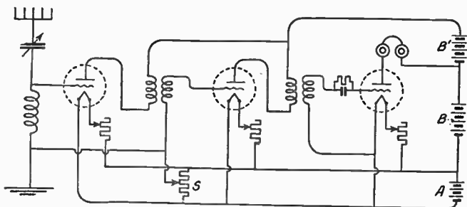
FIG. 59: Two-Stage Radio-Frequency Amplifier and Audion Detector, with Common Batteries. — A single set of batteries supplies current to all the tubes; and a single stabilizing potentiometer regulates both radio-frequency amplifiers. Otherwise the circuit resembles that of Fig. 58.
