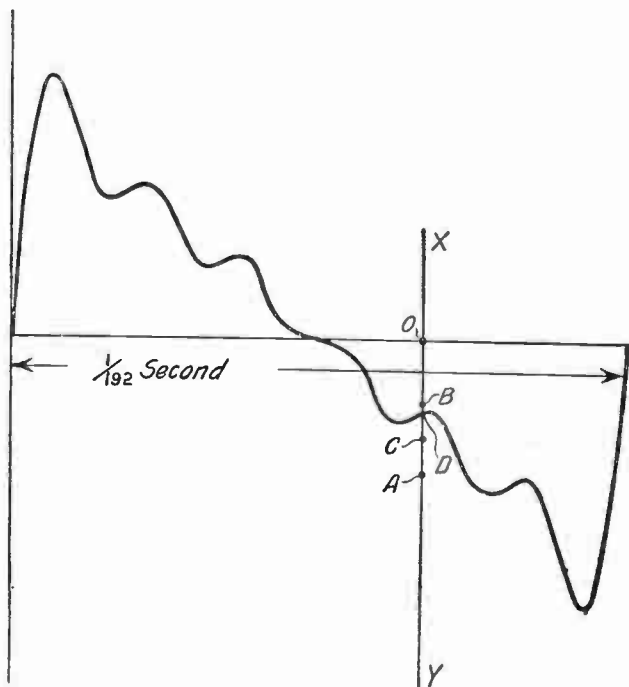
FIG. 28: A Violin Tone of 192-Cycle Pitch. — Such a curve-trace could be produced by playing a violin before the recording diaphragm of Fig. 26. Here it is drawn by adding together the six curves of Fig. 27. The process of adding is indicated in both figures at the lines X-Y , where the distances OA , AB , BC , and CD (Fig. 28) correspond in length and direction to the distances OA , A'B , B'C , and C'D (Fig. 27). The third and sixth harmonic partials contribute nothing to the resultant curve for this particular position of the "line of addition" X-Y .
