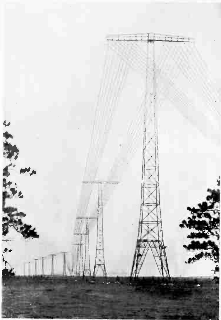
THE TWELVE 400-FOOT TRANS-ATLANTIC TOWERS OF THE RADIO CORPORATION'S STATION AT ROCKY POINT, LONG ISLAND, N. Y.
