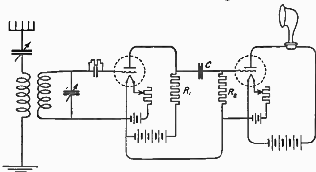
FIG. 53: Condenser-coupled Single-Tube Amplifier, with Audion Detector. — A circuit arrangement like that of Fig. 52, except for the use of fixed condenser C and resistors R_1 and R_2 in place of the amplifying transformer, for linking the detector to the amplifier. R_1 is usually of about 50,000 ohms resistance, and R_2 (a leak resistor) of about 2,000,000 ohms. The fixed condenser may be relatively large, or about one microfarad.
