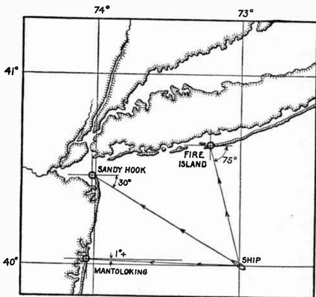
FIG. 68: Determining a Ship's Position by Radio. — The Radio Compass station at Fire Island finds that radio signals from the ship illustrated, come in along a line 75^\circ south of east. Sandy Hook hears the same signals along the line running 30^\circ south of east. When these two lines are drawn on a chart, their point of crossing will be found to be at 73^\circ longitude and 40^\circ latitude, which is the ship's position while sending. A third observation from Mantoloking (in this case a little over 1^\circ south of east) will check the other two readings. If the three lines cross in a single point, the determination is accurate; but if they enclose a large triangle, the position of the ship will not be definitely known.
