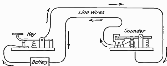
FIG. 9: The Simple Electric Telegraph. — The arrows indicate the direction in which the electric current will flow around the circuit as soon as the sending key is pressed down.
