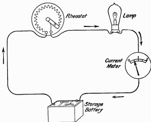
FIG. 18: A Battery Circuit of Variable Resistance. — With all of the rheostat (6 ohms) in series with the lamp (also 6 ohms), the 6-volt storage battery will force \frac{1}{2} an ampere of current through the circuit. As the handle of the rheostat is turned to the left, so reducing the amount of resistance in circuit, the ammeter (current meter) will show the current increasing to 1 ampere.
