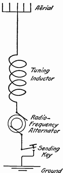
FIG. 24: Continuous-Wave Radio-Telegraph Transmitter. — This circuit is the same as that of Fig. 22, except that a sending key is added to make and to break the current path and so to control the radiation of waves. Note the conventional symbols used to represent aerial, key, and earth.
