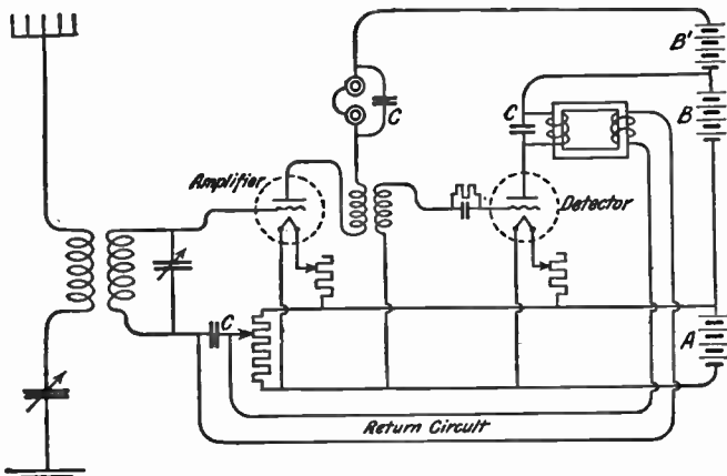
FIG. 63: A Two-Tube Reflex Amplifier. — The order of connecting the instruments in each circuit is very important; and the size of the three by-pass condensers marked C must be carefully chosen. Note how the rectified audio-frequency current from the detector is brought back through the return circuit from the transformer secondary coil to the grid circuit of the first tube, to be amplified again before reaching the telephones.
