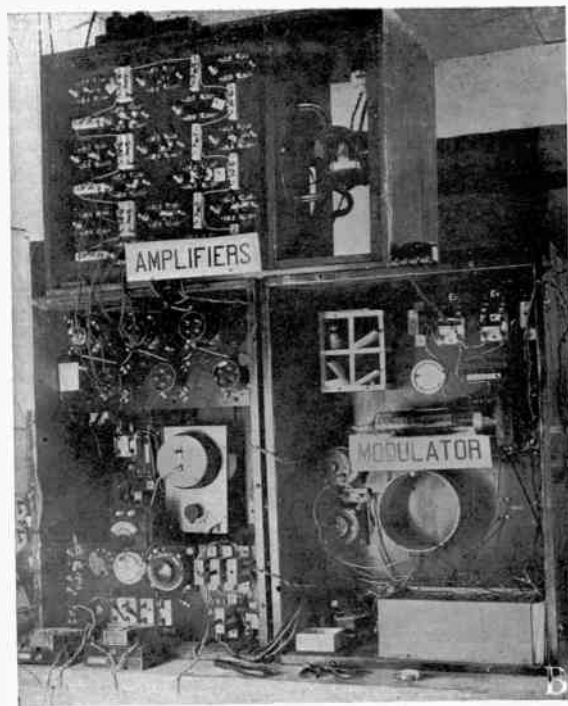
THE RADIO-TELEPHONE TRANSMITTING APPARATUS USED AT ARLINGTON (VA.) FOR THE LONG-DISTANCE EXPERIMENTS OF 1915
