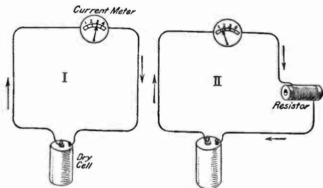
FIG. 17: The Effect of Resistance. — The simple circuit at I passes 3 amperes as shown by the meter. When a resistor of \frac{1}{2} an ohm is inserted in the circuit, as at II, the 1\frac{1}{2} volt dry cell can force only 1\frac{1}{2} amperes through the circuit. The arrows indicate the direction of current flow, according to the usual convention.
