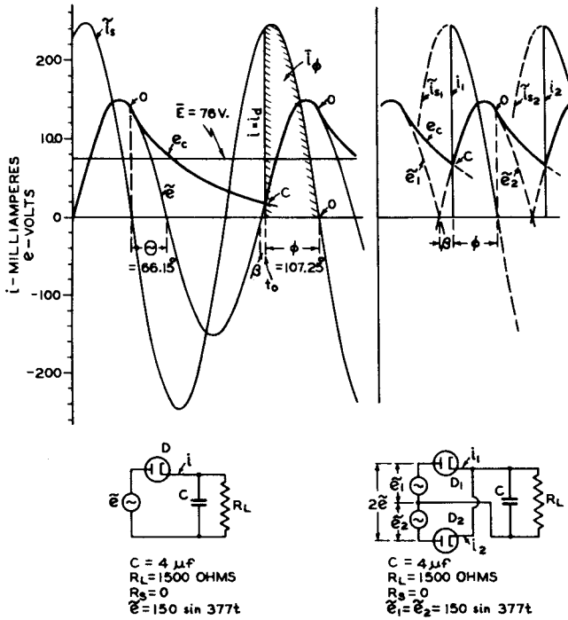
Fig. 13 (left) - Half-wave, condenser-input circuit without series resistance. Fig. 14 (right) - Full-wave, condenser-input circuit without series resistance.
