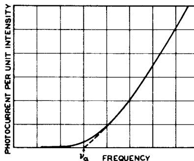
Fig. 3 - Typical spectral distribution curve, showing extrapolation to determine \nu_a (exaggerated). (L. A. DuBridge, see Bibliography)
