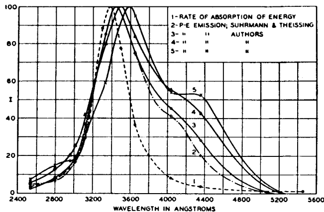
Fig. 4 - Calculated and observed photoelectric emission from thin film of potassium on platinum. (Ives & Briggs, J.O.S.A., Vol. 26, p. 249, 1936).
