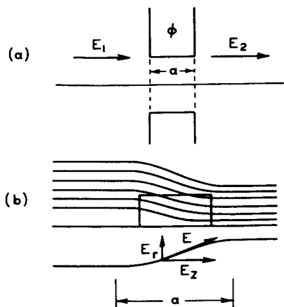
Fig. 9 - Idealized field distribution in simple aperture lens.
