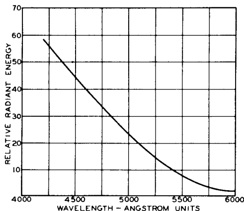
Fig. 9 - Spectral energy characteristic of phosphor No.5.
