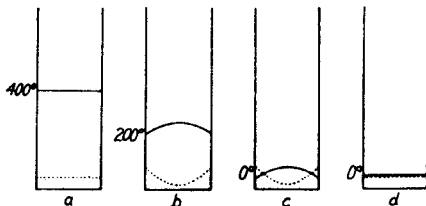
Fig. 6 - Similar to Fig. 5 except that the glass is cooled from a temperature below the annealing range, in which case no permanent strain is introduced. (From Jour. Franklin Inst., Vol. 190, No.5, page 603; 1920).
