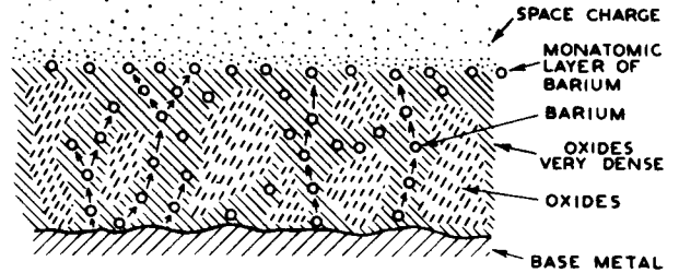
Fig. 4 - Structure of cathode coating.
