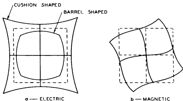
Fig. 6 - Distortion.
