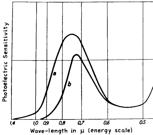
Fig. 13 - Spectral distribution curve of a Ag:Cs 2 O, Ag-Cs cathode: (a) in a fresh state; (b) after fatigue has set in. (J. H. DeBoer, see Bibliography) Courtesy of The Macmillan Company
