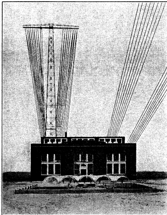
The Power House at Radio Central.
