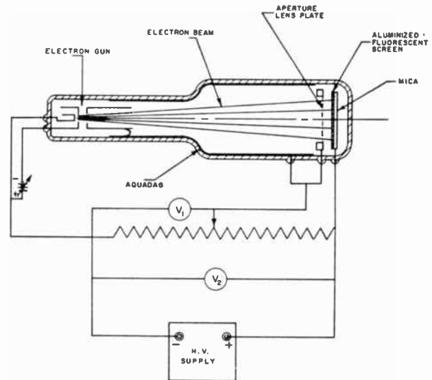
Fig. 2—Diagram of a tube used for studying the aperture lens.
