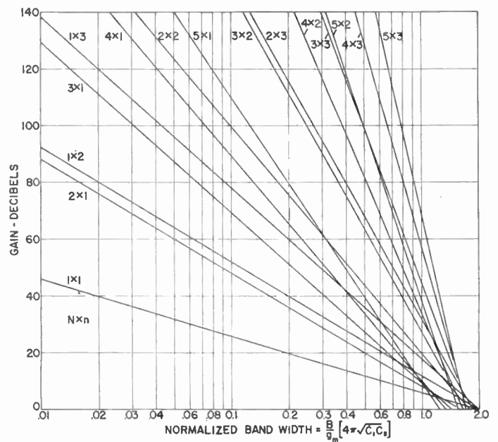
Fig. 5—Gain vs bandwidth for different amplifier configurations.
