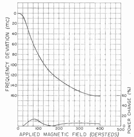
Fig. 1—Frequency deviation and power change as functions of the applied magnetic field for a ferrite in the external cavity of a klystron.
