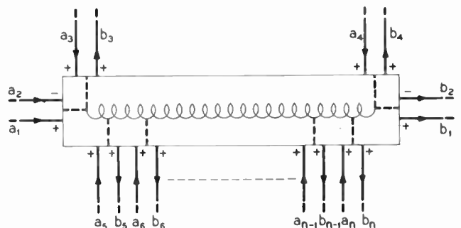
Fig. 3—Traveling-wave tube with distributed loss.
