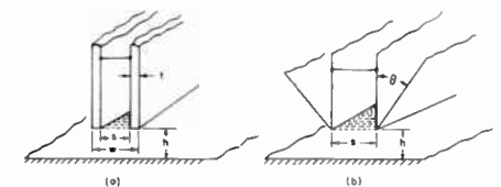
Fig. 3—(a) Fins of finite thickness facing a ground plane. (b) Sharpened fins facing a ground plane.
