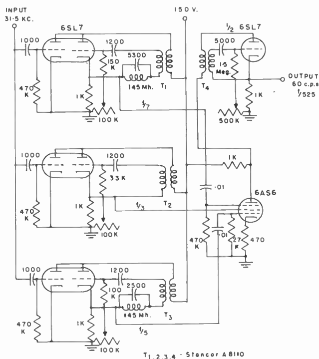
Fig. 4—Schematic diagram of a counter circuit which uses the pulse-coincidence principle. For the transformers indicated, in T 1, T 2 and T 3 the green lead is the plate, and the blue lead the grid connection. In T 4 the plate lead is blue, and the grid lead is green.
