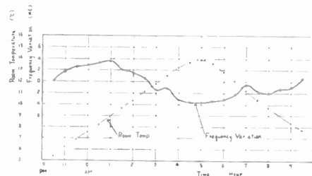
Fig. 3—Long-time stability of this equipment.
