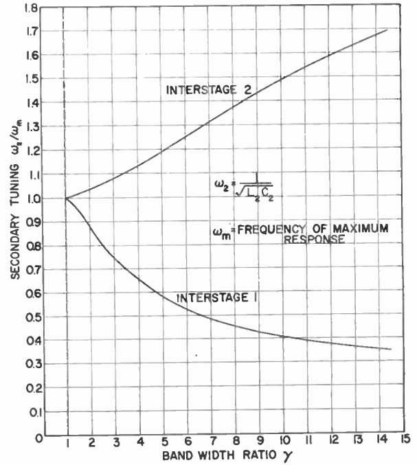
Fig. 9—Secondary tuning \omega_2/\omega_m vs bandwidth ratio \gamma for a staggered double.
