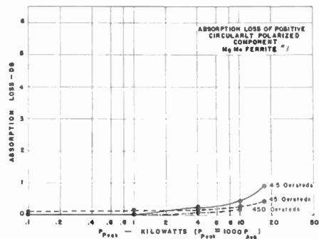
Fig. 2—Power absorbed from a positive circularly polarized wave by a ferrite cylinder ( \frac{1}{4} inch diameter X 2 inches length) versus the peak power, the applied longitudinal magnetostatic field as a parameter.
