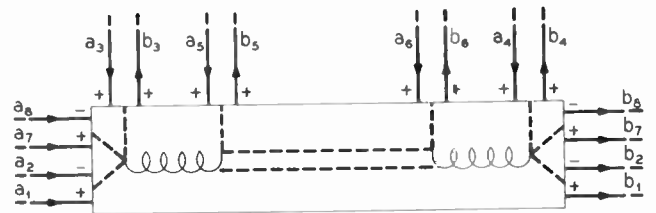
Fig. 5—Double-stream amplifier.
