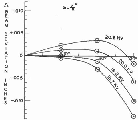
Fig. 5—Beam deviation vs deflection angle as calculated from (10) for various values of V_s . V_a=9.80 kv, V_p=3.60 kv, r=12.7 inches, b=3/16 inch, d=0.400 inch.
