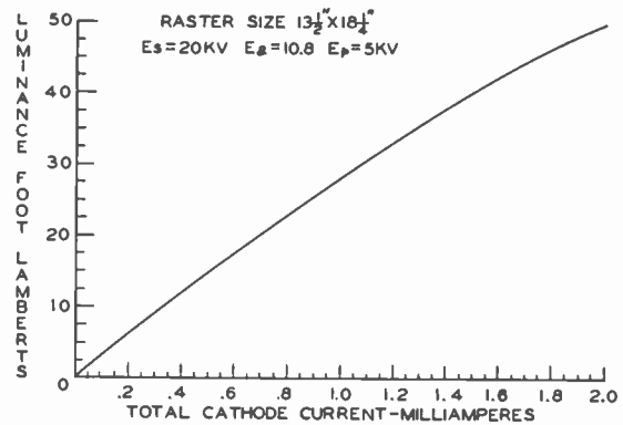
Fig. 9—Luminance vs total cathode current characteristic.
