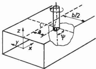
Fig. 1—Rotatable pure inductive probe in a rectangular waveguide.
