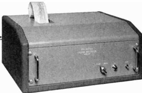
Model 1452 prints 6 digits (8 or 10 on special order) on standard adding machine tape. Is only 19" wide x 10 1/2" high x 14" deep, weighs 60 lbs. Price, $750.00 f.a.b. factory.
