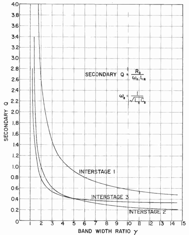
Fig. 15—Secondary Q vs bandwidth ratio \gamma for a staggered triple.
