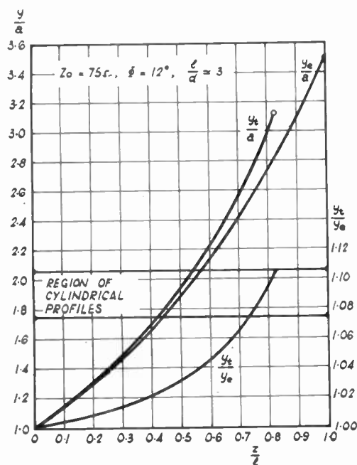
Fig. 5—Profiles of various jackets.
