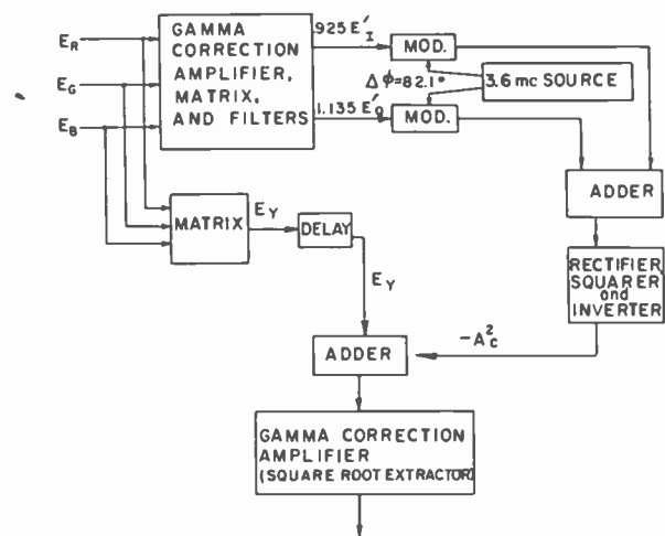
Fig. 3— E_{Y_T} generation.
