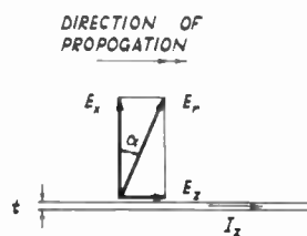
Fig. 6—The field at the surface of the resistor.
