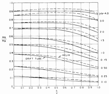
Fig. 1—The plasma frequency reduction factor, \omega_q/\omega_p , for solid electron beams as a function of the ratio of the beam radius b to a coaxial helix or drift tube of radius a for several values of \gamma b .
