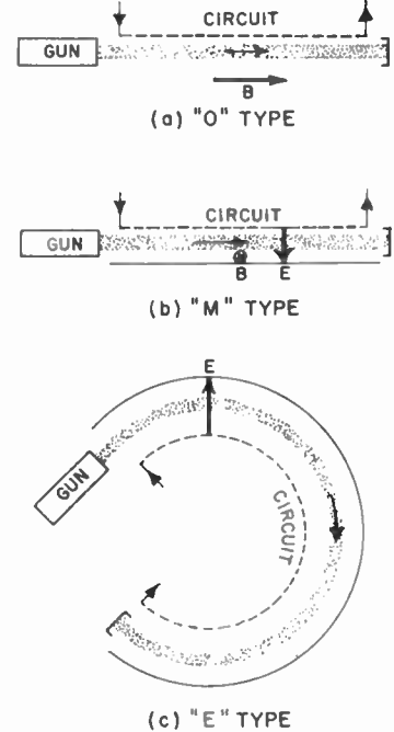
Fig. 1—Schematic representation of three forms of beam-type tubes. In the drawings the symbols E and B indicate static electric and magnetic fields respectively, the "M"-type (b) may also be formed into a circle but here centrifugal force is small compared with electric and magnetic forces.
