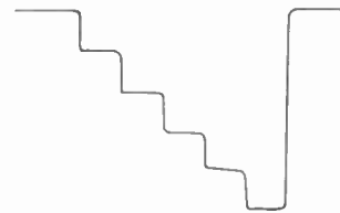
Fig. 9—Quantized output as observed on scope with optimum adjustment of correcting wires (system of Fig. 8).
