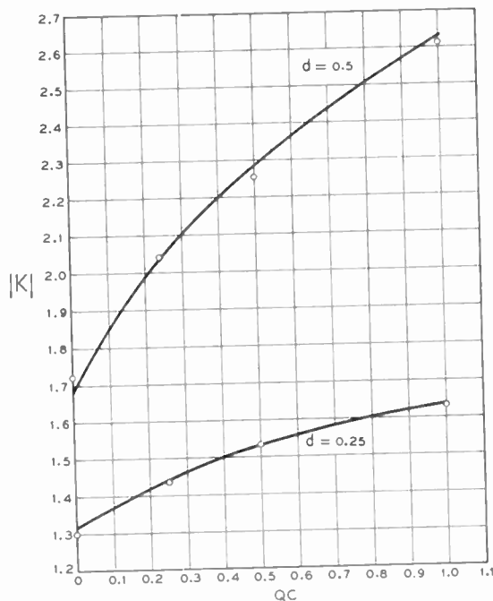
Fig. 4— |K| for a lossy helix. The curves represent Pierce and Danielson's results. The points are calculated from (1) to (6).
