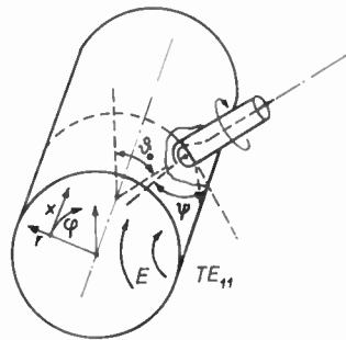
Fig. 3—Rotatable probe in a circular waveguide.
