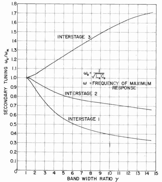
Fig. 13—Secondary tuning \omega_2/\omega_m vs bandwidth ratio \gamma for a staggered triple.
