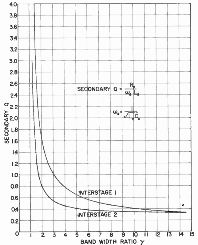
Fig. 11—Secondary Q vs bandwidth ratio \gamma for a staggered double.
