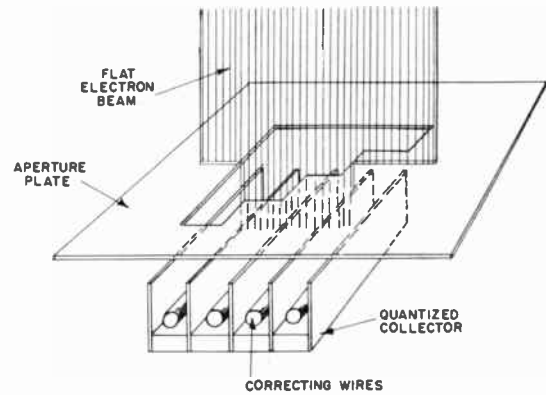
Fig. 5—Target assembly.
