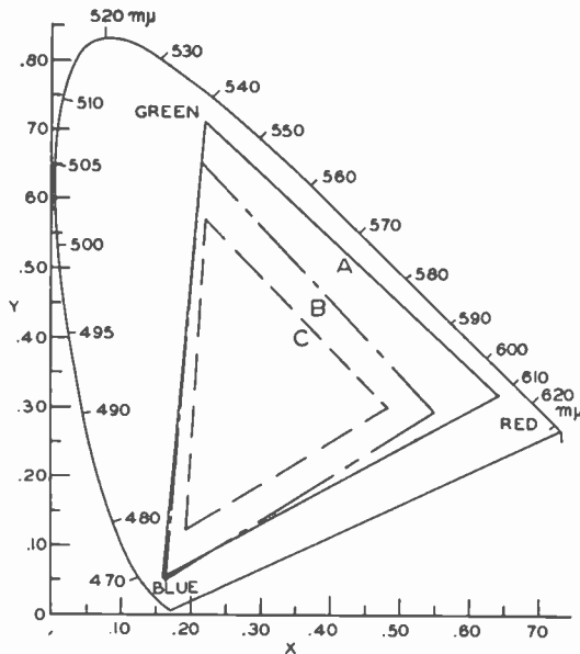
Fig. 10—CIE chromaticity diagram with the color gamuts obtainable on: A, straight parallax mask tube; B, post-acceleration tube with both retarding and accelerating field; C, post-acceleration tube with a single field.
