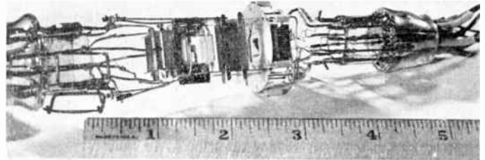
Fig. 12—Photograph of beam-forming and target sections of the quantizing tube.
