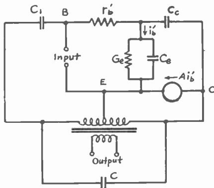
Fig. 9—Partially-neutralized base input IF amplifier.
