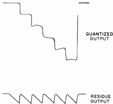
Fig. 7—Output of quantizing tube as observed on scope (system of Fig. 5).
