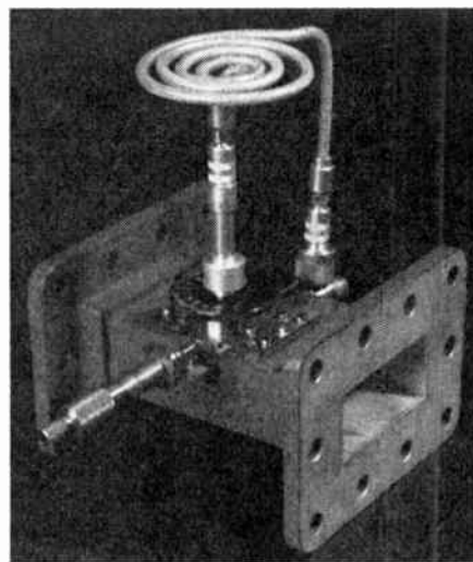
Fig. 7—Prototype of a standing-wave detector with rotatable probe.
