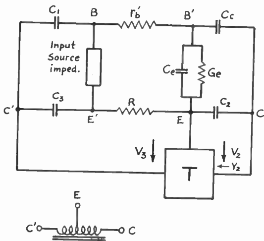
A practical network T
