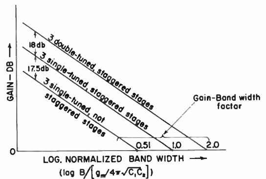
Fig. 3—Comparison of different types of three-stage amplifiers.
