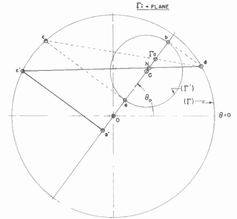
Fig. 1—Determination of maximum efficiency.
