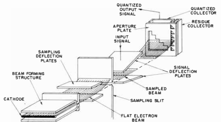
Fig. 4—Arrangement of the elements in the sampling and quantizing tube (suppression and adjustment electrodes have been omitted for simplicity).
