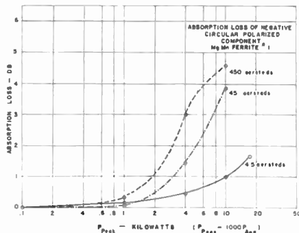
Fig. 1—Power absorbed from a negative circularly polarized wave by a ferrite cylinder ( \frac{1}{4} inch diameter X 2 inches length) versus the peak power, the applied longitudinal magnetostatic field as a parameter.
