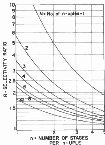
Fig. 6—Selectivity ratio as a function of N , the number of n -uples, and n , the number of stages per n -uple.
