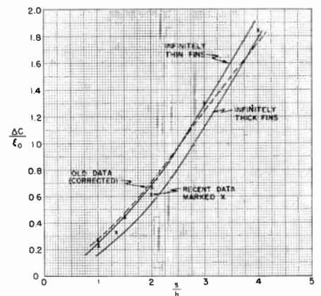
Fig. 2—Normalized capacity change as a function of the ratio of slot spacing to slot height above ground plane.
