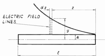
Fig. 2—The assumed field distribution in the exponential termination.
