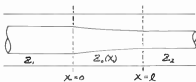
Fig. 1—Matching section between impedances Z_1 and Z_2 .
