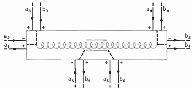
Fig. 2—Traveling-wave tube with center loss.
