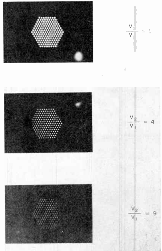
Fig. 4—Photographs of the dot pattern produced on the fluorescent screen of the tube shown in Fig. 2, for various V_2/V_1 ratios.
