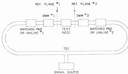
Fig. 2—Microwave circuit.
