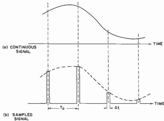
Fig. 3—Time sampling.
