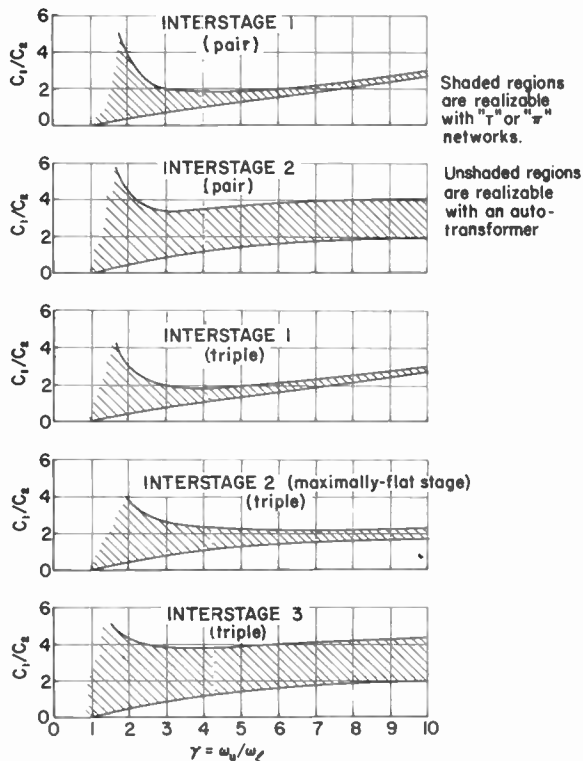
Fig. 4—Regions of physical realizability for the auto transformer and the "T" or "π" equivalents.
