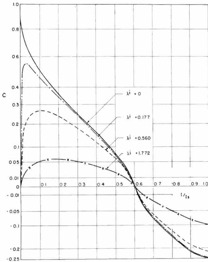
Fig. 4—Detection sensitivity factor C as a function of current for various values of \lambda^{1/2} . For I_s = 1 \text{ A/cm}^2 and T = 1,000 degrees K., \lambda^{1/2} = 1.772 corresponds to a frequency of 10^4 \text{ mc.} , \lambda^{1/2} = 0.560 to 3.10^3 \text{ mc.} , \lambda^{1/2} = 0.177 to 10^3 \text{ mc.}
