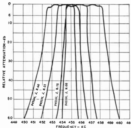
F455H, J and K New tubular case mounting, temperature compensated for signals at 455 kc. Bandwidths of 0.8, 1.5, 3.1 and 6.0 kc at 6 db attenuation. Transmission loss, 10 db.
