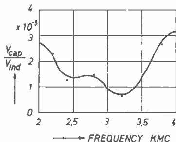
Fig. 6—Ratio of the capacitive to the inductive component of the probe voltage induced in a compensated inductive probe.
