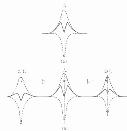
Fig. 1—Differential figures of two resonance curves. (a) Single Modulation. (b) Double Modulations.
