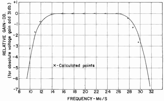
Fig. 17—Measured frequency response of double-tuned staggered pair.
