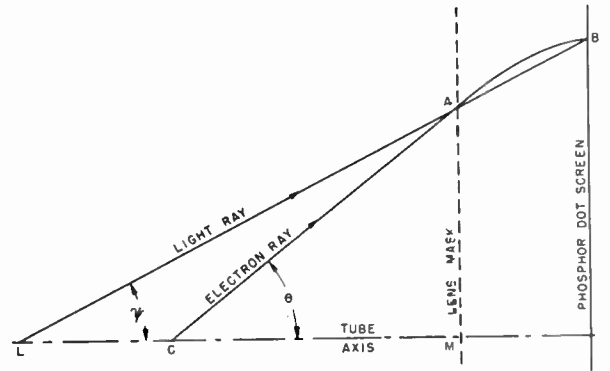
Fig. 7—Diagram to illustrate electron ballistics of the lens mask.
