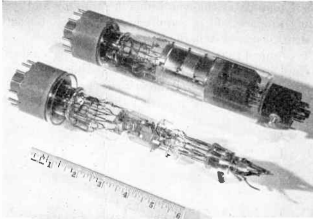
Fig. 11—Photograph of time-sampling and amplitude-quantizing tube.
