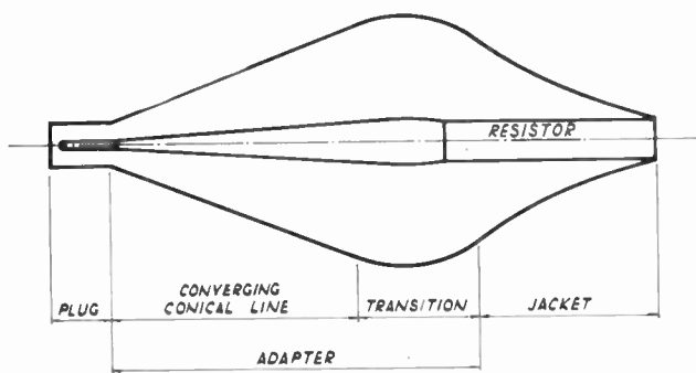
Fig. 9—General layout of a tractorial termination.
