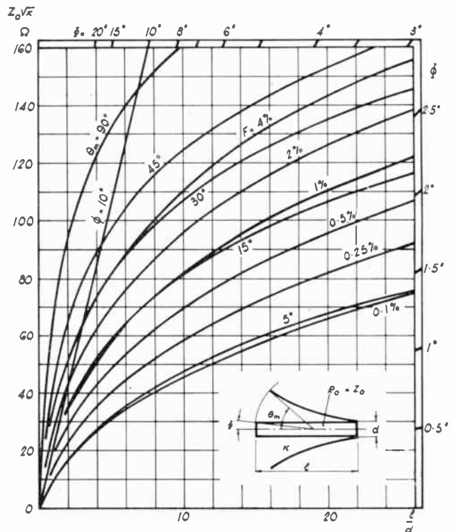
Fig. 8—Dependence of \theta_m , F and \Phi on the characteristic impedance and on the l/d ratio.
