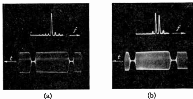
Fig. 5—Effect of oscillator tuning on the frequency spectrum obtained with relatively long pulses; f_0 = 10 \text{ mc} and f_1 = 40 \text{ kc} .
