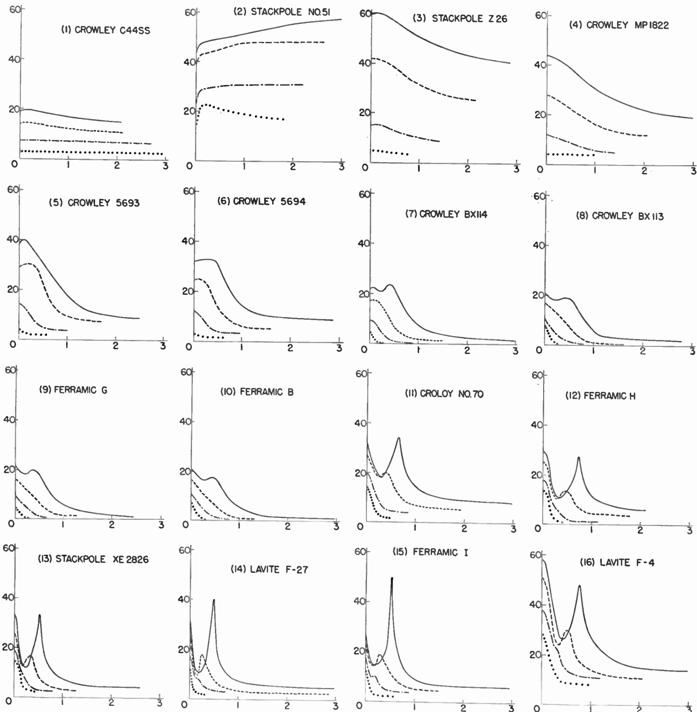
Fig. 6—Attenuation in decibels versus electromagnetic current in amperes is shown for the magnetic attenuator using various dissipative materials. The name of the material is shown on each family of curves. In each case, the solid curve represents a frequency of operation of 3000 mc and the other curves correspond in descending order to frequencies of 2000, 1000, and 300 mc.
