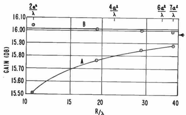
Fig. 7—Experimental results
