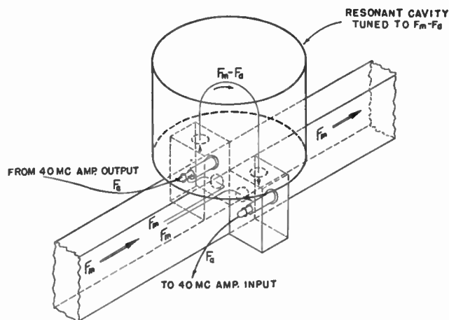
Fig. 5—Arrangement of the tunable frequency reference cavity and crystal mixers.
