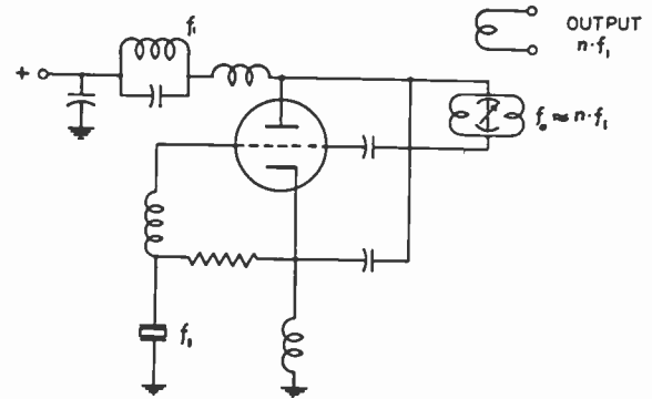
Fig. 3—Schematic diagram of a complete uhf spectrum generator.
