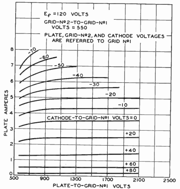
Fig. 9—Average plate characteristics of Type 6181
