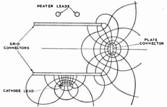
Fig. 6—Approximate cross section of the 6AJ4 lead configuration with a flux plot to indicate the degree of inductive isolation between input and output current paths.
