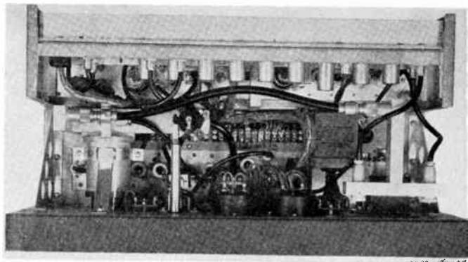
Fig. 7—Receiver RF assembly.
