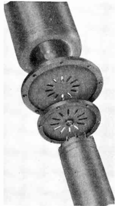
Fig. 3—Axial-flow resnatron electrodes including anode, screen grid, grid, and cathode.
