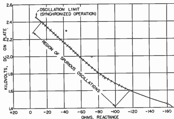
Fig. 3—Loop reactance at 825 mc at different plate voltages of a nonoscillating magnetron measured at plane L.
