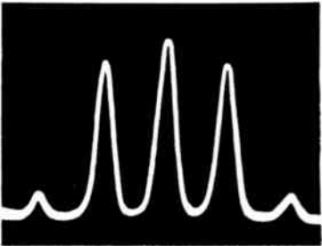
Modulation Index 1.3
