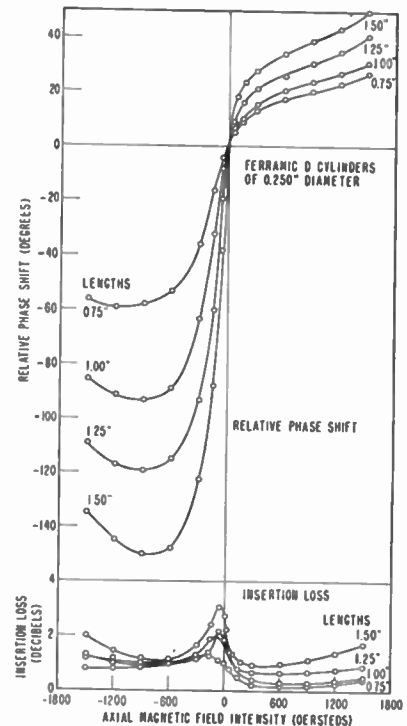
Fig. 4—Relative phase shift and insertion loss versus applied axial magnetic field intensity with the length of the sample as a parameter in the case of circularly polarized wave propagation.
