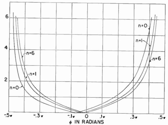
Fig. 3(b)— |\theta / \theta_n^2(1 + \theta \tan \phi)| versus \phi .
