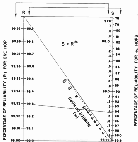
Fig. 15—System reliability.
