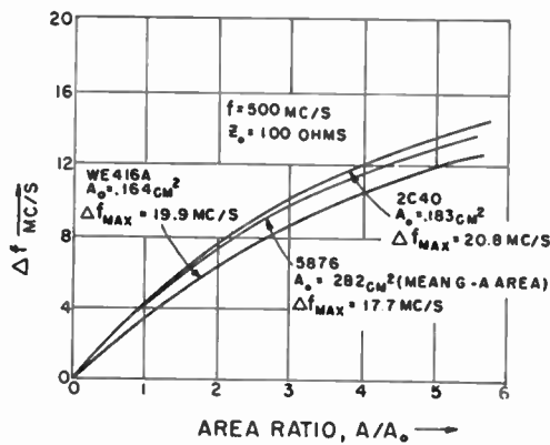
Fig. 13—Operating bandwidths as a function of area ratios. A_0 = cathode area of individual commercial tube. A = cathode area of hypothetical tube.
