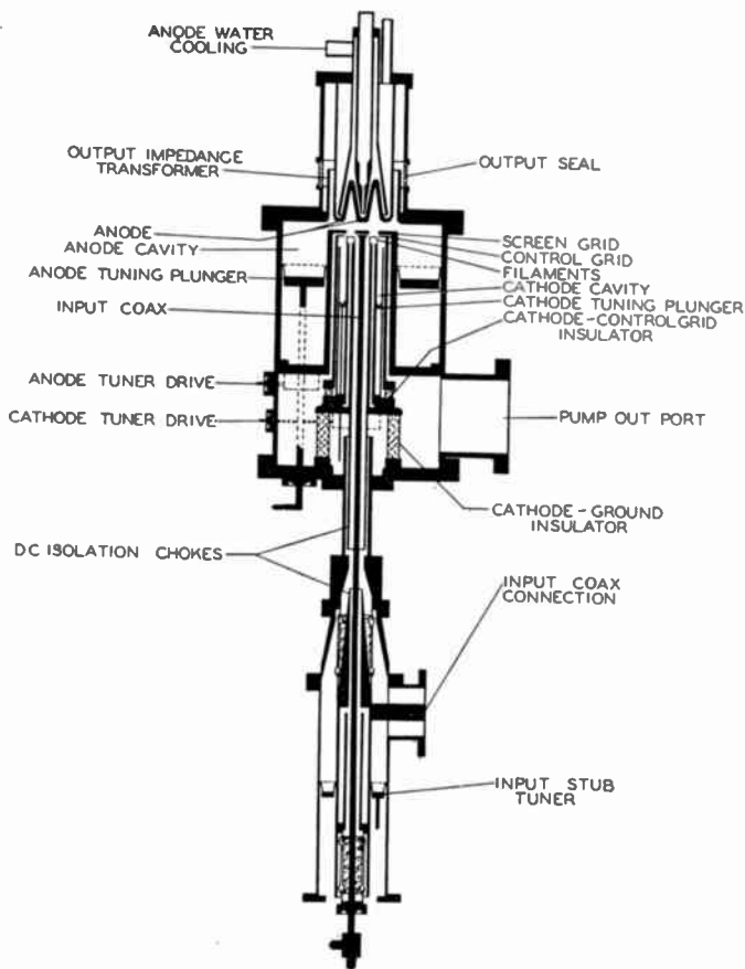
Fig. 2—Cross-section schematic of axial-flow resnatron.
