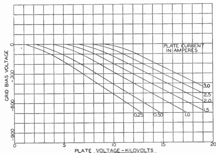
Fig. 5—Constant-plate current curves.
