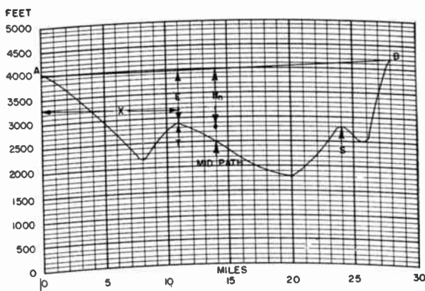
Fig. 9—Large clearance path (4/3 earth profile paper).
