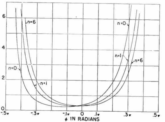
Fig. 3(d)— |\theta^2 / \theta_n^4(1 + \theta^2/3 + 2\theta \tan \phi + \theta^2 \tan^2 \phi)| versus \phi .
