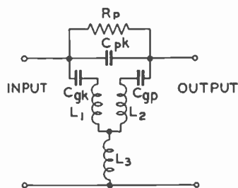
Fig. 4—The approximate equivalent circuit responsible for coupling between input and output circuits of the 6AJ4.
