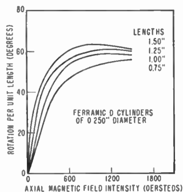
Fig. 5—Calculated angle of rotation of the plane of polarization versus applied axial magnetic field intensity.
