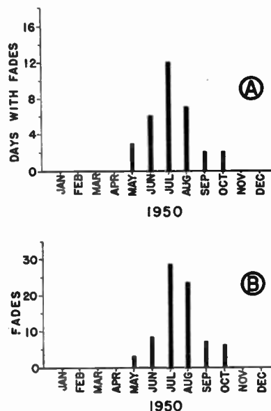
Fig. 6—Summary of fading 10 db or more below median field strength. (A) Number of days with fading. (B) Number of individual fades.
