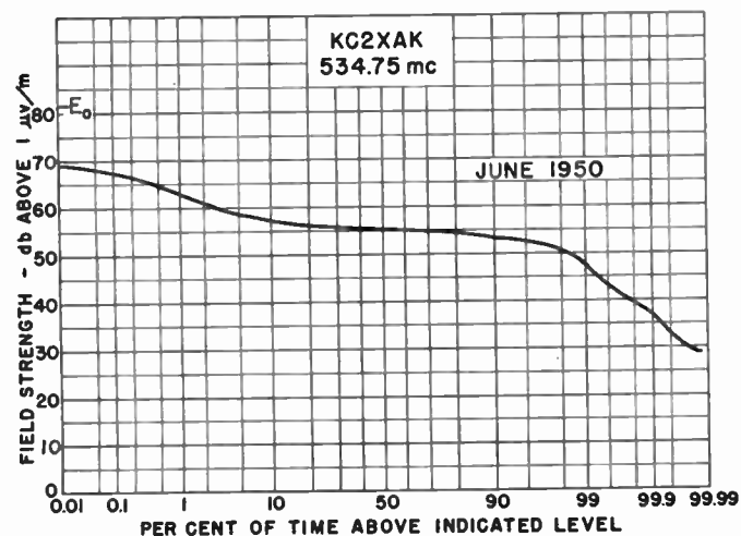
Fig. 3—Typical field-strength distribution for summer months.
