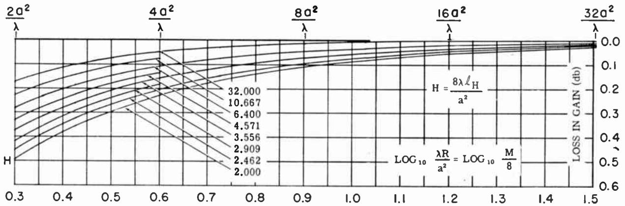
Fig. 5— H -plane correction curves.
