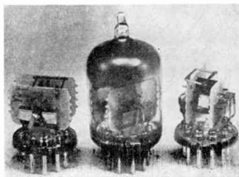
Fig. 5—Tube and mounts showing the construction of the 6AJ4.
