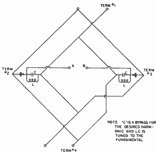
Fig. 10—Harmonic generator.
