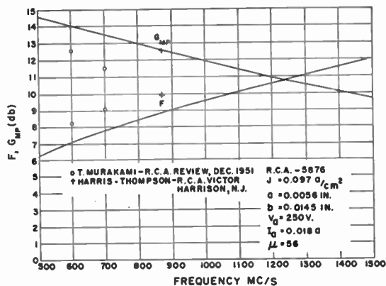
Fig. 12—Computed and measured performance of RCA 5876 triode.
