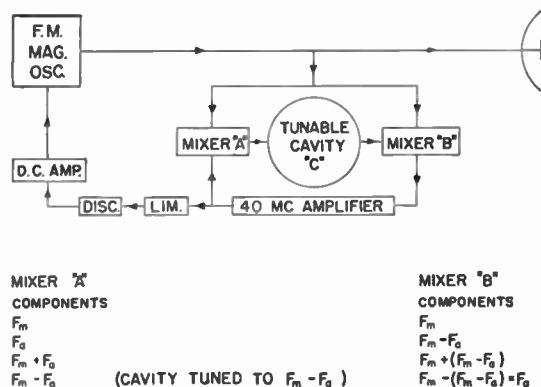
Fig. 4—Block diagram of the frequency stabilization circuit. Arrows indicate direction of the principal frequency components.
