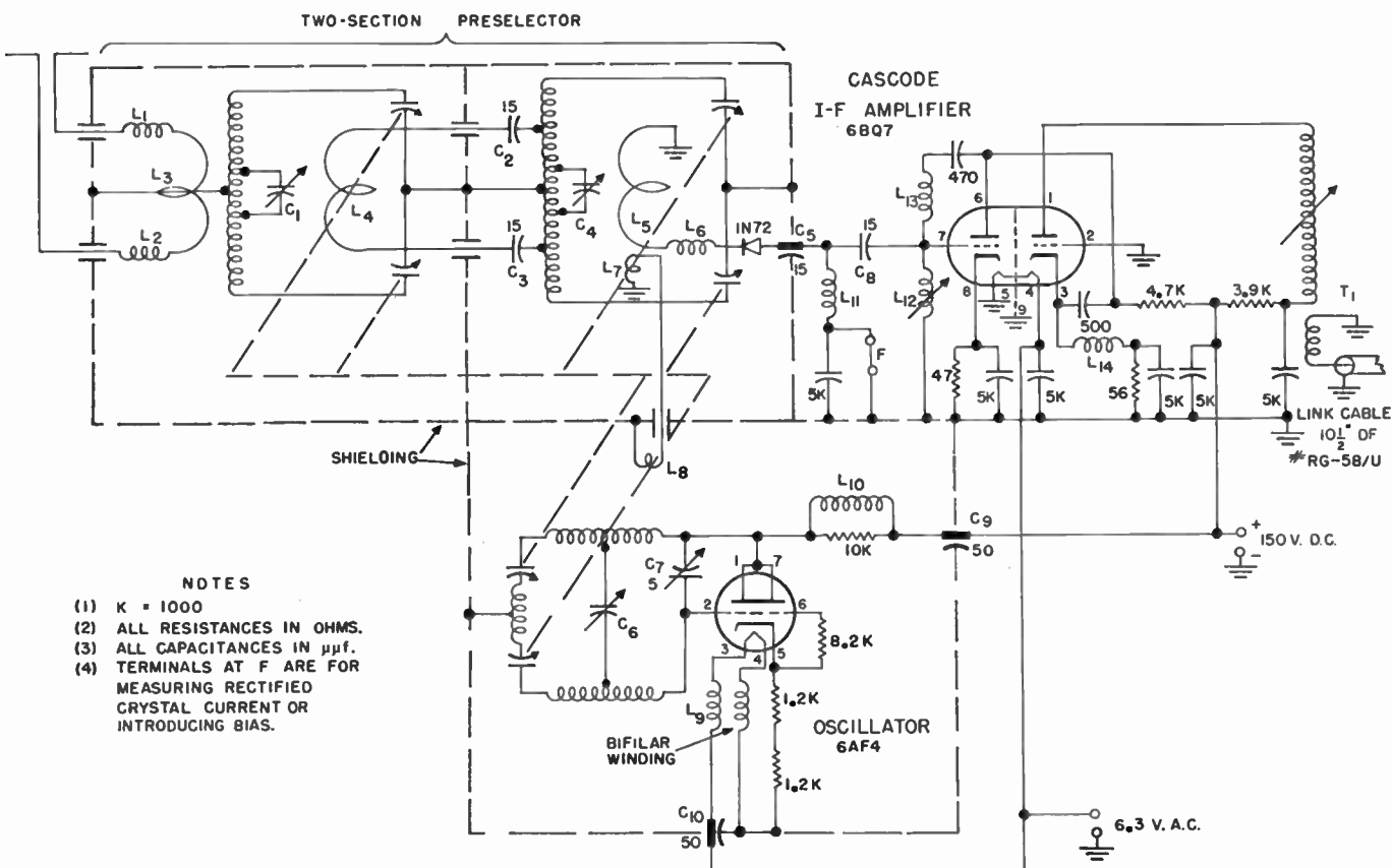
Fig. 3—Schematic circuit.
