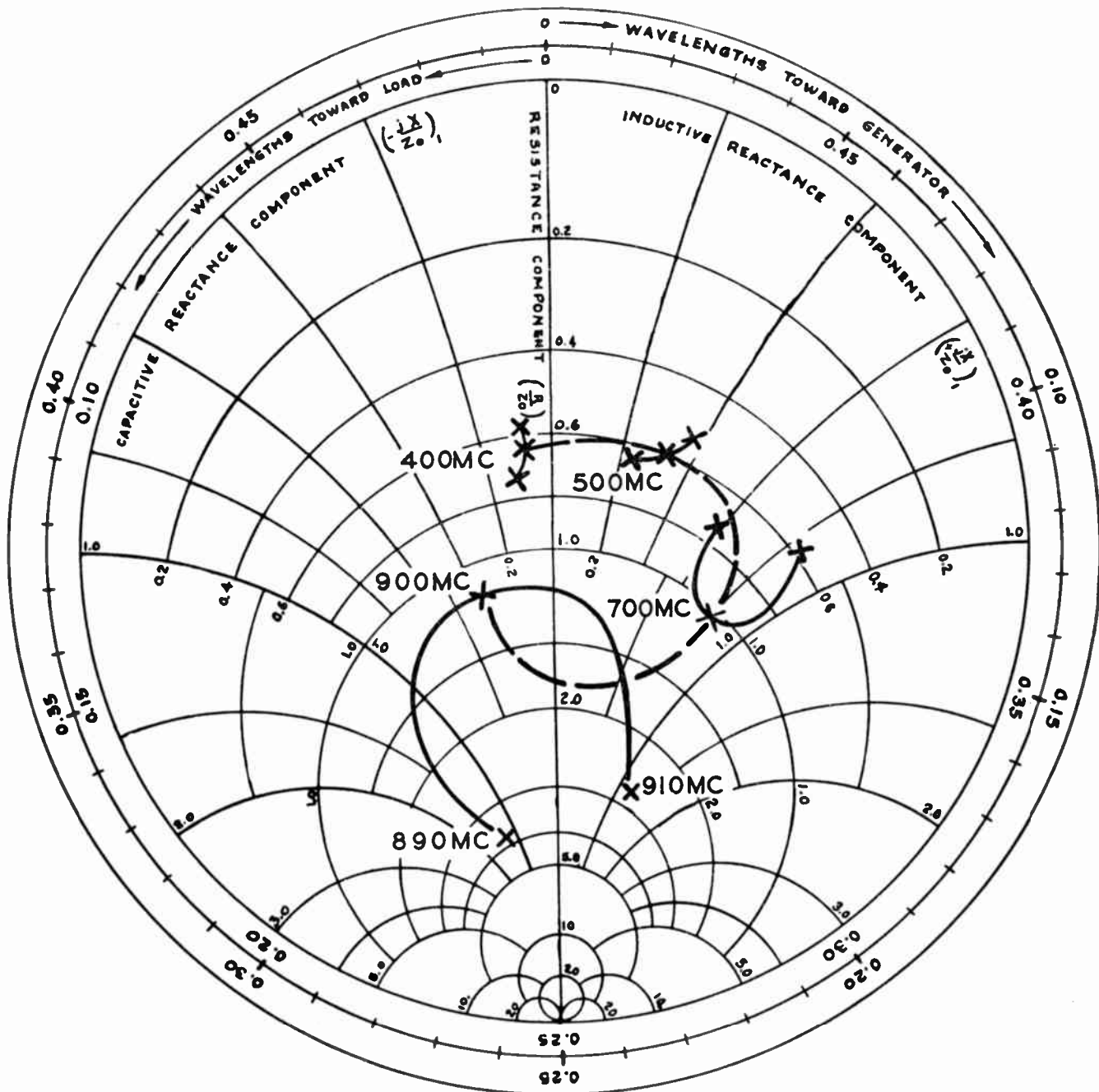
Fig. 2—Smith chart plot showing the excessive input impedance variations of an early developmental tube.
