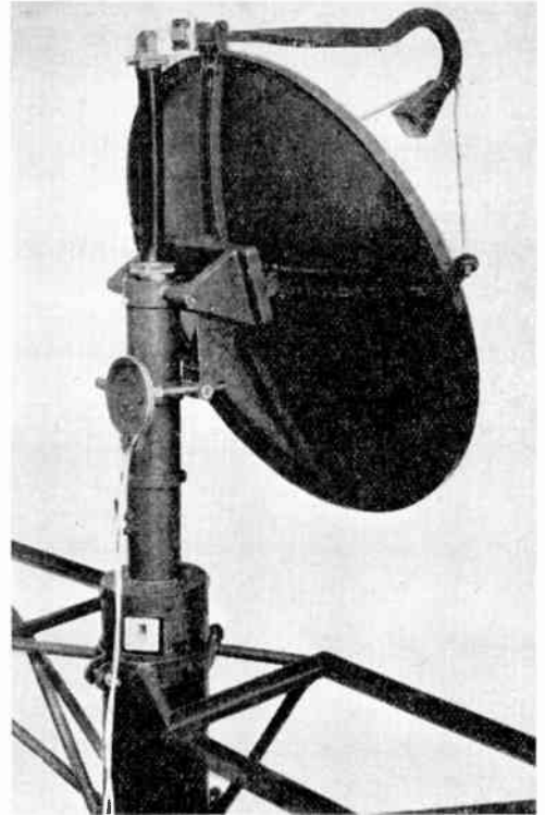
Fig. 3—Antenna assembly shown mounted directly on the hybrid T and RF equipment support.
