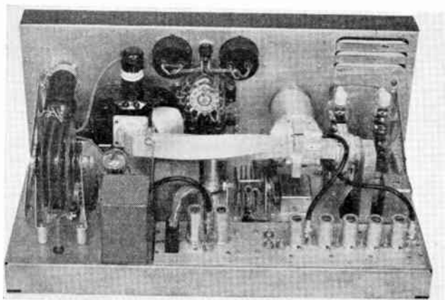
Fig. 6—Transmitter RF assembly.
