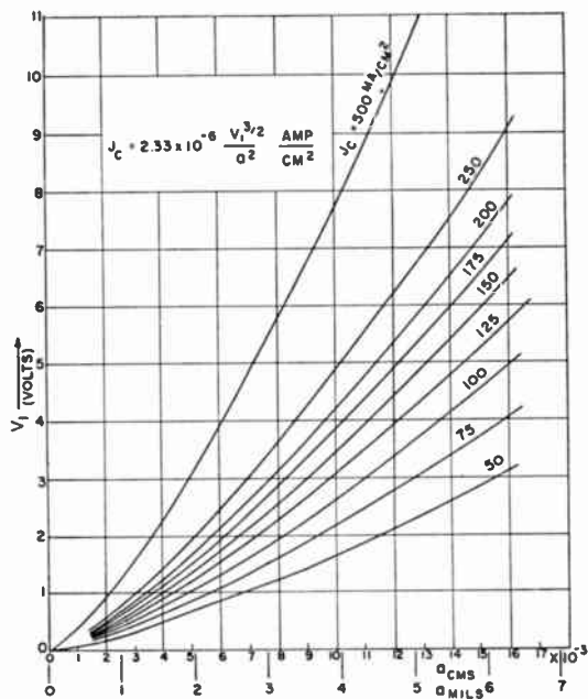
Fig. 2—Equivalent diode characteristics. J_c =cathode current density, amperes/cm 2 , V_1 =grid plane equivalent voltage, volts, and a =grid-cathode spacing, cm.
