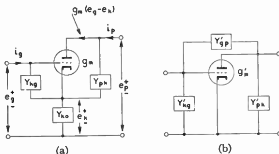
Fig. 2—Common cathode transformation. (a) Star connection. (b) Delta connection.
