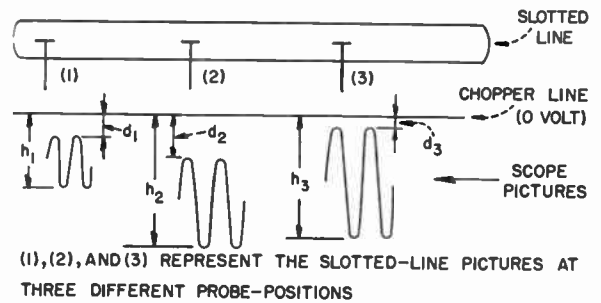
Fig. 5—Changes of detected modulation envelopes, as observed on the scope along the slotted line.
