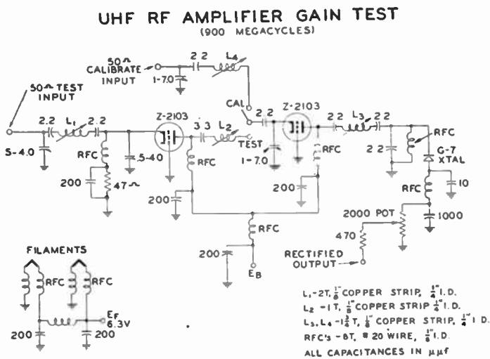
Fig. 7—Circuit diagram of a two 900-mc amplifier.
