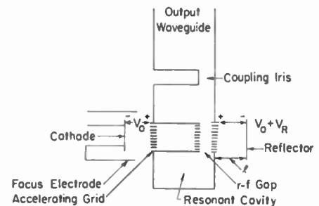
Fig. 2—Schematic sketch of reflex klystron.
