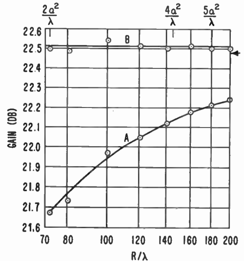
Fig. 6—Experimental results.
