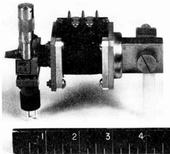
Fig. 2—Microwave elements of basic magnetometer.
