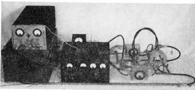
Fig. 4—Experimental 1.1-kmc 20-per cent bandwidth correlator.
