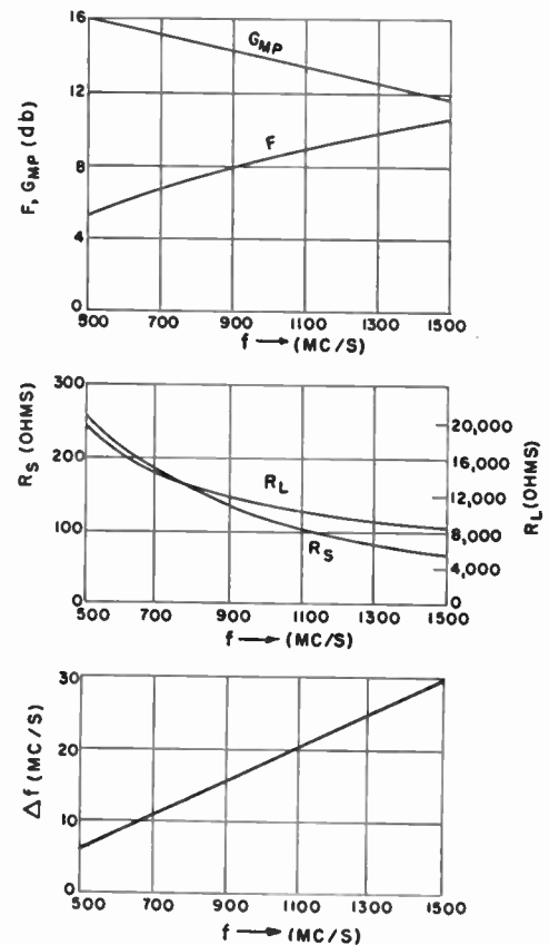
Fig. 14—Computed performance of hypothetical uhf television triode.
