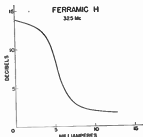
Fig. 8—Control of attenuation using small electromagnet.
