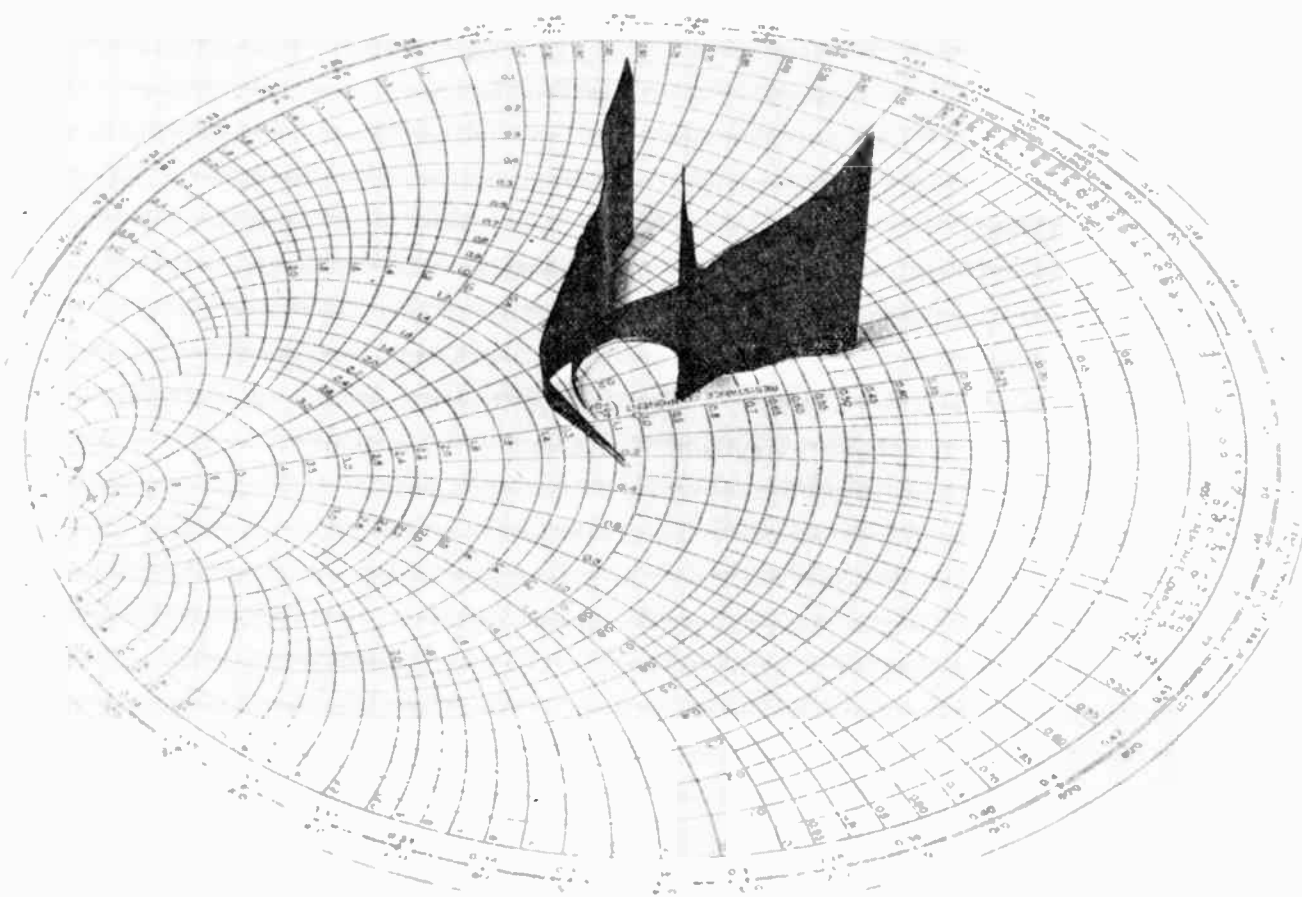
Fig. 13—Photograph of a three-dimensional plot of the attenuation and impedance changes obtained with a magnetic attenuator as the electromagnet current is increased from zero to 3 amperes. Two graphs are shown, one for an operating frequency of 3000 mc (on the right) and the other for a frequency of 2000 mc. Attenuation is plotted vertically, the two horizontal lines corresponding to 10 and 20 db. The normalized impedance is shown on the horizontal Smith chart. The dissipative material is Croloy No. 20.
