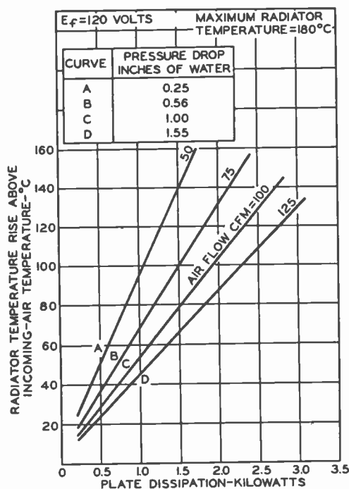
Fig. 8—Cooling requirements of Type 6181.
