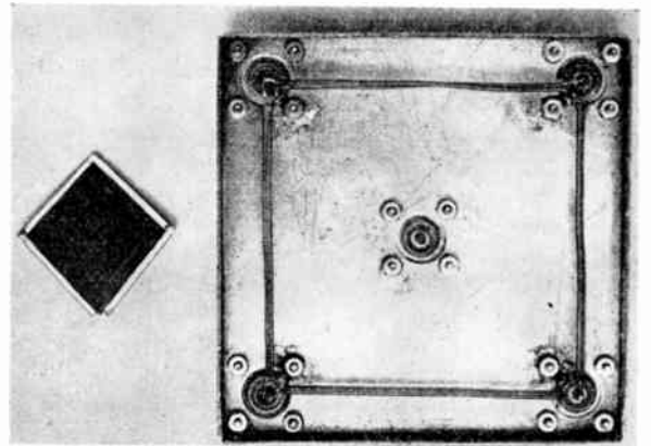
Fig. 6(b)—Printed circuit wide-band hybrid ring and twin-lead version using unbalanced feeds.
