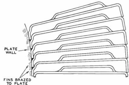
Fig. 7(b)—Radiator fin assembly.
