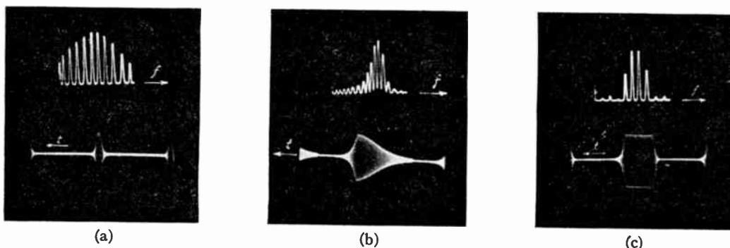
Fig. 4—Wave shape and frequency spectrum for relatively short pulses; f_0 = 10 mc.
