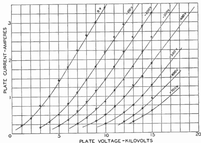
Fig. 4—Plate current versus plate voltage curves for constant-grid voltages as indicated.
