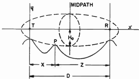
Fig. 2—Free-space clearance.
