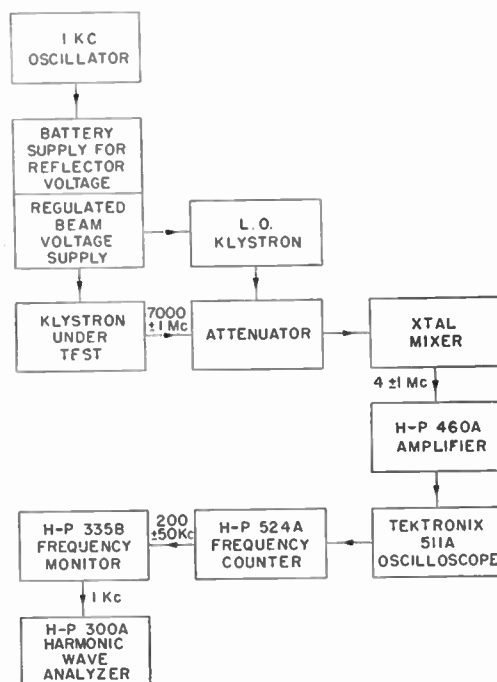
Fig. 5—Experimental setup used for measuring FM distortion.
