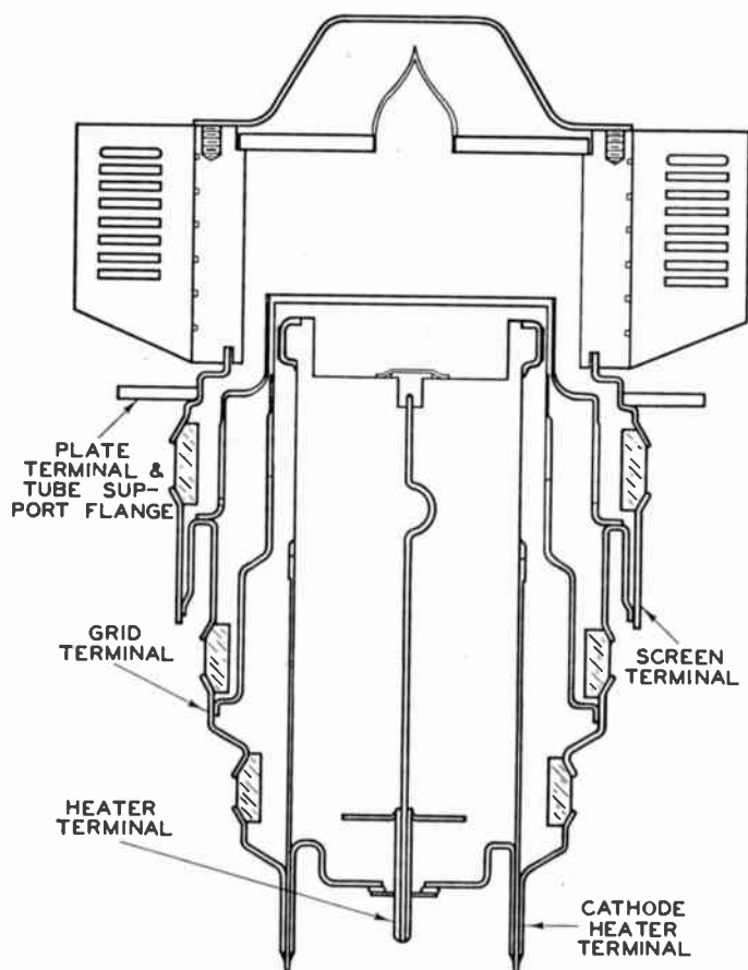
Fig. 2—Cross section of uhf power tetrode type 6181.
