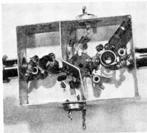
Fig. 6—900-mc chassis using lumped constants.
