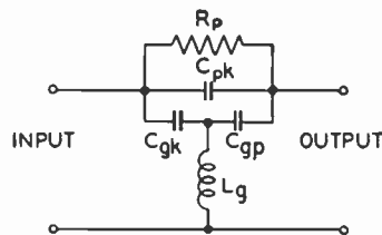
Fig. 1—The approximate equivalent circuit responsible for coupling in a conventional triode used as a grounded-grid amplifier.
