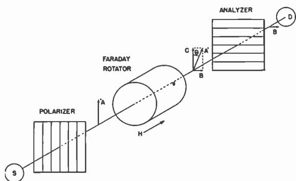
Fig. 1—Optical analogy of the microwave magnetometer.
