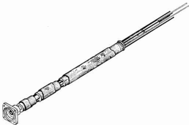
Fig. 1—Cutaway view of 7/8-inch coaxial-line termination.
