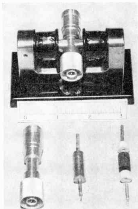
Fig. 4—Assembled magnetic attenuator using the small electromagnet and internal parts of the attenuator.
