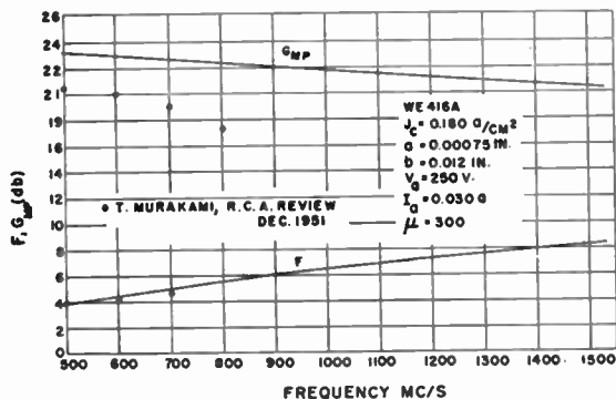
Fig. 11—Computed and measured performance of WE 416A triode.
