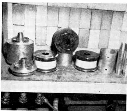
Fig. 7—Tube cavity parts and drift tube sections.
