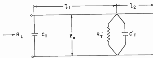
Fig. 6—Output matching circuit.
