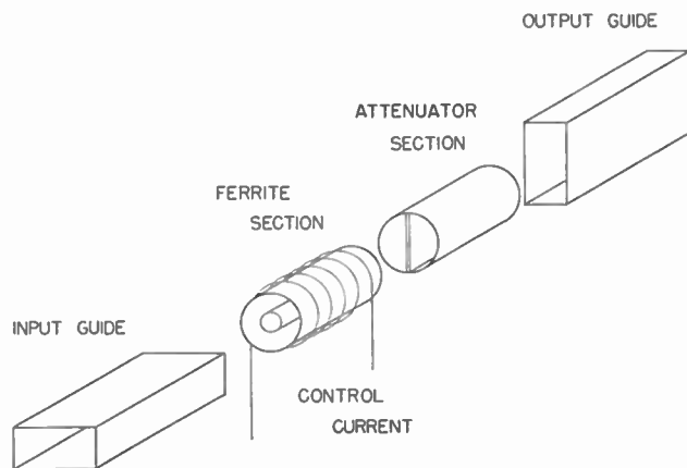
Fig. 2—Ferrite modulator unit.
