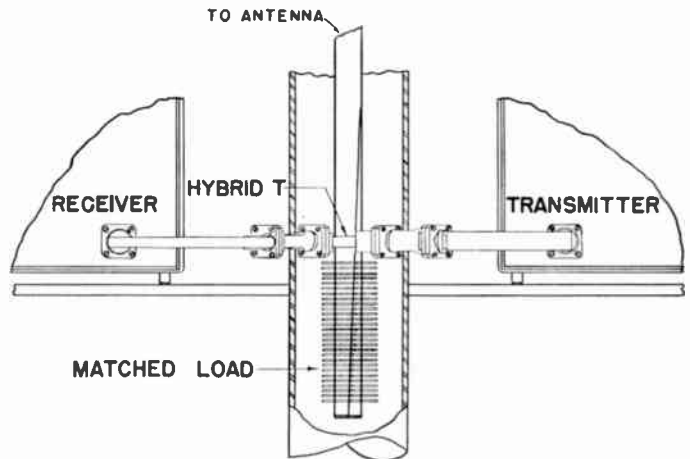
Fig. 1—Arrangement of the antenna duplexing T shown connected to the RF assemblies.
