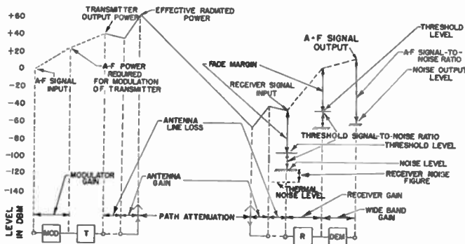
Fig. 10—One-hop system—level diagram.
