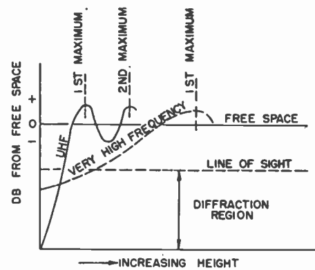
Fig. 1—Height-gain curves.
