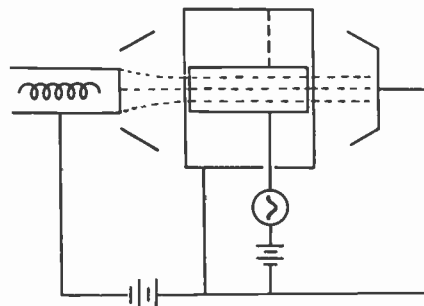
Fig. 1—Schematic diagram of floating-drift-tube klystron.
