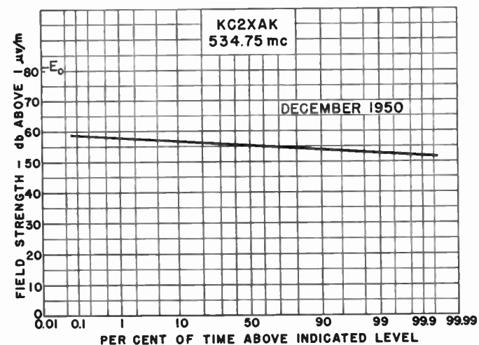
Fig. 4—Typical field-strength distribution for winter months.
