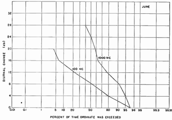
Fig. 3—Predicted frequency distribution of exceeded diurnal change in June.
