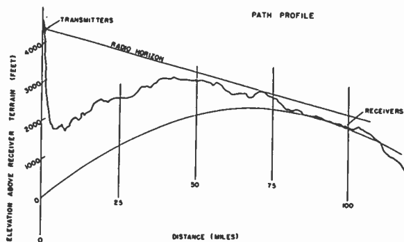
Fig. 1—Path profile for CRPL Cheyenne Mountain links.
