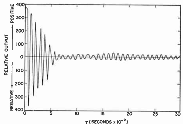
Fig. 6—Measured autocorrelation function.
