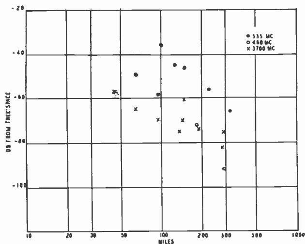
Fig. 2—Median signal levels measured at 460, 535, and 3,700 mc.
