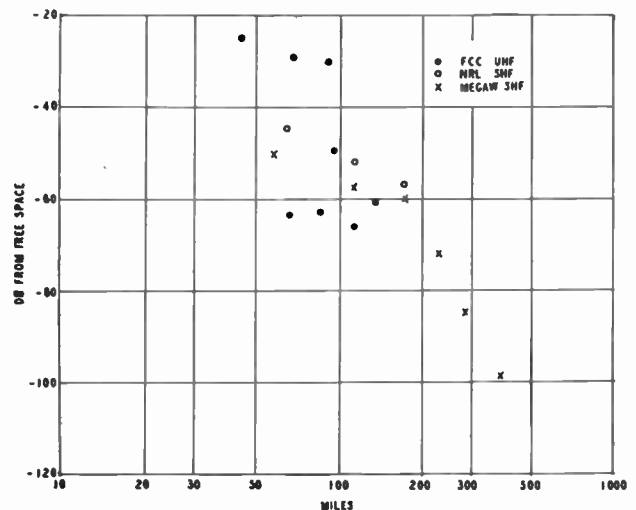
Fig. 3—Median signal levels at uhf and shf (from previously published material).
