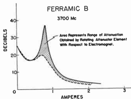
Fig. 9—Effect of rotating magnetic field of an attenuator operating near ferromagnetic resonance and using anisotropic dissipative material.
