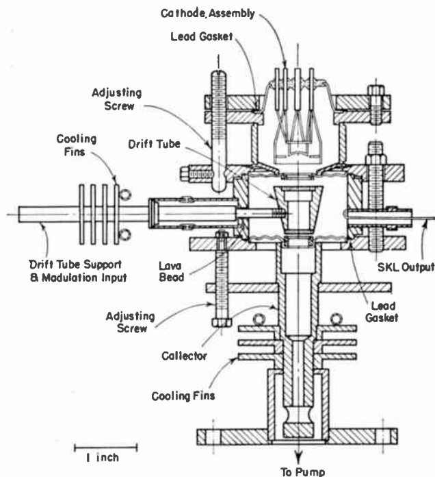
Fig. 4—Assembly of the experiment tube.
