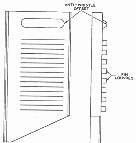
Fig. 7(a)—Radiator fin.
