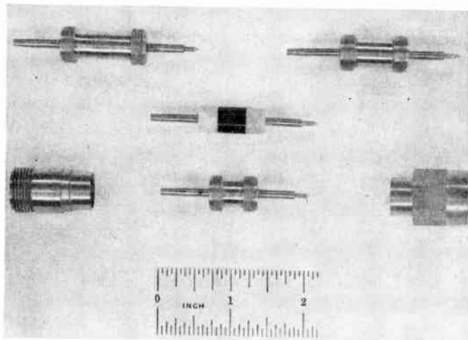
Fig. 2—Short section of transmission line showing the end connectors, the ferrite material, and three sizes of material housings for holding inserts of different lengths.
