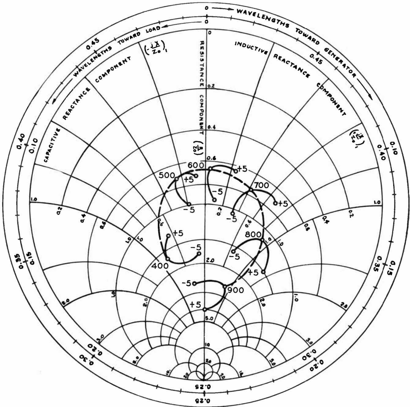
Fig. 7—Smith chart representation of the input impedance of a 6AJ4 grounded-grid amplifier circuit over the frequency range of 400–900 mc.
