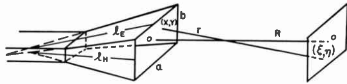
Fig. 3—Physical dimensions for calculating the gain.
