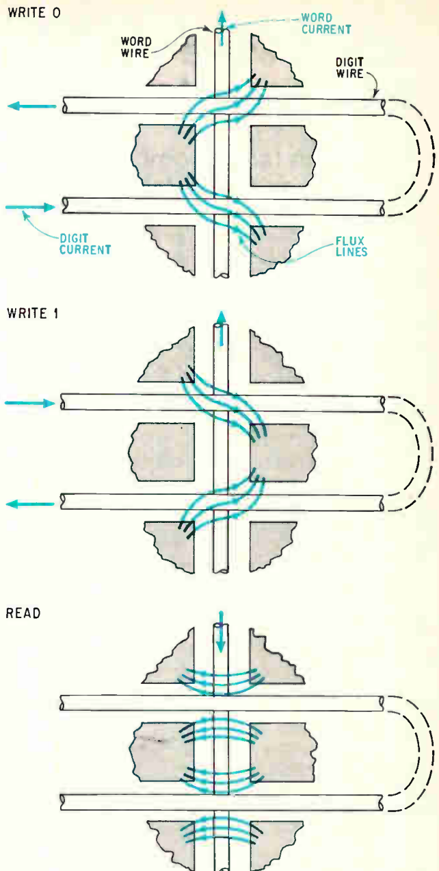
Catercorner. Flux paths in the thick film lie diagonally over the intersections of two grooves; two intersections store one bit.
