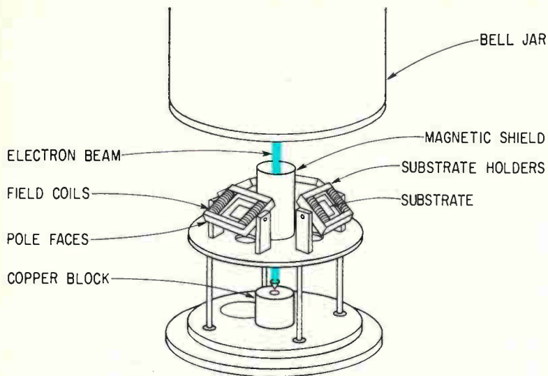
Evaporator. Electron beam (color) melts piece of permalloy on hearth; permalloy evaporates in vacuum, and vapor precipitates on relatively cool substrates.
