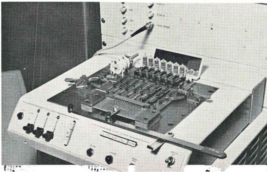
Counter clearance. Mounted in its adaptor is the main circuit board from a frequency counter. Even though the board contains a particularly complex array of circuitry, its test program took but a week to write. It runs in three minutes.
