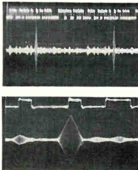
50-tap performance. First trace, the digital drive for the biphase modulator. The filter output with its sharp correlation peak is shown in the second trace after all 50 taps add in phase. Expanded in the last trace, this peak has a 200 nsec rise time.
