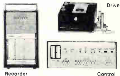
Clevite Surfanalyzer 150 Surface Measurement System
