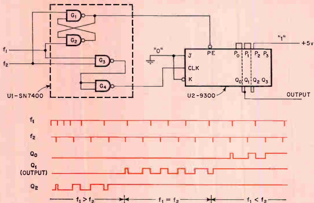
Right shift. The middle-bit position, P 1 , of the shift register will alternate between logical 1's and 0's when the two input signals, f 1 and f 2 , are equal in frequency. The duty cycle will be proportional to the phase difference between the incoming pulses.
