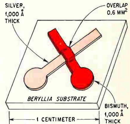
Slim. Bismuth-on-silver-on-beryllia thermocouple has 30 nsec response time for measuring fast-pulsed infrared laser.
