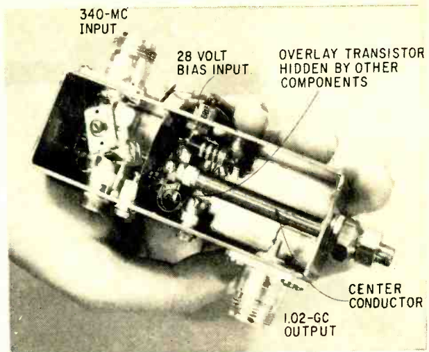
Combination amplifier-tripler uses one overlay transistor as both amplifier and frequency multiplier. The unit measures approximately 4 by 1¼ by 1¼ inches.
