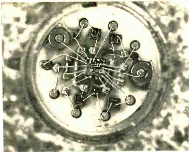
These two hybrid integrated circuits illustrate the partial integration concept. For example, the use of one multipurpose chip in the round package makes possible the housing of all the components in a Jecdec TO-5 package.
