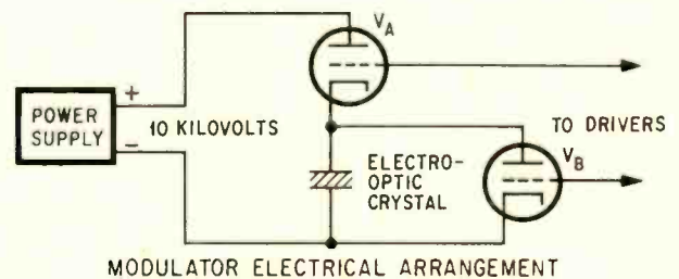
Electro-optic light modulator circuit. The high-voltage power supply is required to supply the electric field for the electro-optic crystal. Switching tubes V_A and V_B charge and discharge the crystal voltage.
