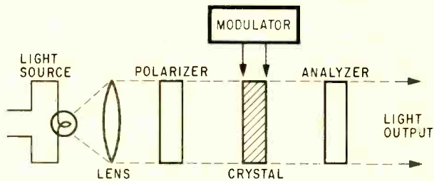
Optical arrangement shows position of the electro-optic crystal relative to the light source and modulator.
