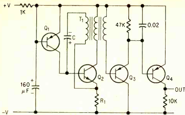
Early body-fluid pacemaker used rectifying action of base-emitter junction of transistor Q_2 to enable oscillations from ringing-choke oscillator to charge C_1 . Voltage on capacitor C_1 is raised by charging to a level that cuts Q_2 off. Then C_1 is discharged to create output pulse.
