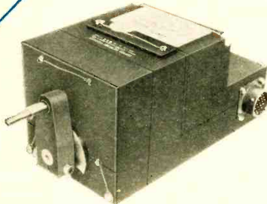
AUTOMATIC STABILIZATION ACTUATOR CH47A HELICOPTER (SEA KNIGHT)
