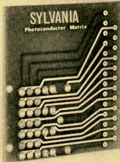
32-WAFER MATRIX
