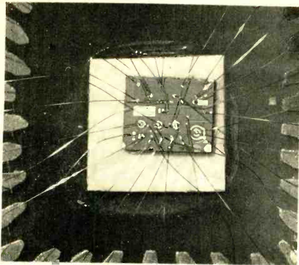
Mirt chip was the first general-purpose linear integrated circuit developed by Westinghouse. In 1961 it was used to build a prototype infrared search-track system and the IC is still being used.
