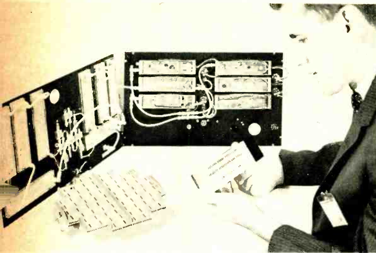
Doppler radar system , built for the Air Force, demonstrated that it was practical to mix Mirt and Lava chips in breadboarding prototype equipment. Breadboarded system is in background. Bill List holds actual-size model of final equipment.
