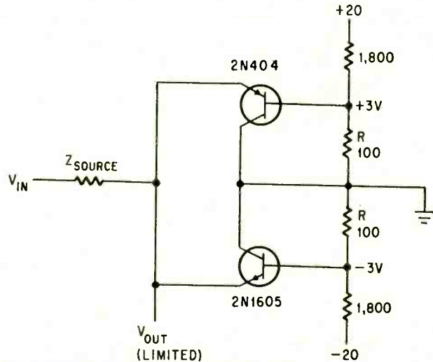
Transistor limiter uses minimal d-c power to establish reference voltages and simulates a diode with small internal d-c resistance.
