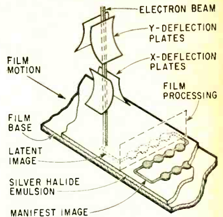
Basic elements of electron beam recorder
