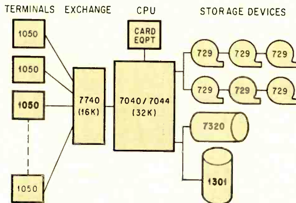
Equipment for remote-computing Quiktran system. Up to 50 remote terminals may be connected. Numbers in the blocks are IBM model numbers.
