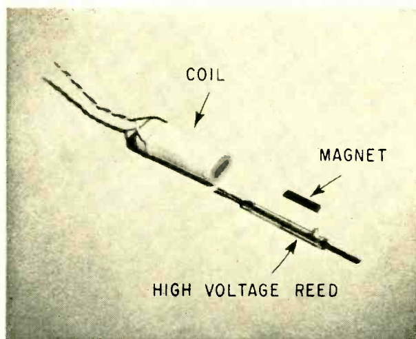
Components for the latching relay include a coil, a high-voltage reed and a small bar magnet. Reed should have a high pull-in to drop-out ratio.
