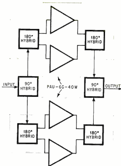
Twin boosters. The last stage has two 40-w modules coupled by hybrids.
