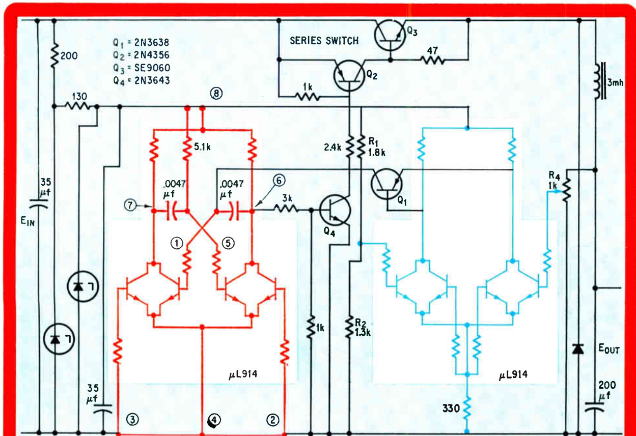
Versatility. With a few extra components, the uL 914 two-input dual AND gate can be converted into a differential amplifier and an astable multivibrator. Connecting the two makes a voltage regulator. The amplifier acts as an error detector, changing the duty cycle of the multivibrator.
