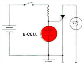
Basic-E-CELL Timing Circuit
