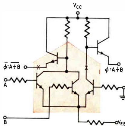
Linkable. Shaded area of one ECL gate can be connected to another to get wired-AND or wired-OR function.
