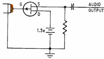
Less. Sony's electret capacitor mike, bottom, replaces conventional version in new portable tape recorder selling in Japan for $63. The simplified schematic shows how the electret model does away with preamplifier and power supply.
