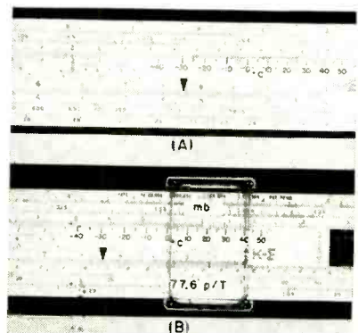
FIG. 1—Slide rules for the radio refractive index of air (A) for term 77.6 \frac{p}{T} and (B) for second term
