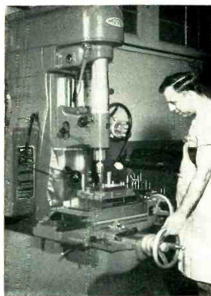
Use of new jig borer in Sylvania's Buffalo plant for drilling required holes in punching die for auto-radio switch contact
