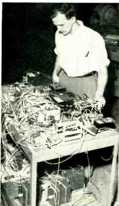
Appearance of breadboard setup for two-stage self-excited magnetic amplifier voltage regulator being designed for use in the atomic-powered submarine Nautilus
