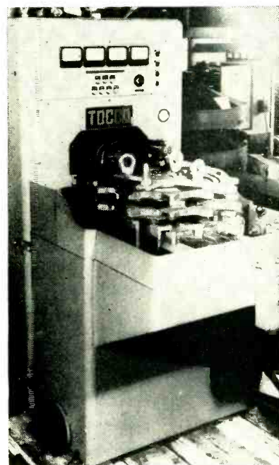
Example of induction heater using wire thread inserts in transformer panel face. Fixture in foreground is bolted to the generator and its inductor blocks are mounted securely on the transformer panel with cap screws that go into the insert-protected holes. The fixture serves to locate a sprocket during heating and hardening of its teeth
