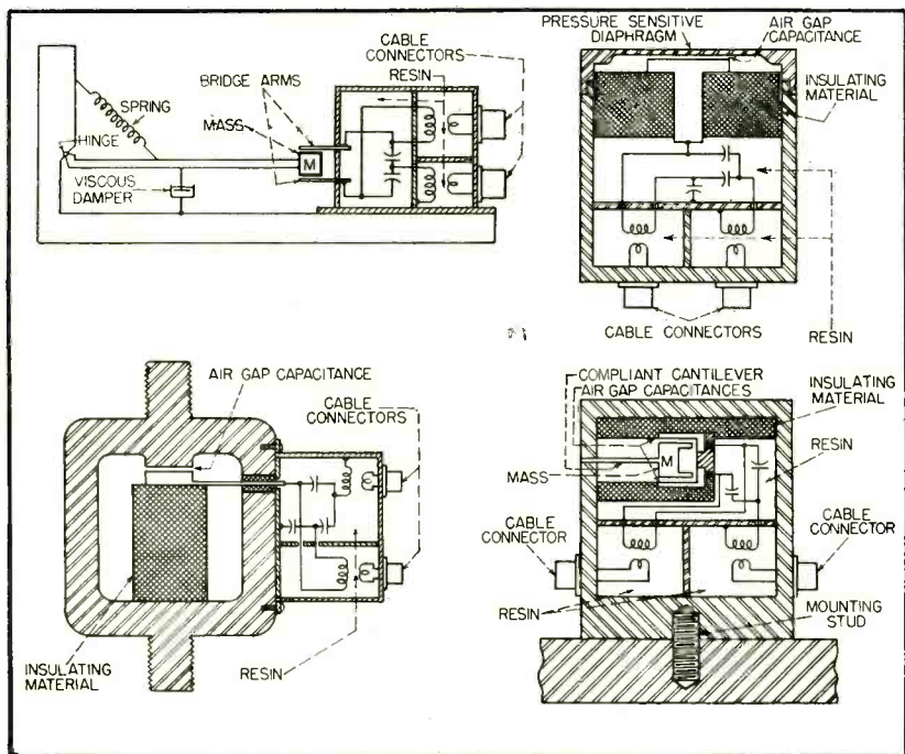
FIG. 5—Typical arrangements for measuring seismographic displacements, force, air pressure and acceleration
