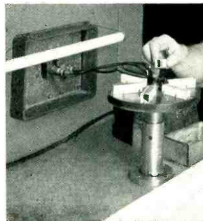
Six-position pedal-operated work table brings tin-plated steel housings under work coil for soldering of seams. Strips of precut solder are in wood box, and unsoldered housings are stacked neatly on table. Finished housings go into bin on floor at right of operator
