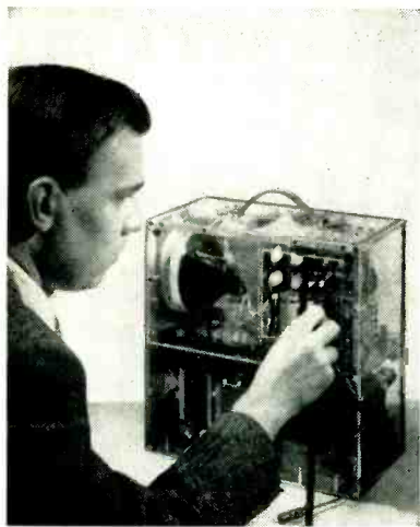
Thirty-six transistors perform all the functions in this 5-inch battery-powered tv set, except for c-r tube
