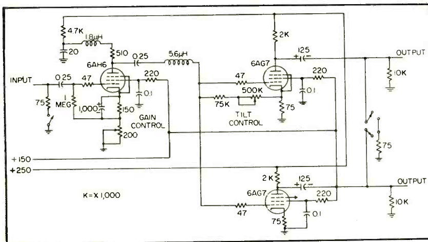
FIG. 2—One channel of two-channel distribution amplifier with frequency 3 db down at 10 mc. Output impedance is either 75 or 10,000 ohms. Tilt control maintains 60-cps square wave within \pm 2 percent
