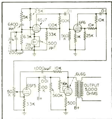
FIG. 1—Circuit of 5-kc RC oscillator
