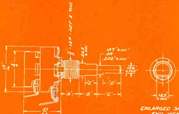
TYPE C45-70
