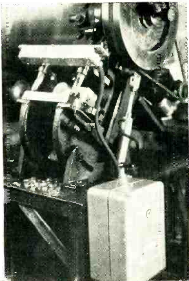
Radiation-type safety control installed on small motor-driven punch press
