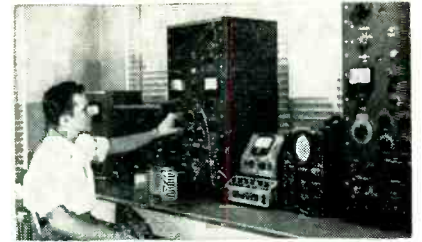
INDUCTANCE MEASUREMENT — Any operating condition can be simulated in the range of 0-100CV A.C. and 0-5 Amps. D.C.
