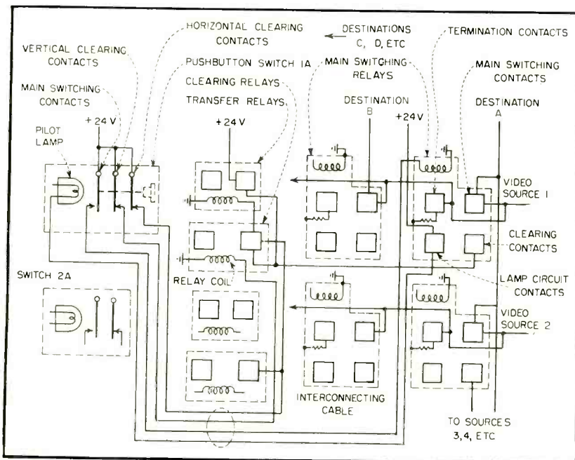
FIG. 1—Simplified block diagram of the switching action. Small squares are relay contacts, relay coils are shown as inductances and termination contacts are grounded through resistors
