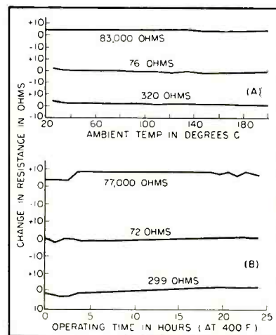
FIG. 1—Charts showing operating characteristics of carbon-film resistors
