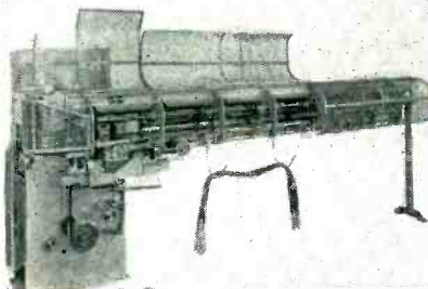
Special machine for automatically cutting and stripping leads up to 45 feet long
