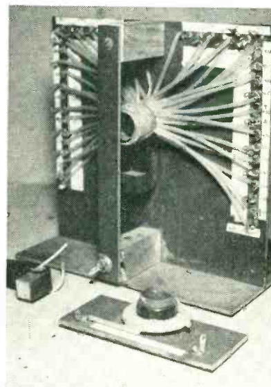
Rear view of early model of test transformer, with half of core removed. Core is replaced after swinging Bakelite locking strip out of way and placing secondary coil (in foreground) over other leg of mounted half of core. Each tap is labeled with number of turns from start of primary lettered on masking tape
