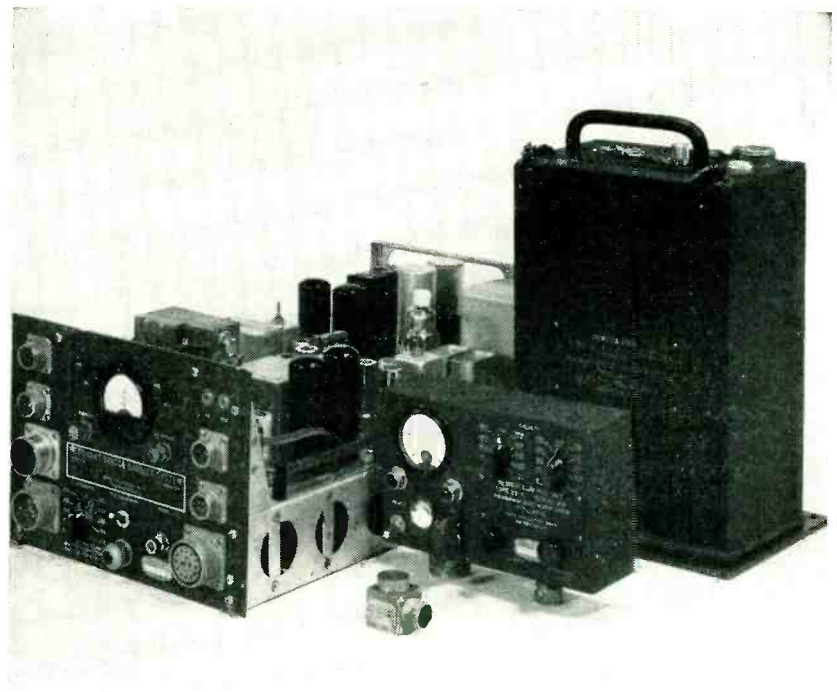
Complete system for measuring dynamic pressure under wing of aircraft in flight
