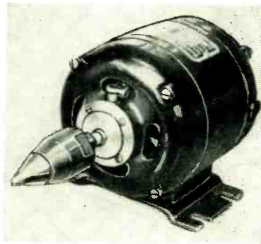
CASE HISTORY NO. 5 —Enamel-insulated telephone switchboard wires were to be stripped. The outer covering was removed with a hot-blade stripper, and the ends then inserted in the cone-shaped head of the above stripper to remove enamel. This machine is suitable only for AWG 20 to AWG 24
