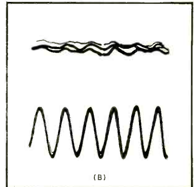
FIG. 2—Dual oscilloscope presentation with upper waveform showing longitudinal oscillation (A) at 300 cycles and diminished-amplitude waveform (B) with needle tied back. Improved lateral waveform (lower oscillogram) is apparent at (B)
