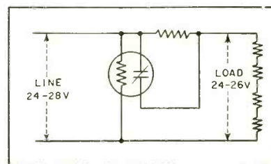
FIG. 1—Thermal-relay circuit for introducing a dropping resistor in series with vacuum-tube heaters when the supply voltage exceeds a certain value
