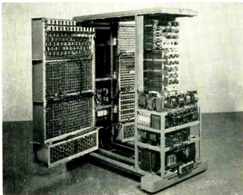
Highlight of the second annual joint AIEE-IRE-ACM Computer Conference held in New York, Dec. 10-12 was Eastman Kodak's multiple-stylus electronic printer, the electronic portion of which is shown above. Printing capacity is 400 characters per second. Machine is designed for printing magazine and mailing envelope labels, utility bills and insurance premium notices. Address labels can be turned out at six hundred per minute.
