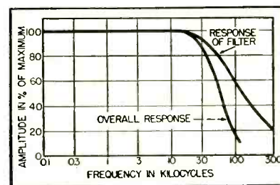
FIG. 2—Overall frequency-response of measurement system
