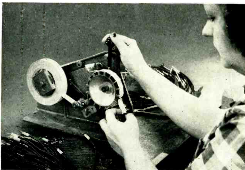
Automatic dispenser with side cover removed. Cutoff blade at top of spoked wheel is operated by hand lever simultaneously with tape feed mechanism. Slitter blades are under spoked wheel, behind thumb screw
