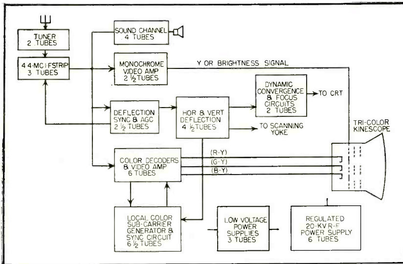
FIG. 1—Arrangement of stages in the overall receiver
