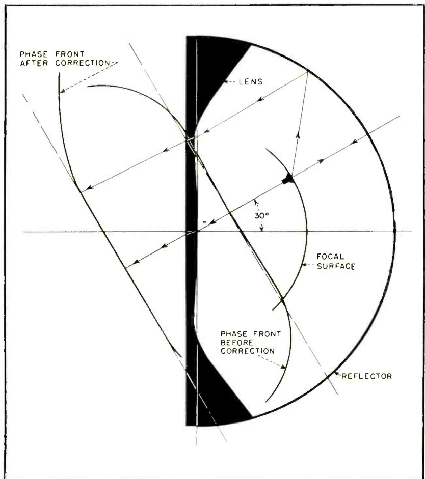
FIG. 6—Off-axis ray tracing shows that normal Schmidt lens overcorrects edges of wave front
