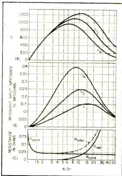
FIG. 2—Curves show resonant properties of two-wire line sections at 100 mc for 1/16-inch copper conductors
