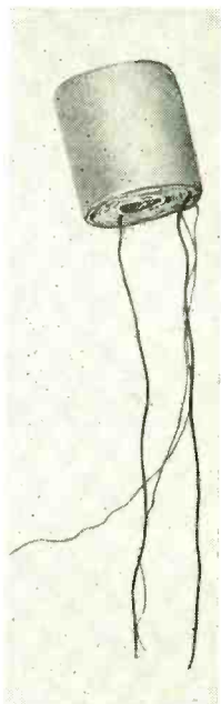
CASE HISTORY NO. 4 —Leads of a typical transformer coil (right) having two widely different gages of wire were to be stripped. Sizes were AWG 24 and AWG 36. A single machine has drawbacks; if the leads tangle, the small wire may be broken, and with the wheels set for the finer wire there will be excessive wire on the wheels and high wheel cost. The answer is the twin-headed stripper shown above, having one pair of wheels for each wire. Machine can be set for any size wire
