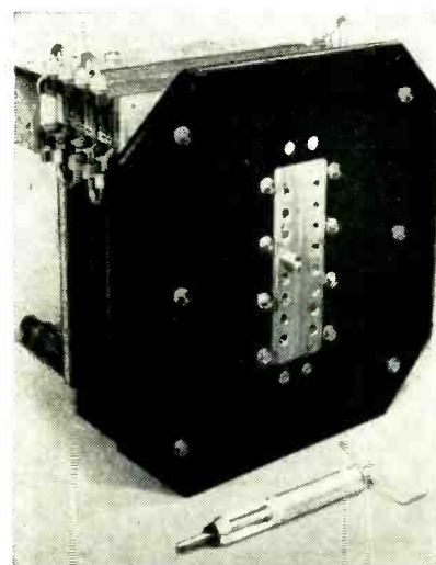
Outlet plate of induction heater transformer, with one insert partly installed and fifteen others already in the threaded holes. Wire-inserting tool is shown below
