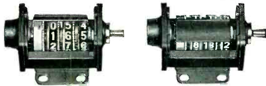
Companion shutter counters used as dual direction indicators. One counter adds while the other subtracts. Shutter blanks out counter which is on negative side of 000.
