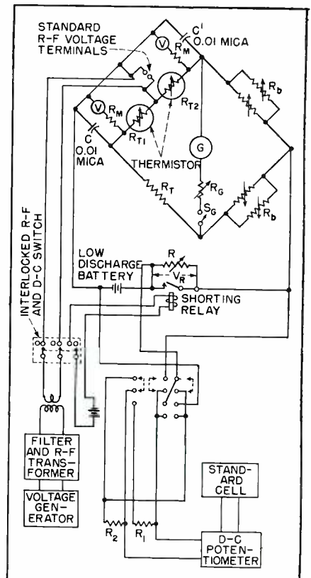
Circuit of new holometer bridge arrangement used in primary high-frequency voltage standard developed at National Bureau of Standards to provide accuracy comparable to that of standard d-c voltage cell
