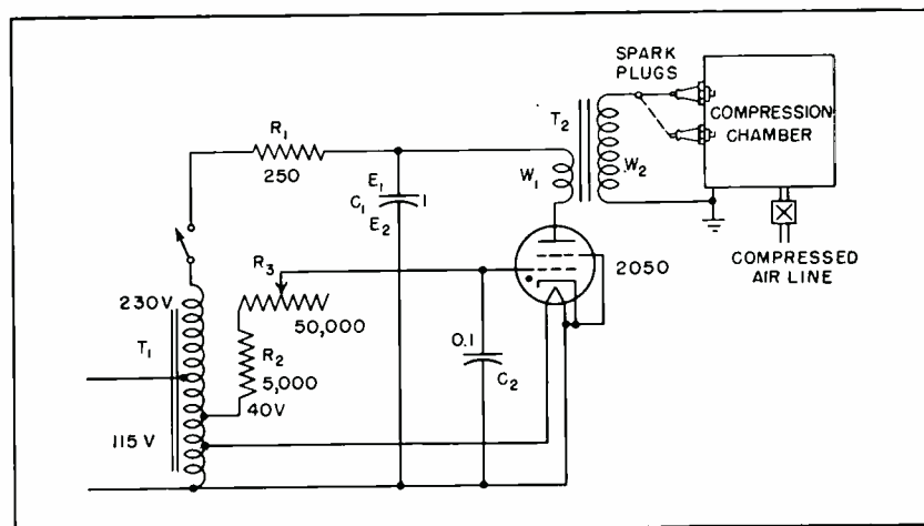
FIG. 1—Complete circuit of the electronic spark-plug tester
