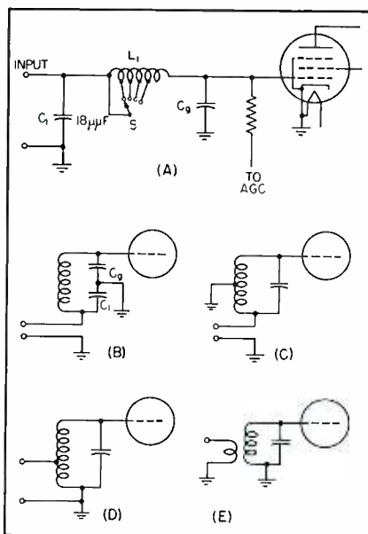
FIG. 9—Various conformations yielding essentially the same type of grid circuit used in the r-f stage
