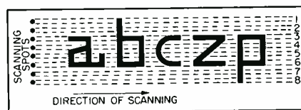
FIG. 1—Eight scanning spots are used in the letter reader
