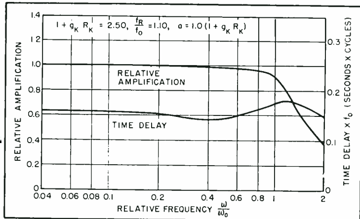
FIG. 4—Amplification and time delay characteristics for circuit constants and conditions of Fig. 3
