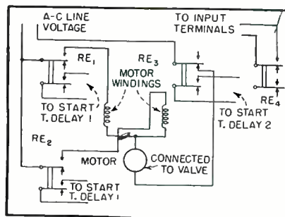
FIG. 4—Connections used for inching pressure control
