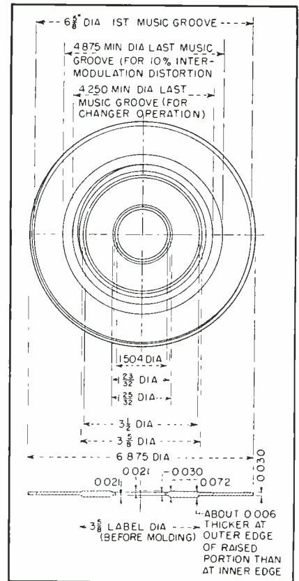
Dimensions and contours of the seven-inch record
