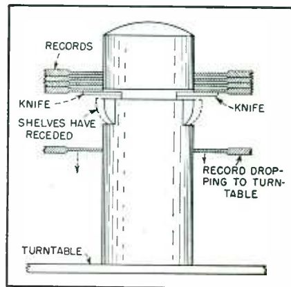
Eccentric-operated knife and shelf combination forms simple but speedy record-changer action on the 45-rpm unit
