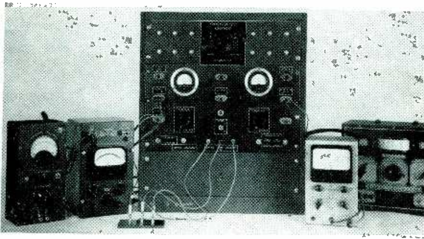
Complete equipment for testing transistors. Left to right: Electronic a-c voltmeter; vtvm for d-c emitter voltage; test unit, with transistor on three-terminal panel in foreground; vtvm for d-c collector voltage; audio signal generator. Jacks on test unit permit quick connection of additional precision meters and experimental connections to pentode grids
