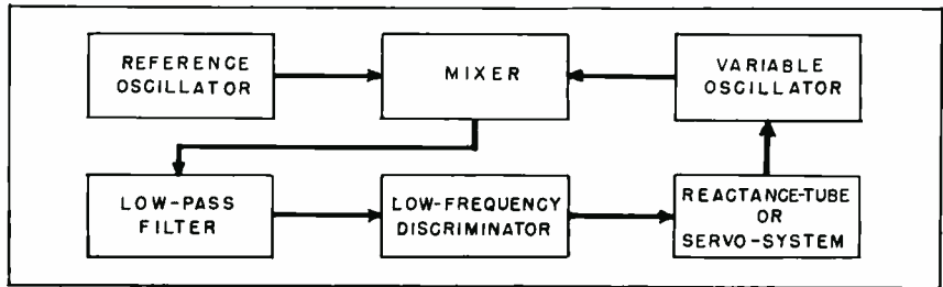
FIG. 4—To stabilize one r-f oscillator relative to the other, the low-frequency discriminator is used with a reactance tube or servo system
