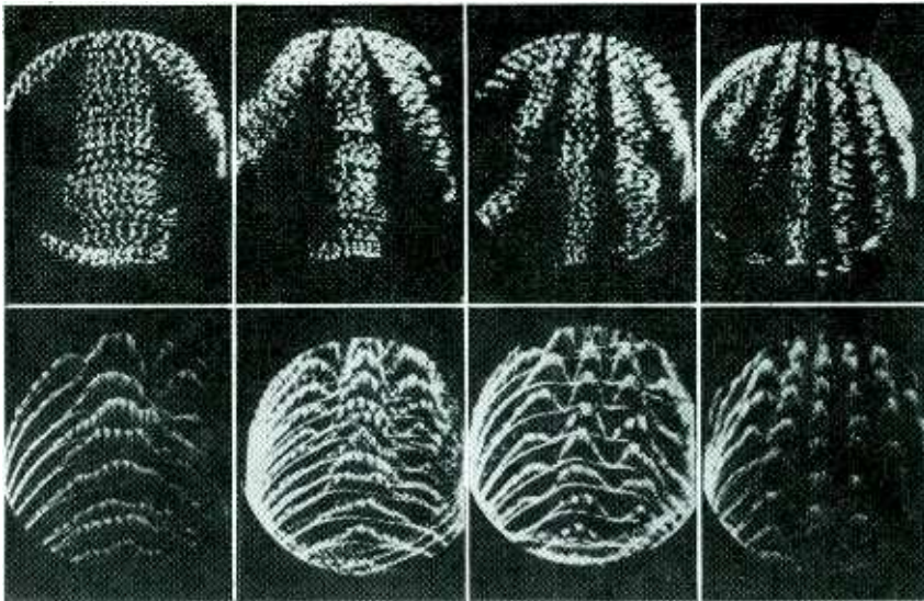
Oscilloscope patterns of wave interference in an electromagnetic field. Wavelength of both sources is 10 cm. Vertical columns from left to right are for distances of 1, 2, 3 and 5 wavelengths respectively between the interfering sources. University of Illinois photo
