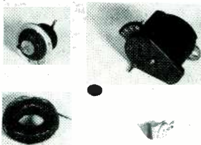
FIG. 3—Some measuring elements suitable for use with Flexi-Trol. They are toroidal coil, selsyn, induction generator and thermistor. Penny indicates relative sizes
