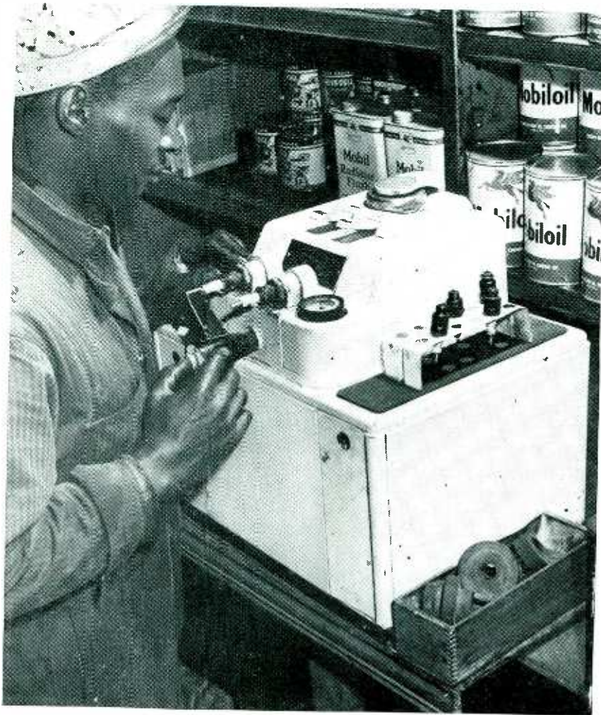
Typical spark-plug testing machine employing a compression chamber in which the plugs are fired
