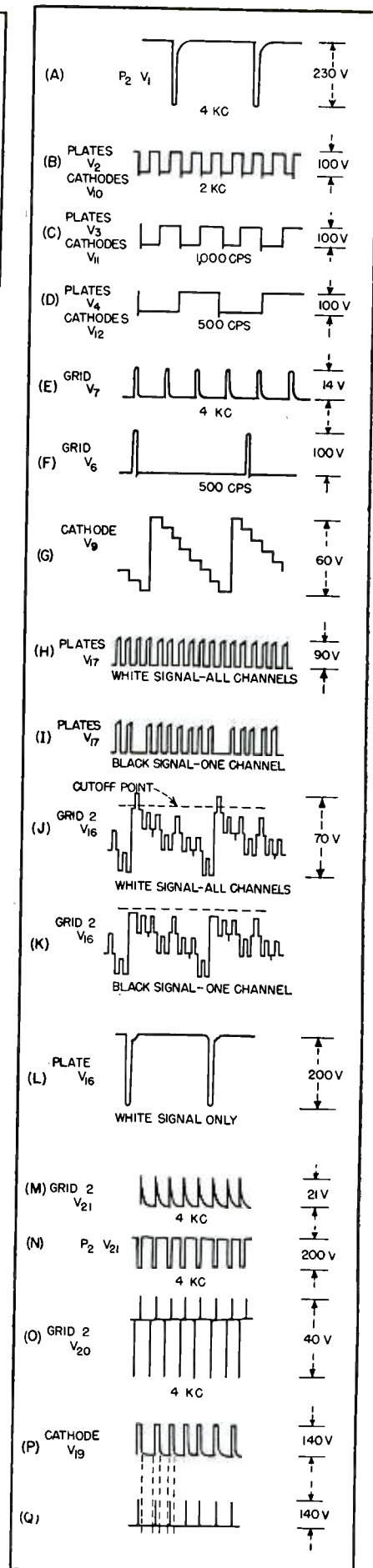
FIG. 7—Waveforms encountered in the reader circuits
