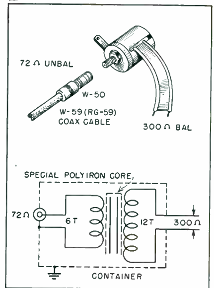
Matching transformer for television receiver antennas
