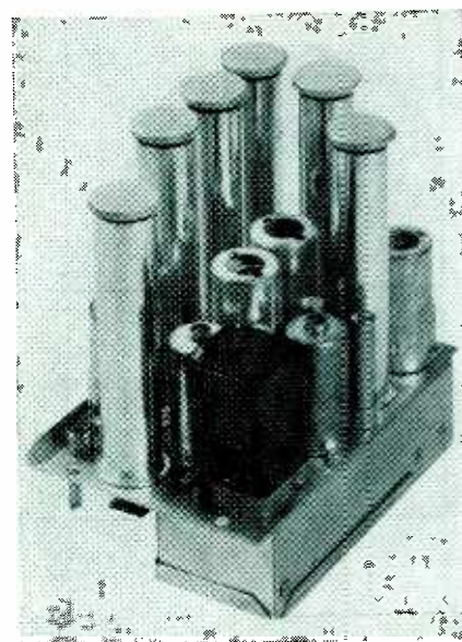
Closeup of receiver r-f deck. Crystal oven is in foreground
