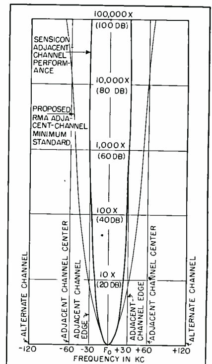
FIG. 2—Sensicon receiver selectivity curve
