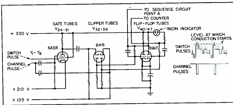
FIG. 8—Demodulator circuit, showing interaction of switch and channel pulses
