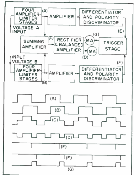
Waveshapes show operation of phase meter that gives unambiguous indication
