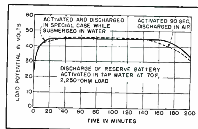
FIG. 2—Comparison of discharge of emergency battery in air and in special case
