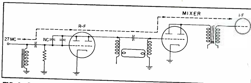
FIG. 2—Simplified circuit to show how diathermy signal passes circuit of Fig. 1 to show up as i-f interference
