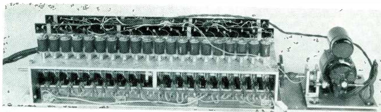
Letter-pronouncing section of the reader. The solenoids operate the magnetic tape recorders when tripped by the proper signals
