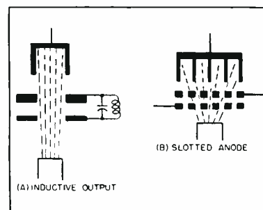
FIG. 1—Inductive output avoids effects of secondary emission. Slotted anode alone is unsatisfactory
