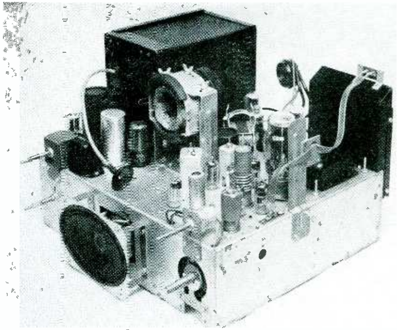
Chassis of the seven-inch table model receiver with picture tube removed
