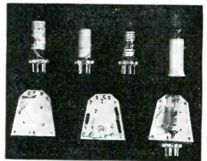
FIG. 1—Oscillator circuits of the two units at top left are printed on the outer surface of a steatite cylinder housing the subminiature tube. Next is a 6K4 with a painted circuit right on its glass envelope. Similar treatment was given the T-2 tube in the lipstick container at top right. Both sides of a steatite plate transmitter and the final assembly are shown at bottom. The silvered spirals form two chokes and the antenna coil
