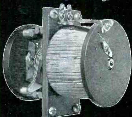
The 1-millihenry toroidially wound standard
