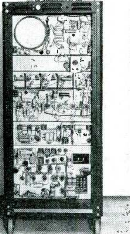
FIG. 1—Television camera and picture system chassis in a 4-foot rack
