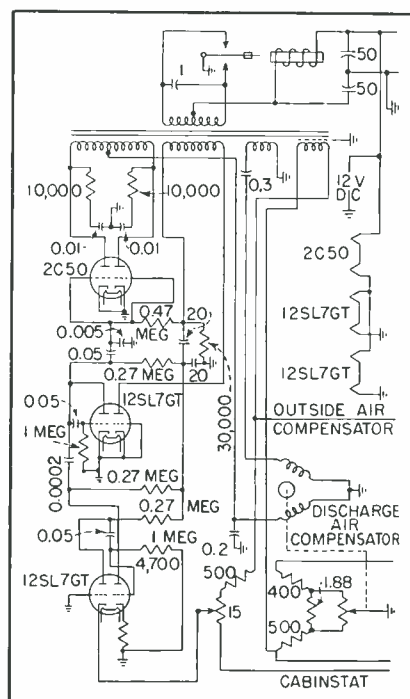
Complete circuit of cabin temperature controller operating from 12-volt vibrator-type power pack
