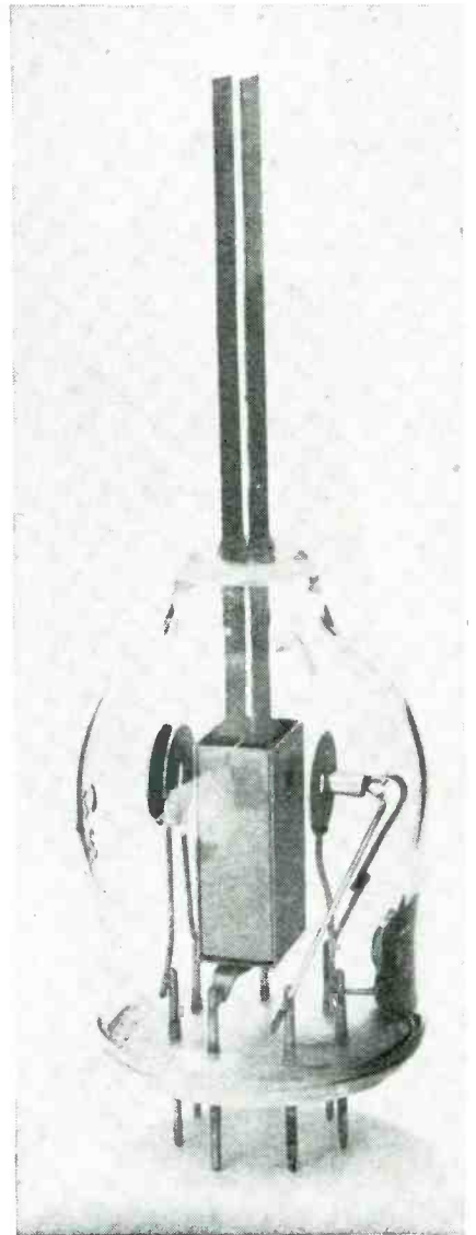
FIG. 2—Multireflection tube in glass envelope of 55 mm diameter produces 20 watts at 50 percent efficiency with magnetic focusing (not shown)
