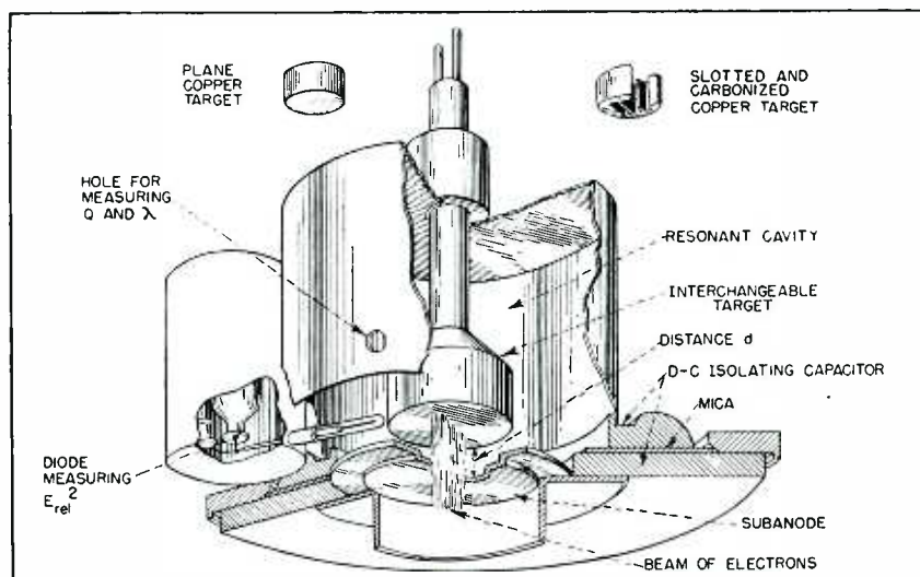
FIG. 2—Experimental setup used to demonstrate how power-output efficiency can be made nearly equal to theoretical maximum at microwavelengths by controlling transit angle, which essentially is ratio of transit time to time of one cycle of oscillation
