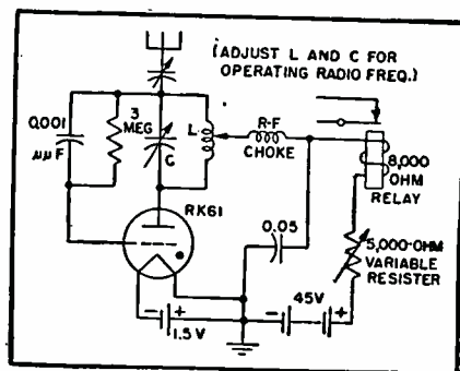
FIG. 1—Remotely controlled radio circuit uses subminiature tube
