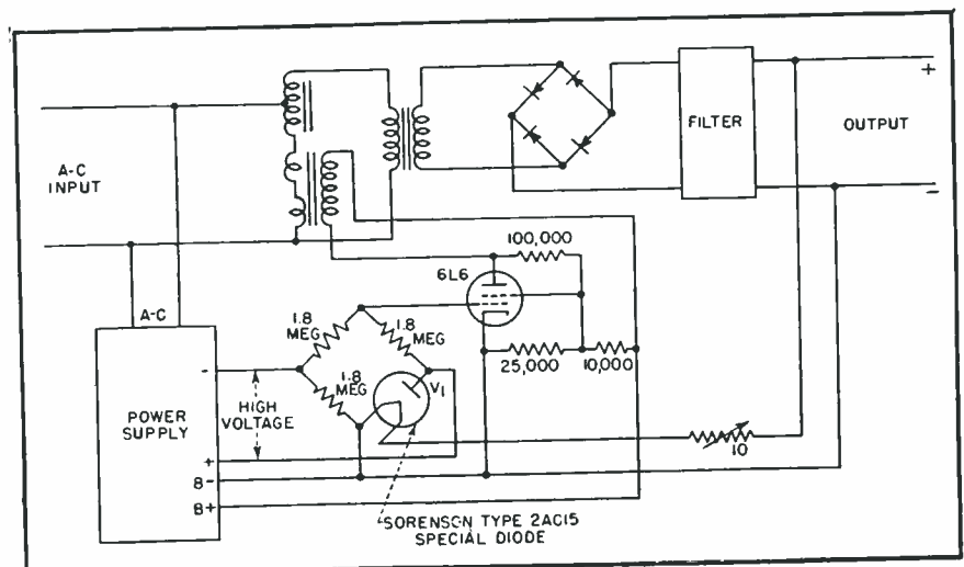
FIG. 4—Nobatron circuit, using dry-disk rectifier in conjunction with temperature-limited diode for regulating high values of direct current at low voltage
