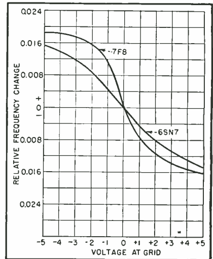
FIG. 4—Curves showing the variation of oscillator frequency as a function of control voltage
