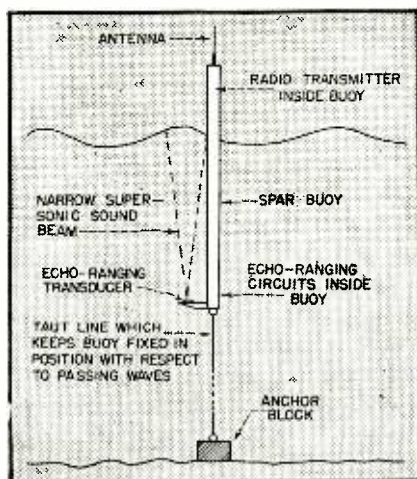
FIG. 6—Sketch illustrating principle of operation of a radio-equipped buoy which transmits wave data to a remote receiver-recorder. It was developed by the U. S. Navy Electronics Laboratory
