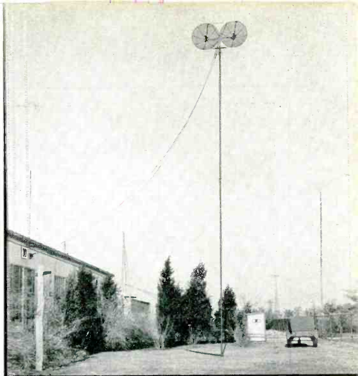
Antenna of the TRC-5 consists of two dipoles with parabolic reflectors atop a guyed fifty-foot pipe
