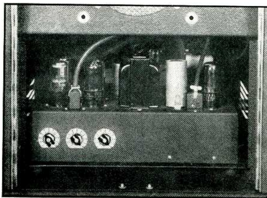
FIG. 2—Controls are set for desired recording characteristics when amplifier is installed. Plug connections facilitate servicing and replacement
