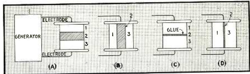
FIG. 2—Fundamental configurations involved in setting bonding glues
