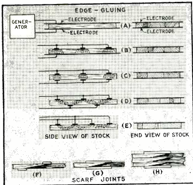
FIG. 5—Electrode arrangements for gluing core lumber
