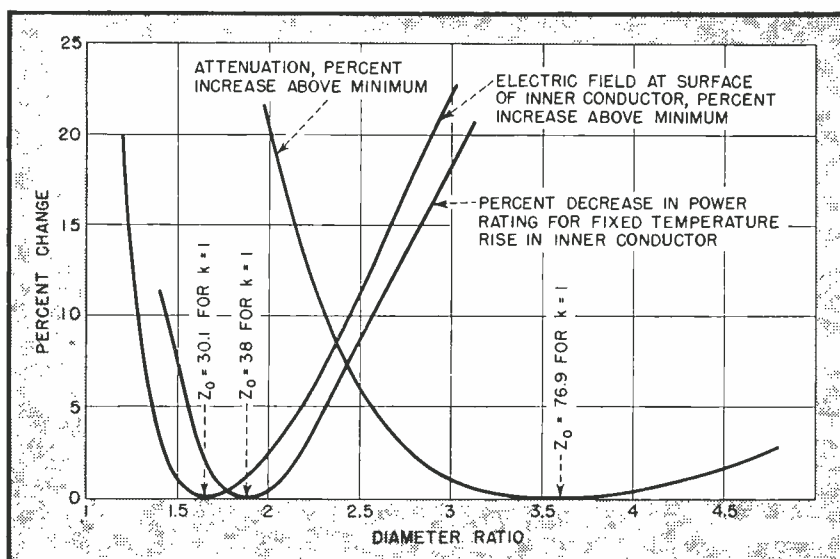
FIG. 1—Effect of diameter ratio b/a (which determines characteristic impedance as set forth in Eq. 1) on attenuation and on power-handling capacity as limited by flash-over and by temperature rise. (Temperature-rise curve calculated from data compiled by H. P. Thomas of the General Electric Co.)
