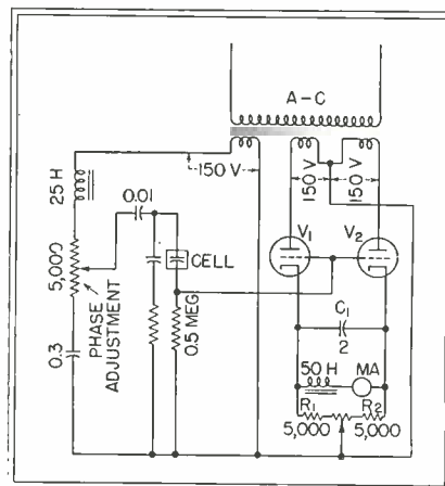
Fig. 1—Circuit for measuring small quantities of moisture in flaked and granular materials
