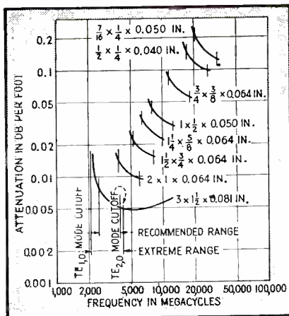
FIG. 4—Theoretical attenuation of copper wave guides over their operating frequency range for the dominant mode. Dimensions are outside measurements and wall thickness. Curves show the extreme ranges possible with each type of guide
