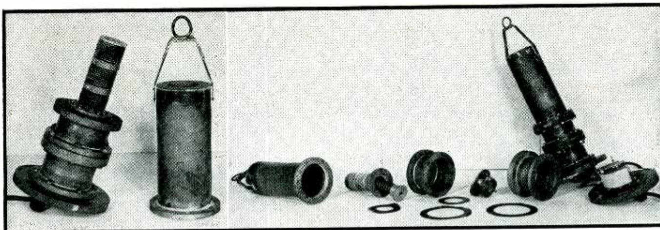
FIG. 3—Moving-coil type wave-pressure measuring unit developed by Woods Hole Oceanographic Institution, shown (left) with the cover removed, and disassembled, with the moving coil and magnet at the lower right
