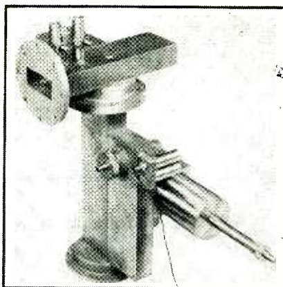
This wave-guide structure comprises a directional coupler, barretter mount, cavity wavemeter, magic tee, crystal mount, and tuning screws for impedance matching
