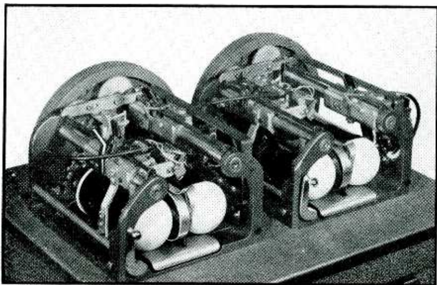
FIG. 5—Induction motors mounted underneath the unit plate drive the recording and reproducing carriages and the recording belt
