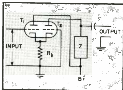
FIG. 1—Basic circuit of the oscillator. Tube T_1 operates as a cathode follower to drive T_2 .
