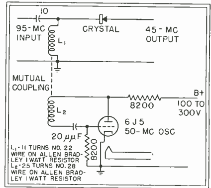
Circuit of a converter for f-m using a crystal detector as the mixer
