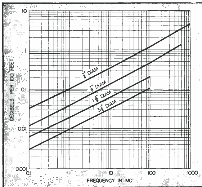
FIG. 5—Standard attenuation curves for nominal 70-ohm beaded coaxial cables used in broadcast-band work
