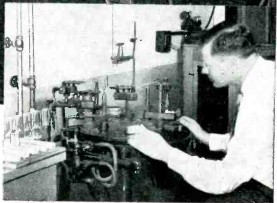
Sealing-in Machine in the process of sealing experimental electronic tubes preparatory to emission testing.
