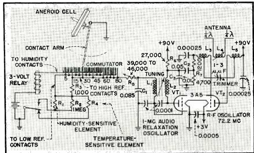
FIG. 1—Complete circuit (above) of radiosonde, including barometric switch. Interaction between the two triodes is such that when the 1-mc oscillator is on, the 72-mc oscillator is off, and vice-versa. The rate at which the 1-mc oscillator goes on and off is determined by the total resistance value shunted across C_1 .
