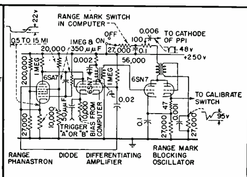
FIG. 5—Range phanatron circuit and succeeding stages in APS-15 system
