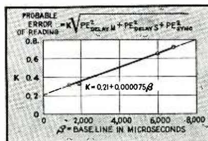
FIG. 14—The increasing value of the correlation factor, K , indicates that as the separation of transmitters increases, variations in delay tend to cancel less. This also shows that over great distances the ionosphere does not move uniformly
