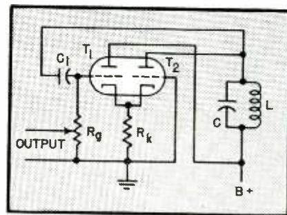
FIG. 3—Capacitor C_1 provides feedback to the grid of T_1 and also blocks the plate voltage
