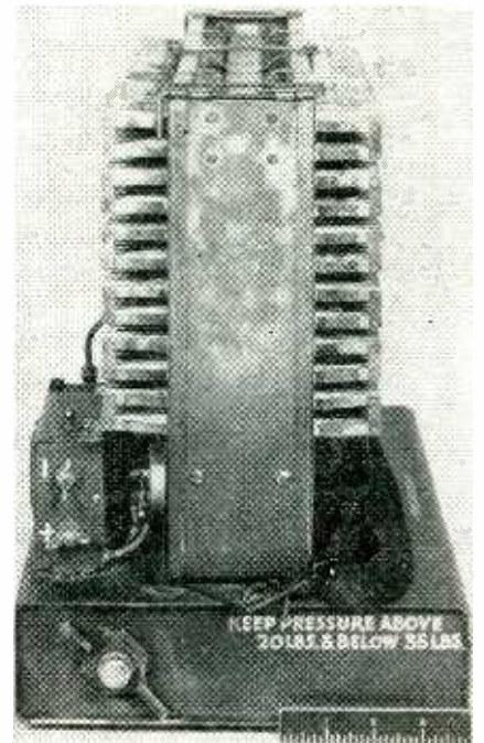
Side view of thermoelectric generator showing pressure-pump fuel cap and thermocouples in position
