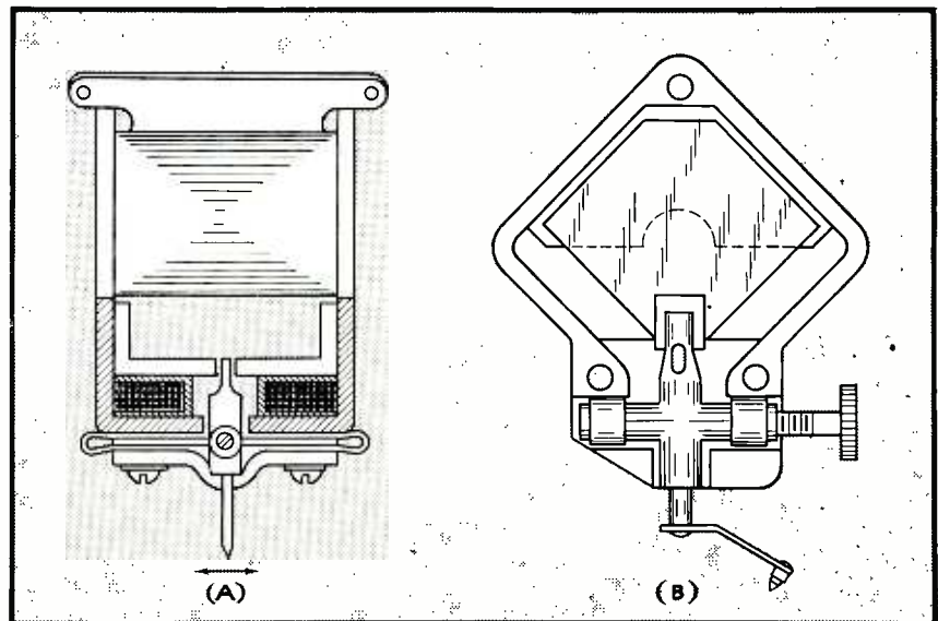
FIG. 4—Electromagnetic recorder head (A) and crystal reproducer (B) can be operating simultaneously on the flexible recording belt
