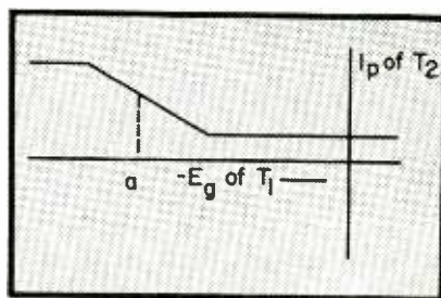
FIG. 2—Characteristics of the plate current of T_2 and the grid voltage of T_1 .
