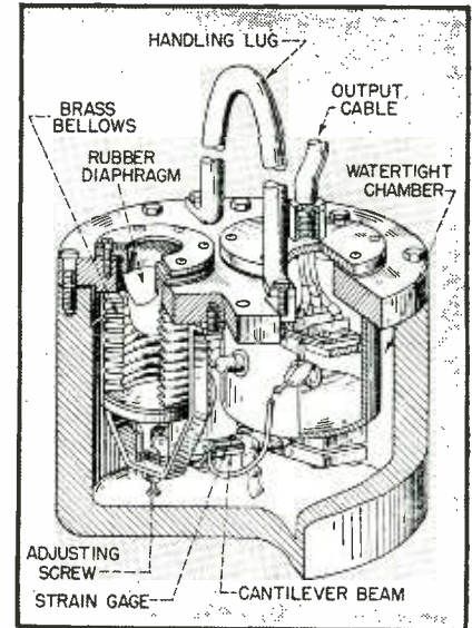
FIG. 2—Mechanical detail of strain-gage wave-recorder unit developed by the University of California. Water pressure acting via the diaphragm and bellows is recorded on shore through the three-wire cable. Wave heights are calculated from the resulting record of pressure on the sea bottom below the wave
