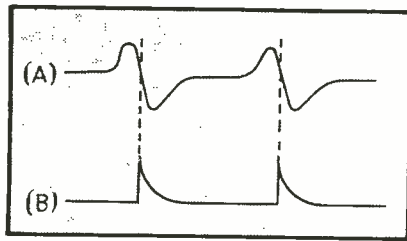
FIG. 1—(A) Pulses produced when a magnetized projectile passes through the two coils of a chronograph and (B) the same two pulses modified by wave-shaping networks
