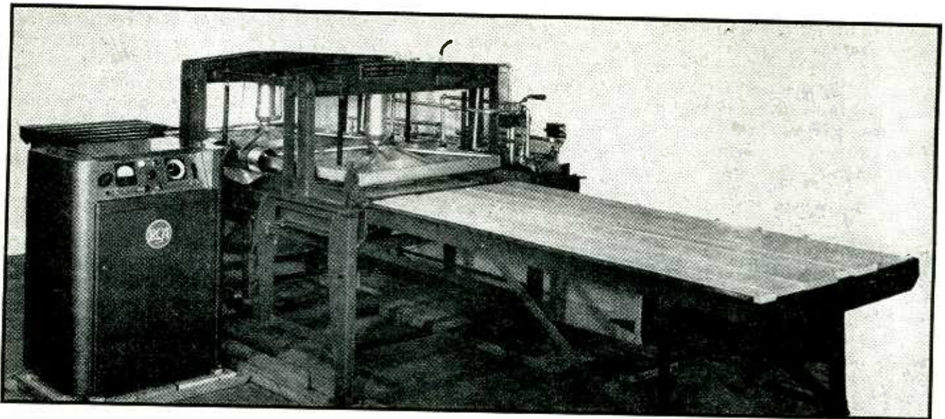
Edge-gluing press connected to 2-kw electronic generator for setting glue in core lumber to be used in veneered furniture
