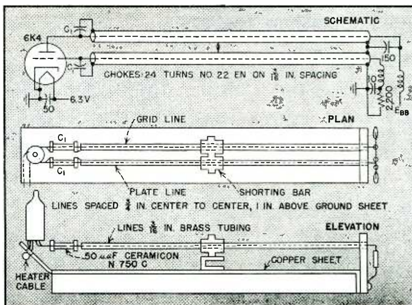
FIG. 6—Layout and circuit of line oscillator using small, baseless triode
