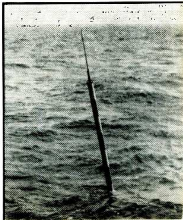
FIG. 7—Radio-buoy shown in Fig. 6 undergoing sea tests off San Diego. The receiver-recorder was in a plane several miles away
