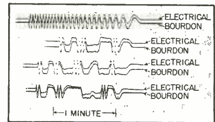
FIG. 5—Sample records of laboratory-generated waves, illustrating the ability of the electrical unit shown in Fig. 3 to reproduce complicated waveforms accurately by comparison with records obtained with a Bourdon gage and optical recording system
