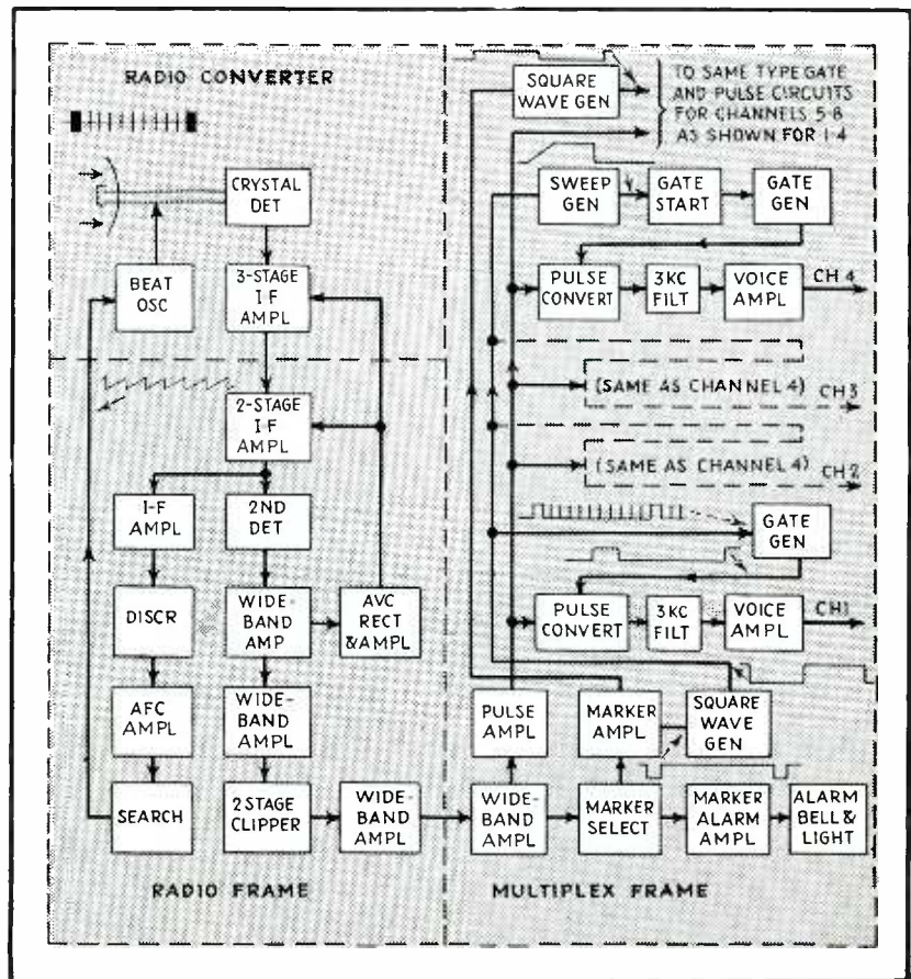
Components of the TRC-6 receiver
