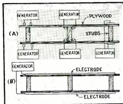
FIG. 7—Electrode arrangements for setting glue in production of prefabricated panels
