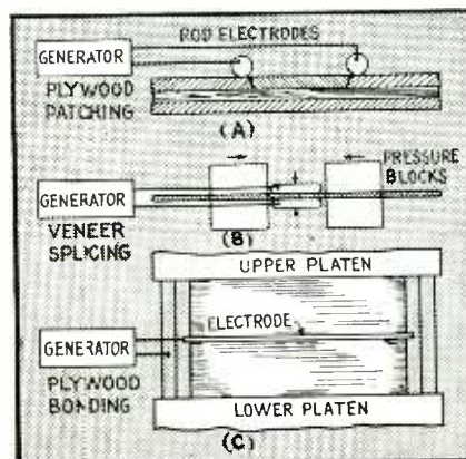
FIG. 8—Three successful applications of high-frequency heating to plywood and veneer pieces
