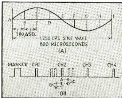
FIG. 2—(A) Signal is periodically sampled. (B) Instantaneous signal amplitude modulates pulses by displacing them about their normal position
