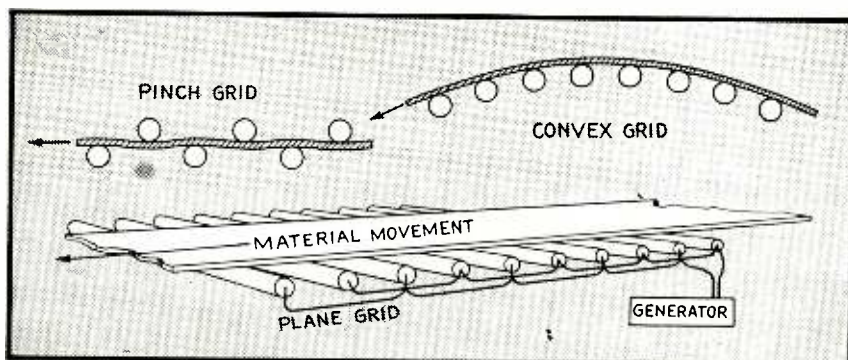
FIG. 4—Arrangement of grid electrodes for heating material from one side, and use of pinch grid for continuous heating of moving material
