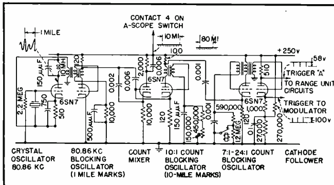
FIG. 4—Circuit of range unit that provides accurate timing pulses for the Philco APS-15 system
