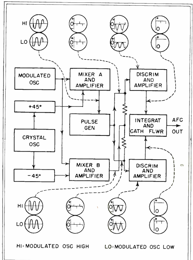
FIG. 2—Pulse counter stabilizes f-m oscillator
