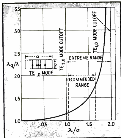
FIG. 3—Wavelength characteristics of a rectangular wave guide operating in the dominant mode. The ratio of wavelength in the guide to wavelength in space (ordinate) is plotted against the ratio of wavelength to the wider dimension (abscissa)
