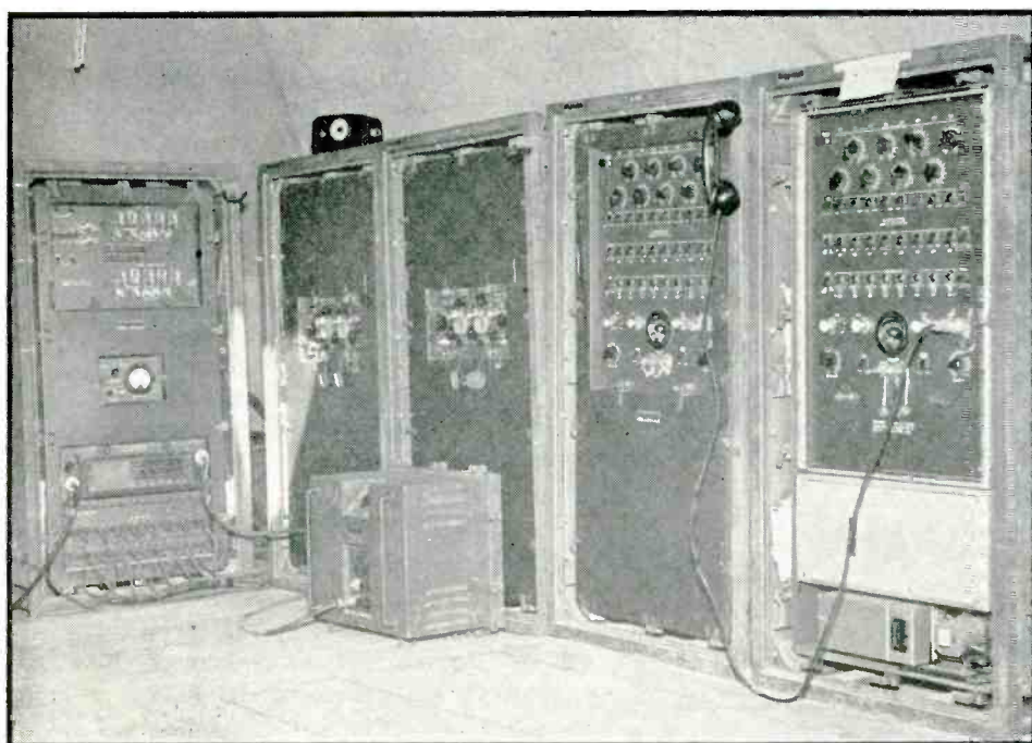
The TRC-6 consists, from left to right, of a common frame, spare radio, operating radio, multiplex frame, spare multiplex, and test oscilloscope
