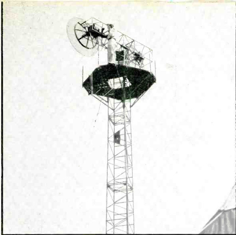
Transmitter and receiver of TRC-6 are mounted at antennas so that super high frequency circuits will be short
