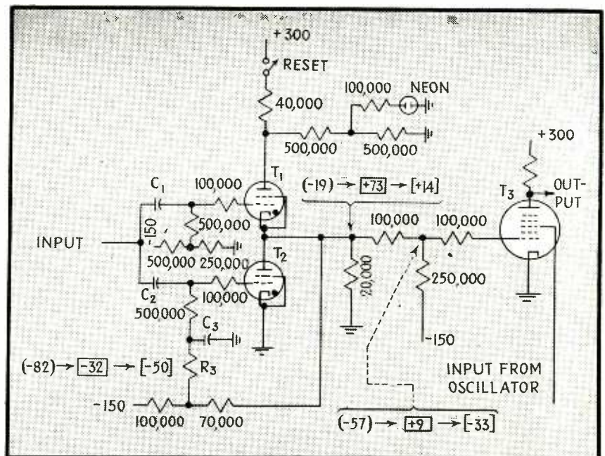
FIG. 3—The gate circuit discussed in the text, substituted for a more elaborate circuit originally employed in a typical chronograph
