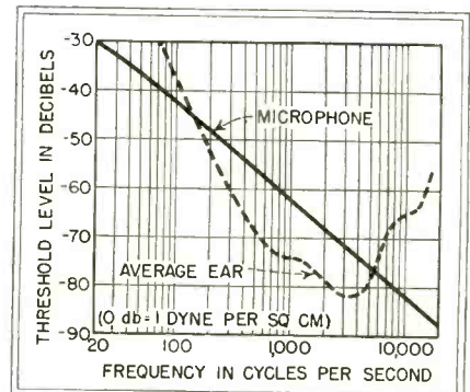
FIG. 3—Comparison of operating thresholds of microphone and of average ear
