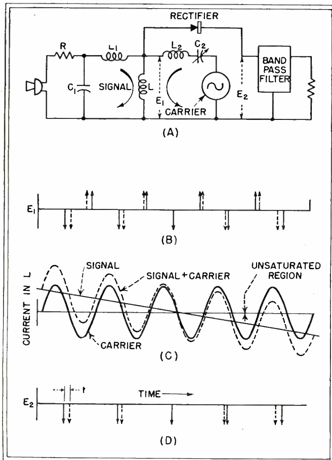
FIG. 1—Nonlinear inductor produces frequency modulation
