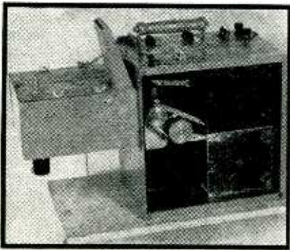
FIG. 4—Optical recorder for determining wave pressure, developed by Woods Hole Oceanographic Institution. The unit is self-contained and readily portable. It is used in connection with the moving-coil unit of Fig. 3
