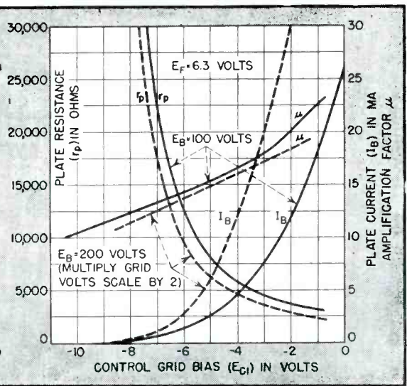
FIG. 3—Transfer characteristics
