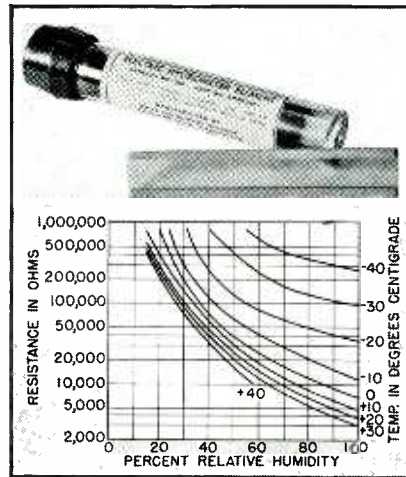
FIG. 4—Characteristics of electric hygrometer. The element is sealed in a glass vial for protection against dust, fumes, high humidity, and other deteriorating influences prior to use, and is removed from the vial and installed in the radiosonde at the time that the batteries are activated
