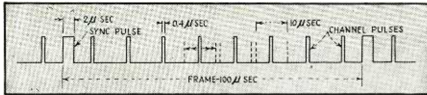
FIG. 1—Frame consists of a long synchronizing pulse followed by short channel pulses
