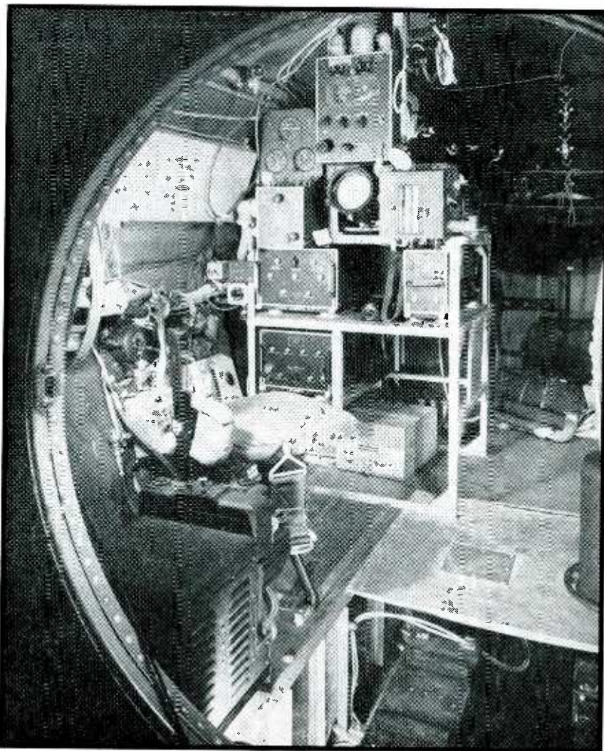
Radar operator's position at APQ-13 bombing radar installation in a B-29. Range unit is on lower deck of rack, while the synchronizer and a low-voltage power supply are on second deck. Antenna control-box is at left of c-r indicator and computer at right, with main control box directly above the c-r tube. Modulator is in lower left-hand corner of illustration, with an inverter unit visible below the floor
