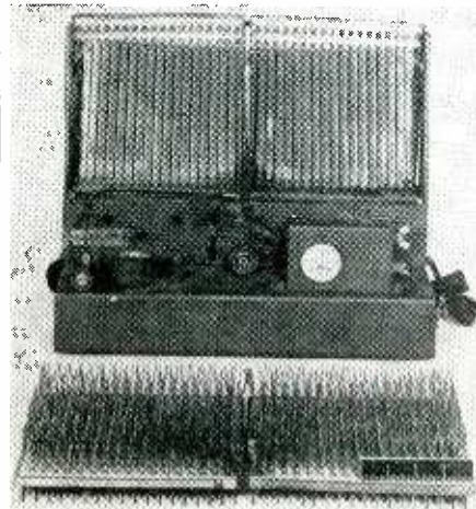
Twenty-watt thermoelectric generator with thermocouple unit removed to show assembly
