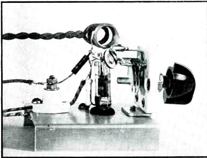
Full-size picture of the circuit diagrammed in Fig. 4 shows use of rubber grommet for shock mounting and compactness of circuit
