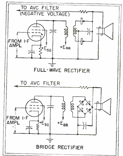
FIG. 2—Best results are obtained with a full-wave rectifier
