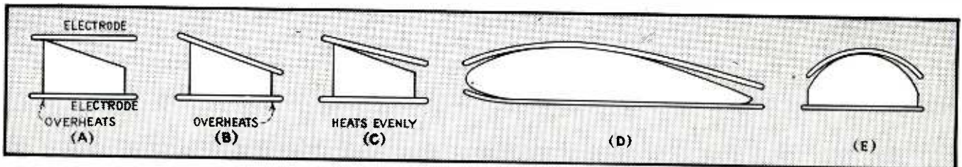
FIG. 3—Electrode contours for securing uniform heating of nonuniform thicknesses
