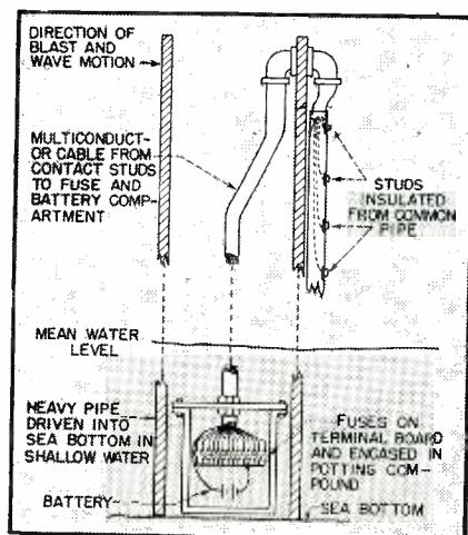
FIG. 8—Maximum water-height recorder which blows fuses corresponding to wave heights when water shorts the contacts. The blown fuses constitute a record which may be examined later, in the case of the Bikini Atoll atomic-bomb tests after danger of radioactivity subsides. A radio-controlled switch may be installed to place the recorder in operation when the tests are about to start
