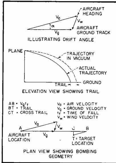
FIG. 3—Geometry of bombing problem
