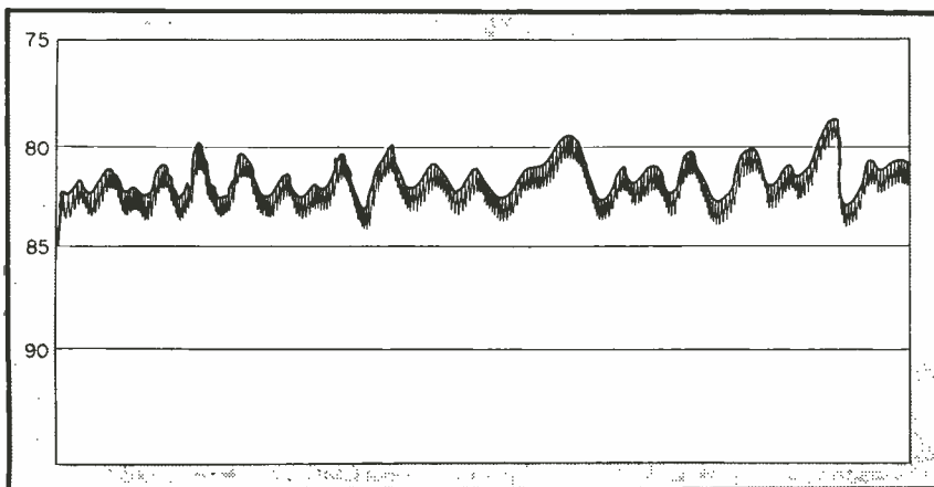
FIG. 1—Typical wave record from a recording echo-sounder installed on a ship at anchor in 82 feet of water. Waves are seen to be from 1 to 4 feet high
