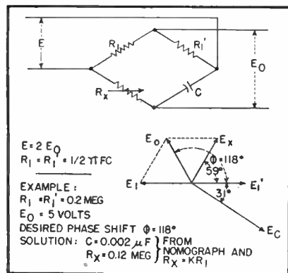
FIG. 1—Bridge-type phase-shifting network, and vector diagram for the example set forth
