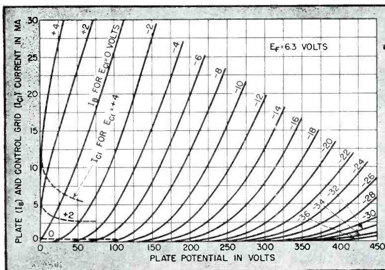
FIG. 2—Plate characteristics
