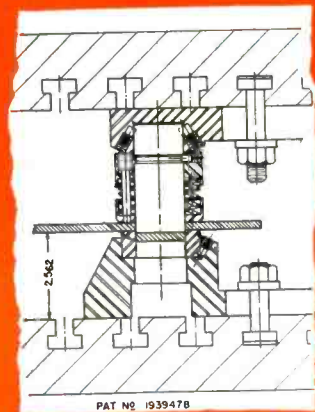
Sectional drawing illustrating simplicity of assembly of punch and die unit parts.
