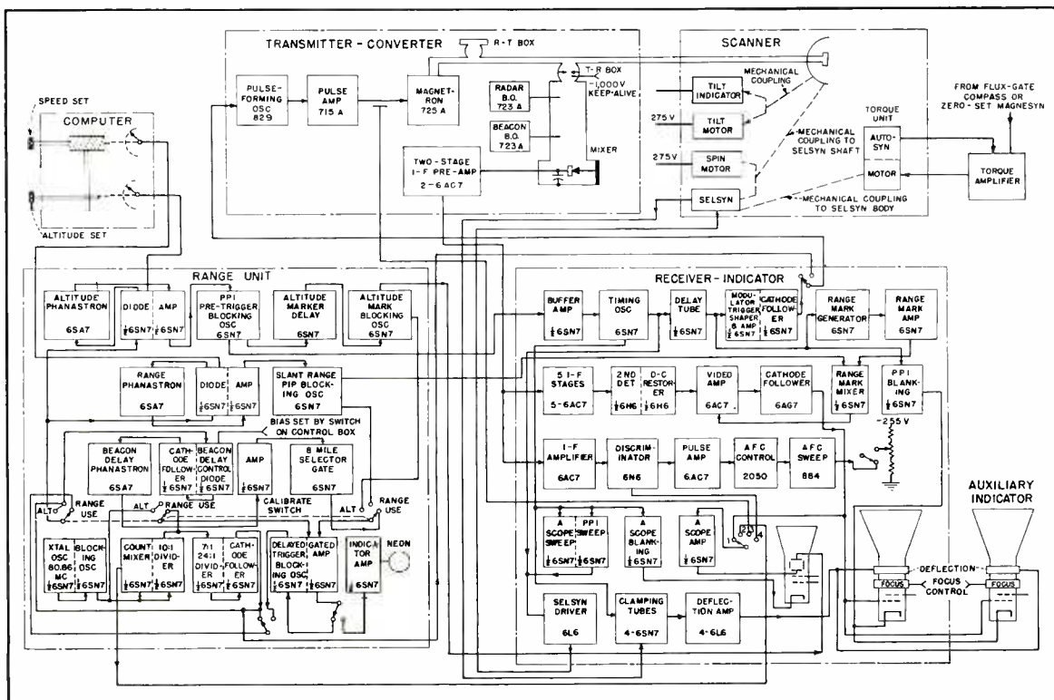
FIG. 2—Block diagram of Philco APS-15 version of H2X bombing radar
