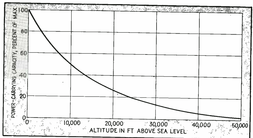
FIG. 5—Percentage decrease in the power-carrying capacity of a wave guide with increasing altitude (decreasing pressure)
