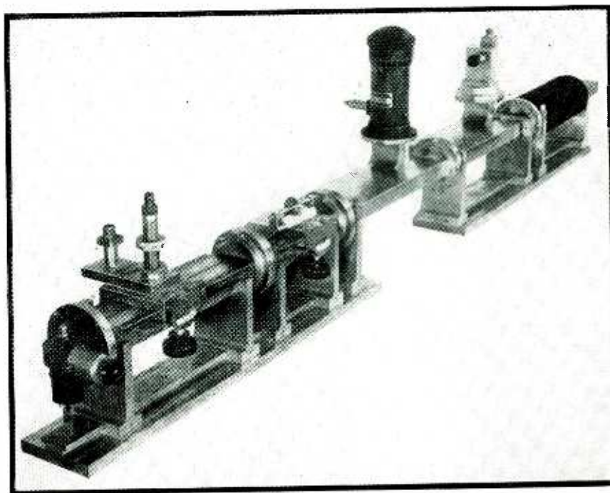
An assembly of wave-guide measuring instruments used to determine the effect of load impedance upon oscillator power and frequency. From left to right are: a reflex klystron, impedance meter, impedance transformer, directional coupler (with a cavity wavemeter this measures frequency) barretter mount for power measurement, and high-power matched load. All the rectangular guide shown is 2 \times 1 inch.
