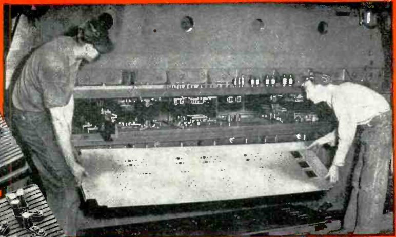
An example of piercing standard size holes, special shapes and corner notching with Whistler adjustable dies.
