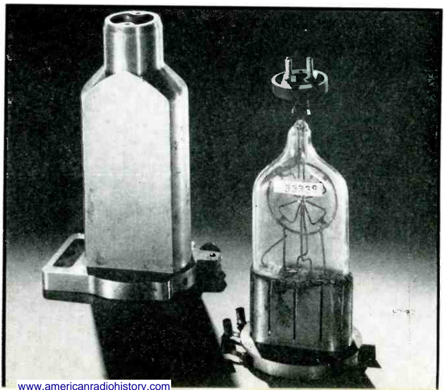
Type M-60 low-power 10-cm receiving magnetron and its cast housing that serves both for shielding and protection. This tube was used in conjunction with the type M-312 for Japanese naval search radar equipment
