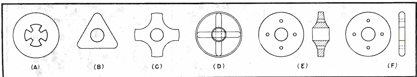
FIG. 4—Typical insulator shapes used in beaded coaxial transmission lines
