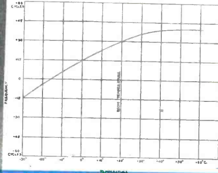
TYPICAL CRL — 30 FREQUENCY TEMPERATURE CURVE
