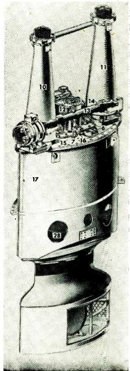
Sonar transducer mechanism in retracted position, showing 20-inch diameter disc that rotates in its streamlined dome. Motor turns gears which rotate lifting screws inside pillars 10 and 11 to raise or lower dome
