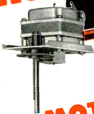
Model RR enclosed split-phase Reversible Motor. Alliance Motors are rated from less than 1-400th up to 1-20th H.P. With or without integral gears.
