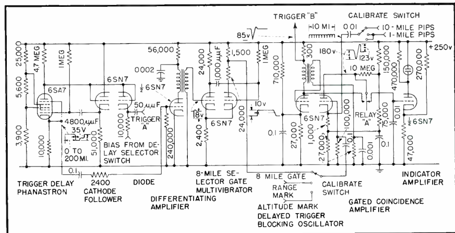
FIG. 7—Trigger-delay phanastron circuit and succeeding stages in APS-15 system, using a coincidence amplifier to increase the accuracy of long delays
