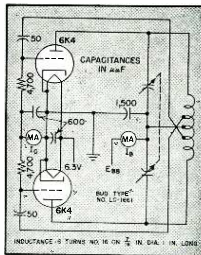
FIG. 6—Layout and circuit of line oscillator using small, baseless triode
