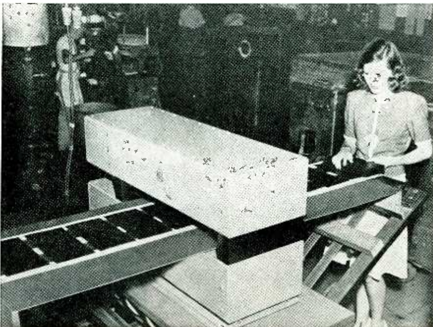
Plastic blanks are inspected for metal particles to prevent damage to dies used in pressing or molding. The blanks on the conveyor belt pass through an aperture where coils are embedded in surrounding panels
