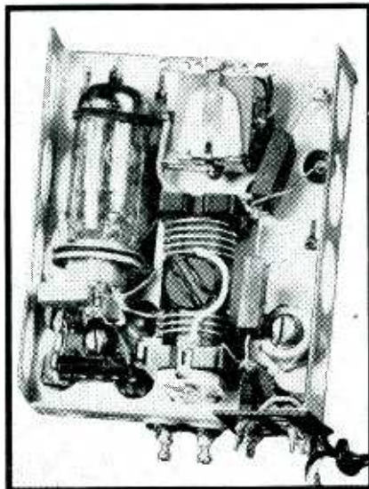
Chassis of radiosonde transmitter, showing 3A5 tube and 3-volt relay (at top), adjusting screws, and antenna terminals (at bottom)
