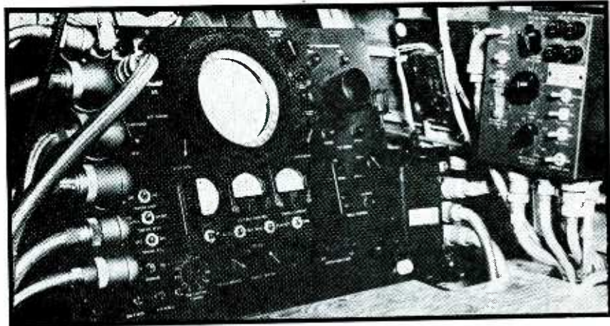
Operator's position at APS-15 installation in a B-17, with range unit and control box at the right of the receiver-indicator with its built-in ppi scope and a small A-scope
