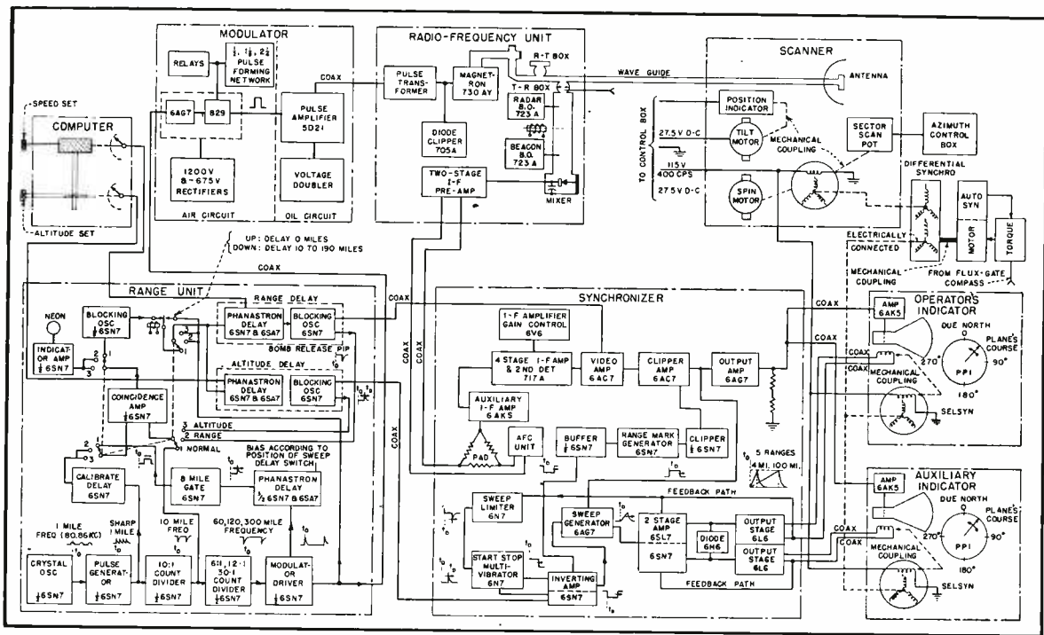
FIG. 1—Block diagram of Western Electric APQ-13 version of H2X bombing radar
