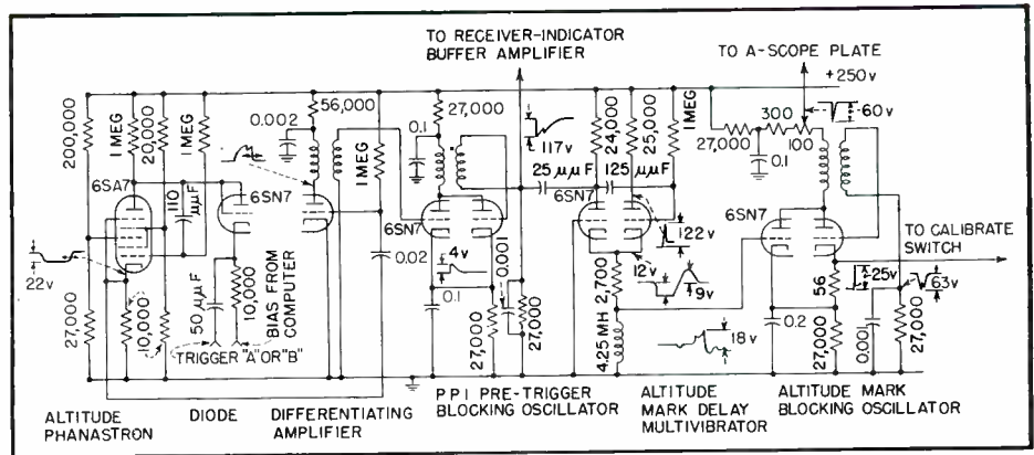
FIG. 6—Altitude phanastron circuit and succeeding stages in APS-15 system, including a one-shot multivibrator serving as altitude mark delay
