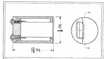
FIG. 2—Microphone consists of a pile of crystal plates within a rigid housing
