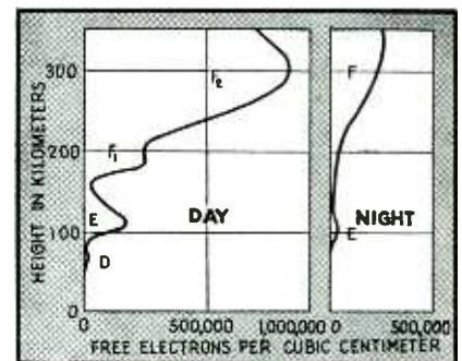
FIG. 2—Night and day distribution of free electrons showing disappearance of the D layer and combination of the F_1 and F_2 layers at night
