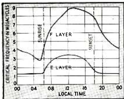
FIG. 6—Critical frequencies for the E and F layers at various times of the day. These plots are particularly important in showing that ionization in the E layer is not entirely dependent upon solar radiation
