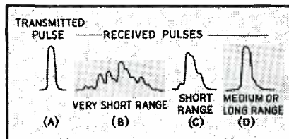
FIG. 11—Within 100 miles of a transmitter the pulses reflected from the E layer are complex and useless for accurate timing techniques. At 300-400 miles, the pulses have achieved sufficient stability
