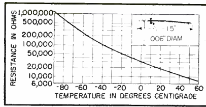
FIG. 3—Effect of temperature on ohmic value of temperature-responsive ceramic resistor used in radiosonde, and closeup view of unit
