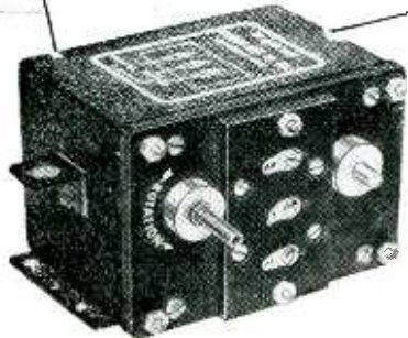
Remote control differential drive for airborne radar computer unit.
