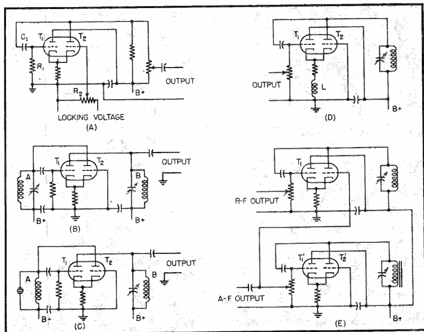
FIG. 4—Five useful circuit arrangements for the two-tube oscillator
