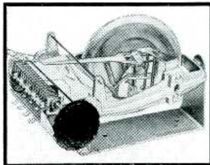
Barometric switch used in radiosondes
