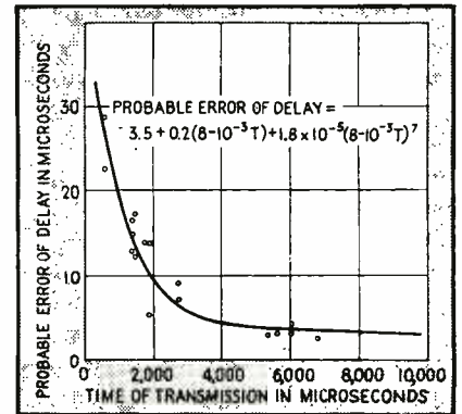
FIG. 13—Probable error of delay has been determined by actual observations at monitor stations of various pairs of transmitters
