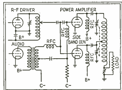
Basic circuit of modulation system for lightweight portable transmitters
