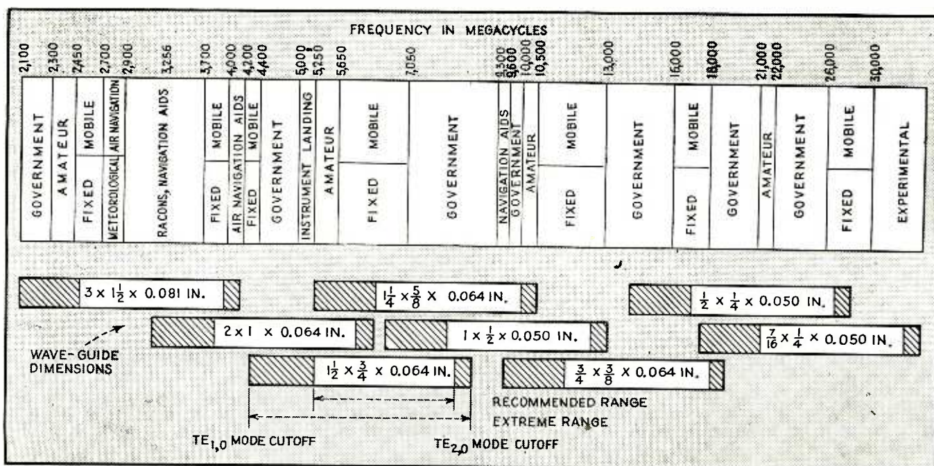
FIG. 2—Federal Communications Commission allocations in the microwave region and standard wave guides suitable for use at various frequencies. Dimensions on the wave guides indicate outside cross section and wall thickness
