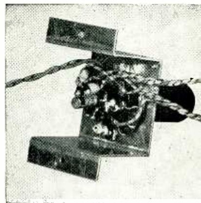
Laboratory model of the simple 100-mc converter made by Electronics Research, Inc. of Evansville, Indiana
