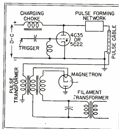
Circuit using a hydrogen thyratron in a line modulator arrangement for pulsing a magnetron
