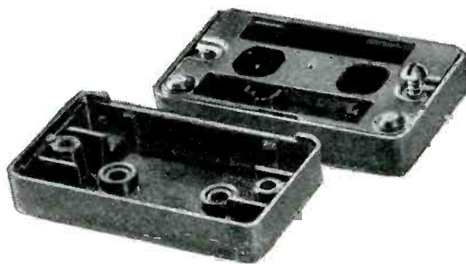
In this typical assembly P-K Type "F-Z" Screws replaced inserts and permitted the use of small, island-bosses without sacrifice of strength.
