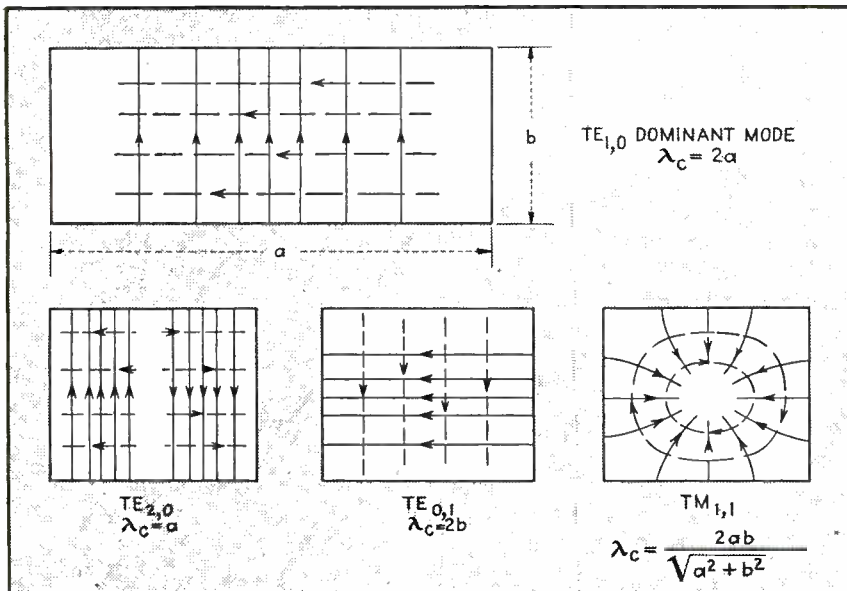
FIG. 1—The distribution of the transverse electric (solid) and transverse magnetic (dashed) waves in wave guides of various rectangular cross sections. The geometry of the guide is usually such that only the dominant mode ( TE_{1,0} ) is above cutoff. A few of the higher modes are shown
