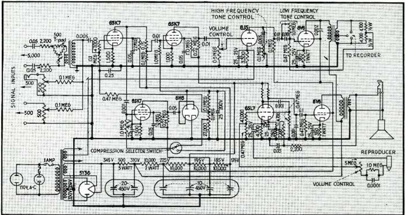
FIG. 3—Recording and reproducing amplifier circuit. Automatic volume compression, and high and low frequency compensation improve intelligibility of low velocity recordings
