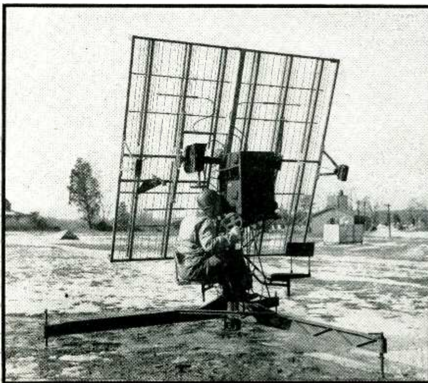
Radio set SCR-658, used for radiosonde tracking to determine wind speed and direction (Signal Corps photo)
