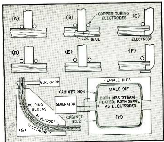
FIG. 6—Electrode arrangements for setting glue in joints
