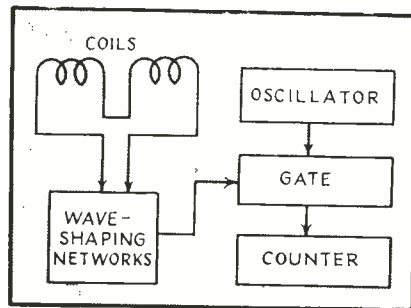
FIG. 2—Block diagram illustrating the basic elements of a chronograph
