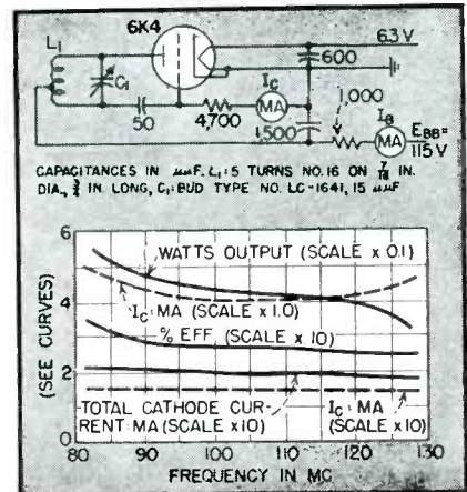
FIG. 4—The 6K4 oscillates stably at vhf in a Hartley circuit
