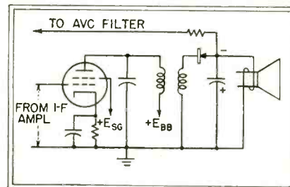
FIG. 1—Metallic-oxide rectifier simplifies audio output circuit
