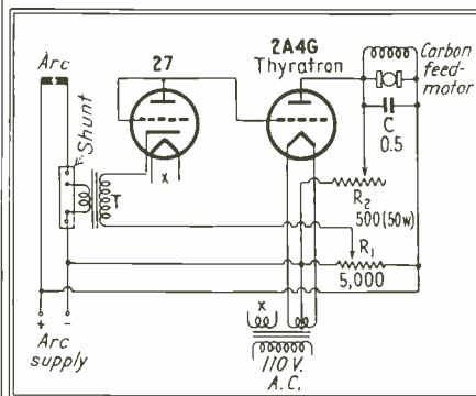
Fig. 2—Carbon arc control circuit
