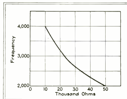
Fig. 3—Oscillator control curve
