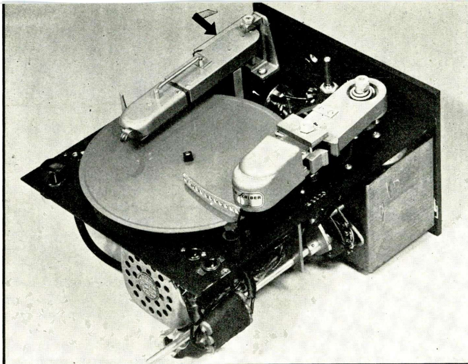
FIG. 1—The SoundScriber office recording machine showing the magnetic recording head at the right and the moving-coil reproducing head at the left. The arrow indicates the spring which neutralizes the tangential forces of the pickup arm
