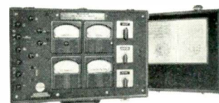
TA Industrial Analyzer—in one case all instruments for a-c data in any industrial plant.
