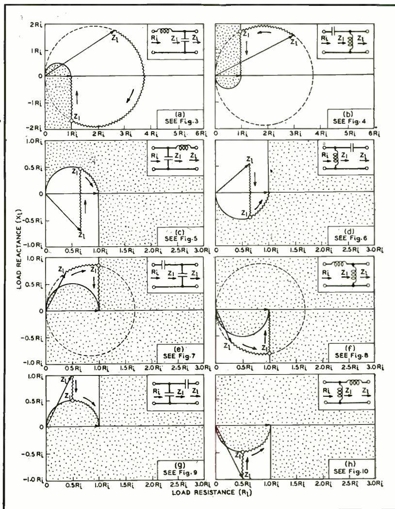
FIG. 2—Any impedance, Z_L , whose vector terminates within an unshaded area on the above diagrams is transformable to a pure resistance, R_L , by means of the circuit to which the diagram applies
