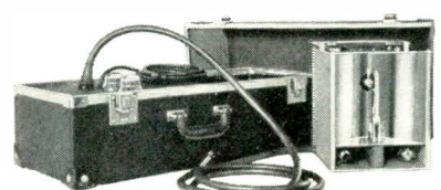
Portable Stroboglow, Type PSE-2, can analyze recurring motions up to a frequency of 30,000 per minute.
