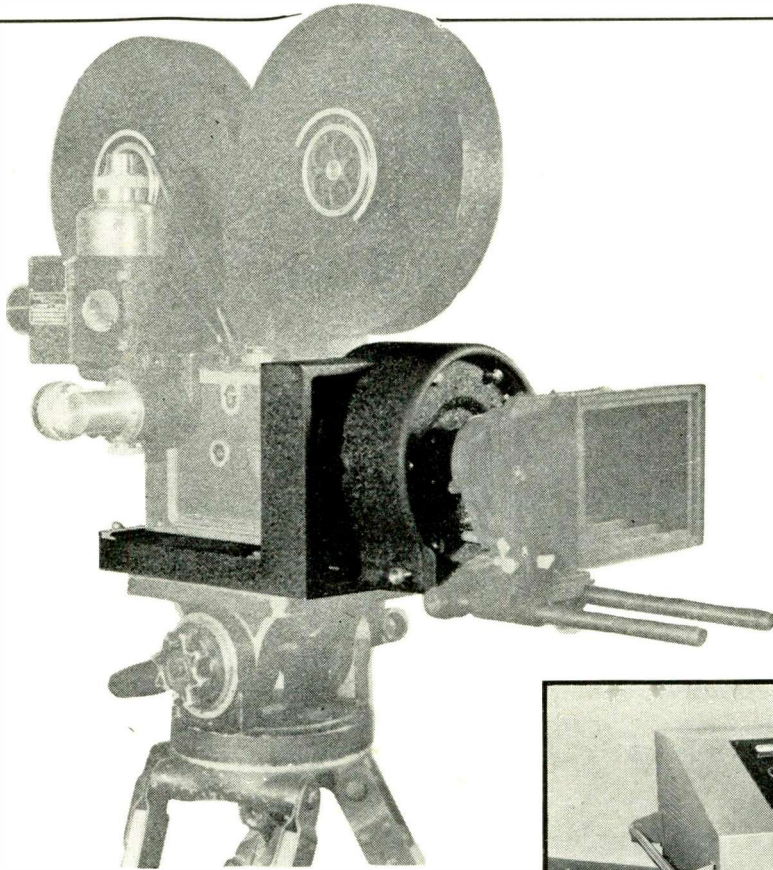
The "lens-motor," substituted for the original lens-turret of a standard motion-picture camera. It contains a 50-mm lens system providing uniform focus from four feet to infinity at full f/3.2 aperture when one element is oscillated. By removing seven screws from the face of the cylindrical part of the casting other objectives may be inserted
