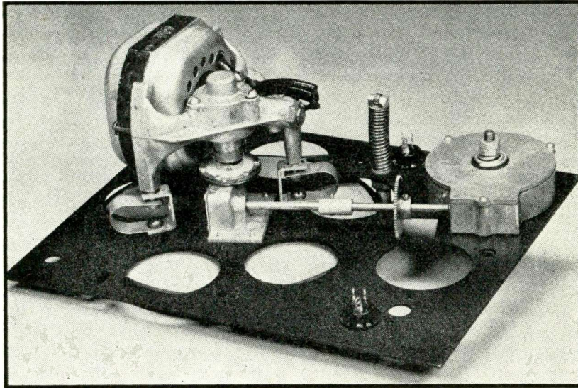
FIG. 5—Bottom of the chassis with the bottom side up. Note the motor mounting and the cutting-head arm drive shaft. Accurately spaced grooves are produced 200 to the inch
