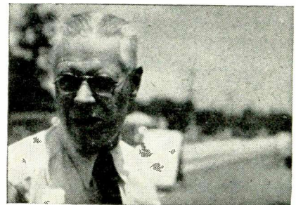
A depth of field comparison. The man is four feet away. Both frames were taken from motion-picture films exposed at f/9 , one with the lens system oscillating and the other with the camera used as a conventional limited-focus device and focussed on the man
