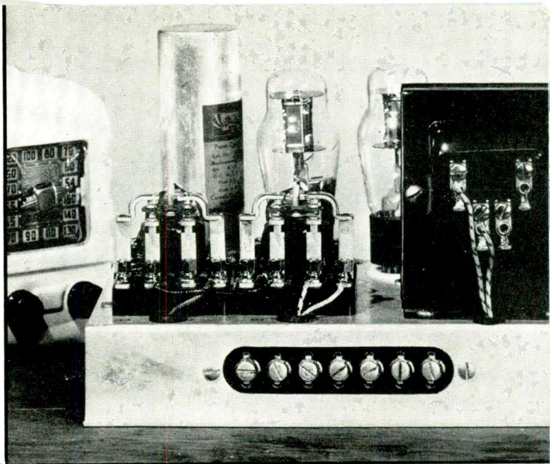
The automatic monitor is contained on the small chassis shown here and may be attached to any set
