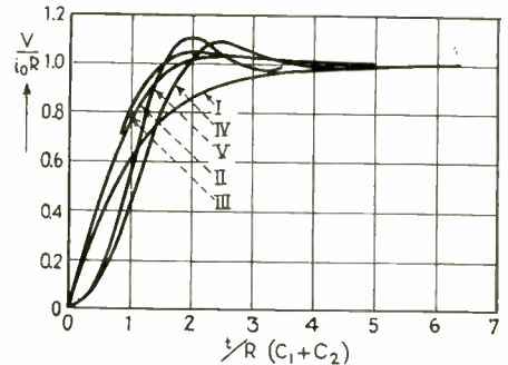
Fig. 3—Transient characteristics of networks of Fig. 1
