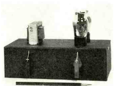
Fig. 1—Completed carbon arc control unit. Pencil in foreground indicates size
