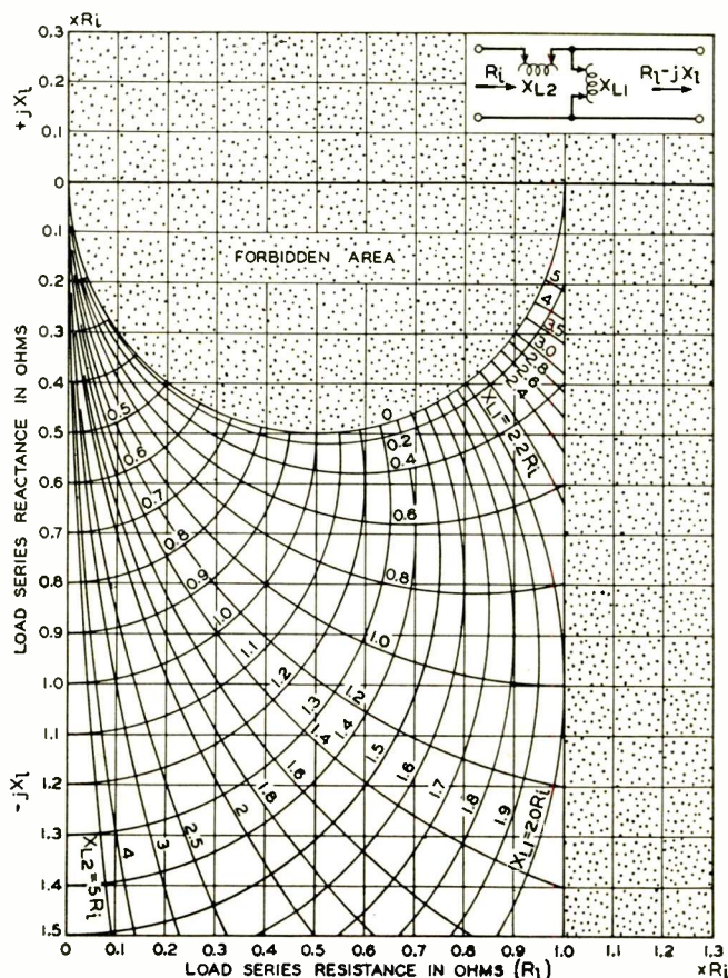
FIG. 8—Series and shunt inductive reactances required to transform load impedance, R_i - jX_i , to pure resistance, R_i .
