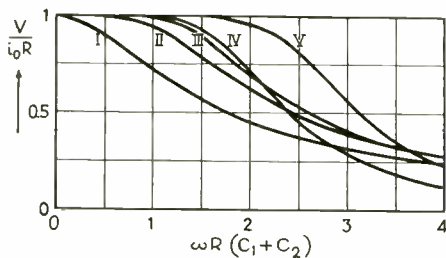
Fig. 2—Amplitude characteristics of networks of Fig. 1
