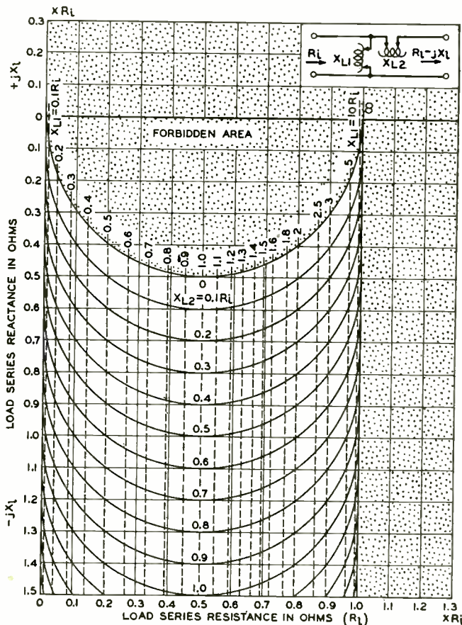
FIG. 10 Shunt and series inductive reactances required to transform load impedance, R_L - jX_L , to pure resistance, R_L .
