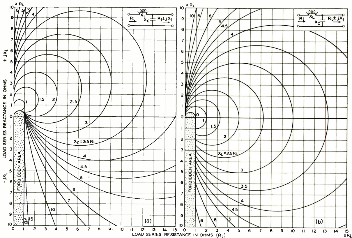
FIG. 3—Shunt reactance, X_c , (left) and series reactance, X_L , (right) required to transform load impedance, R_i \pm jX_i , to a pure resistance, R_i .
