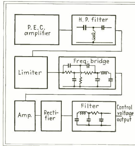
Fig. 4—The discriminator unit
