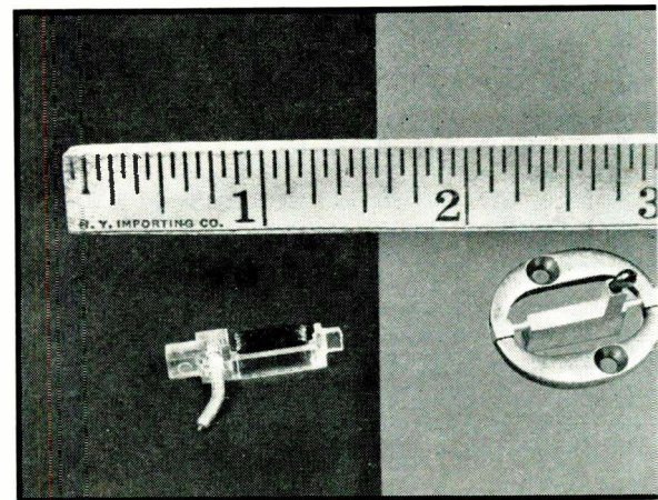
FIG. 7—Pickup unit and coil mounted in a Lucite frame (left) and the cutting head armature (right) mounted in a non-magnetic frame
