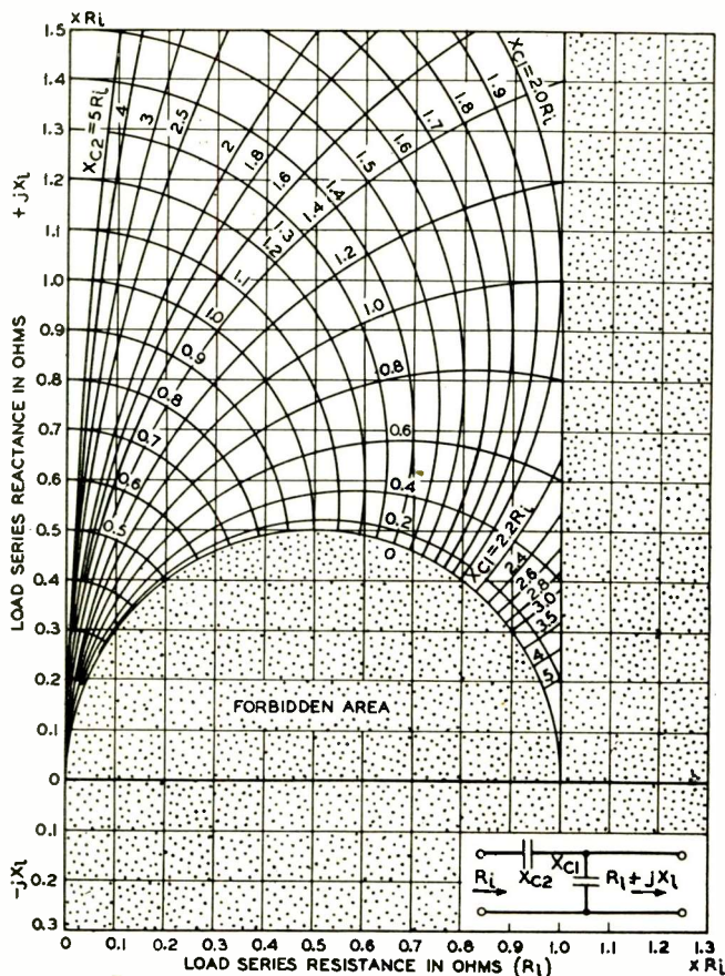
FIG. 7—Shunt and series capacitive reactances required to transform load impedance, R_i + jX_i , to pure resistance, R_i .
