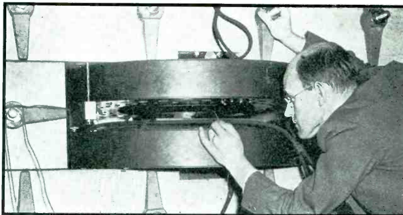
A close-up of the rheotron with W. F. Westendorp of the G-E Research Laboratory making an adjustment
