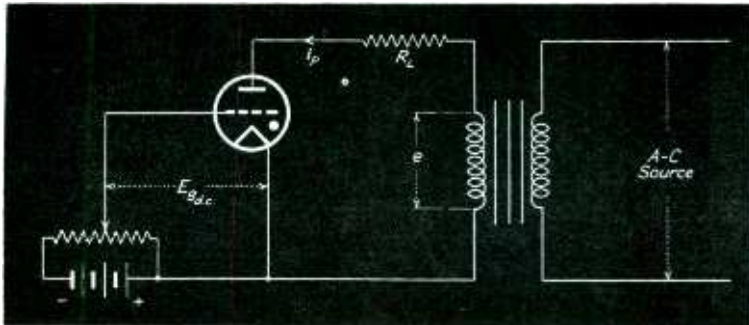
Fig. 3—Simple circuit diagram illustrating amplitude control of the conduction characteristics of gas control tube when plate is fed by alternating current
