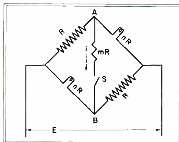
Fig. 1—Schematic diagram of Wheatstone bridge used as voltage regulator
