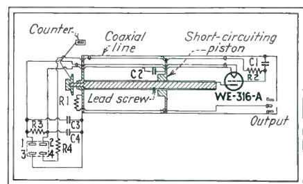
Circuit diagram of 150 to 600 Mc oscillator
