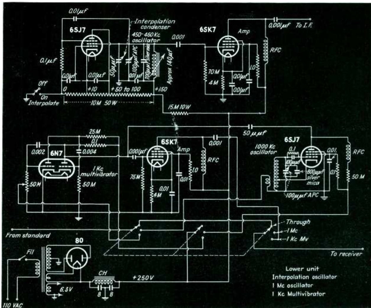
Connections and circuit components are given in this diagram for the interpolation oscillator
