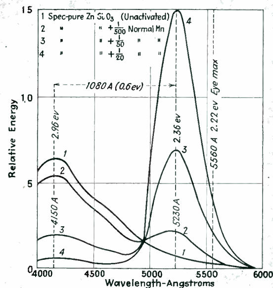
Fig. 3—Curves showing the effect of varying concentration of manganese, used as an activator, on alpha willemite
