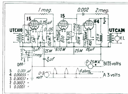
Fig. 1—Schematic circuit of amplifier, using two feedback circuits
