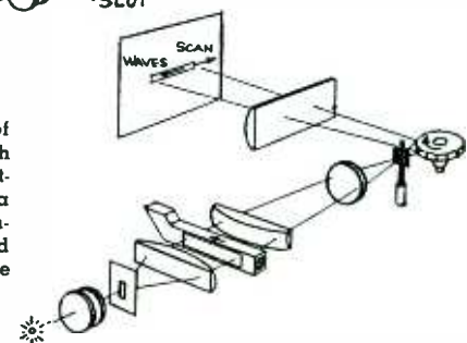
Fig. 4—The elements of Fig. 3 are combined with a multiple mirror rotating wheel to produce a line image whose intensity can be varied with time or with the position of the spot
