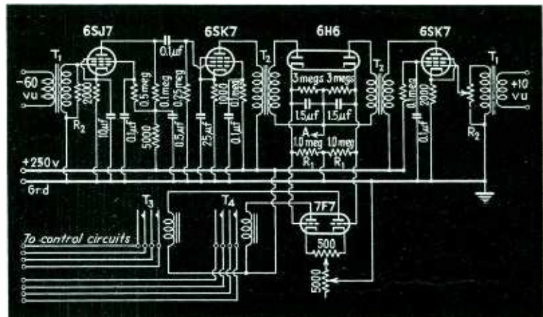
Fig. 3—Circuit diagram of the alarm. The common cathode resistor of the 7F7 increases the sensitivity of this tube as a push-pull d-c amplifier
