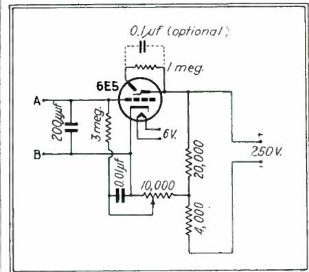
An electron ray indicator tube, connected as indicated above, is useful as a form of electroscop and polarity indicator
