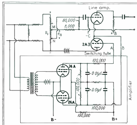
Fig. 2—Circuit diagram of automatic phase reversal amplifier
