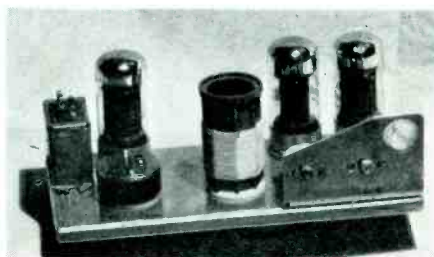
The r-f section, which comprises the top shelf of the transmitter
