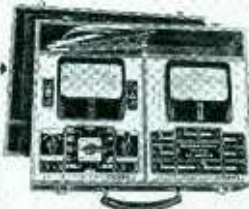
★ Series 844-J Combination AC-DC Industrial Circuit Tester (center illustration). Complete with ohmmeter batteries and high voltage test leads. Furnished in walnut finished hardwood portable case, size 11 x 15 x 6" $48.95
