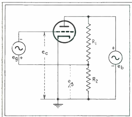
Fig. 1—Simplified circuit of inverse feedback amplifier
