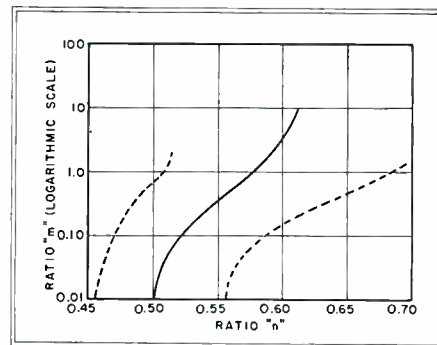
Fig. 2—Ratio of load resistance m to arm resistance n for perfect regulation (solid curve) and good regulation (dotted curves)
