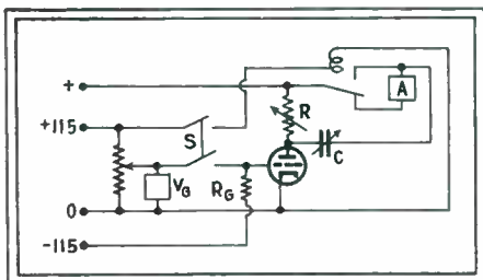
Fig. 2—Circuit for measuring characteristics of a triode
