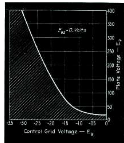
Fig. 1—Control grid characteristics of the RCA-2051 gas tetrode. Conduction cannot occur in the cross-hatched region
