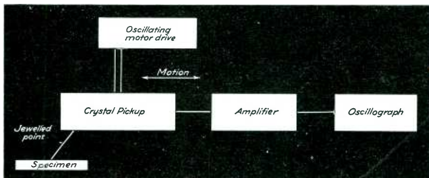
Fig. 2—Block diagram illustrating the principle of the Brush surface analyzer. A diamond point is moved across the surface and any irregularities are shown on the oscillograph
