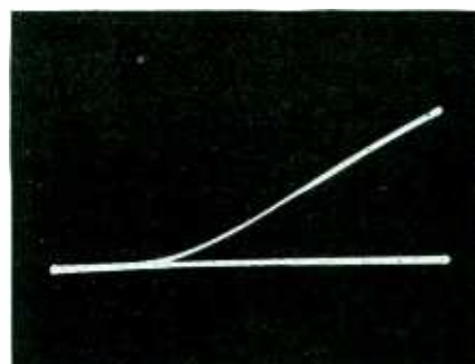
Relation between screen grid voltage and plate current for a 6J7 with control grid at -2 volts
