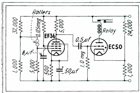
Circuit diagram of pinhole detector
