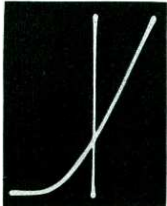
Grid voltage-plate current characteristic of 1G6 tube with plate voltage at 90 volts
