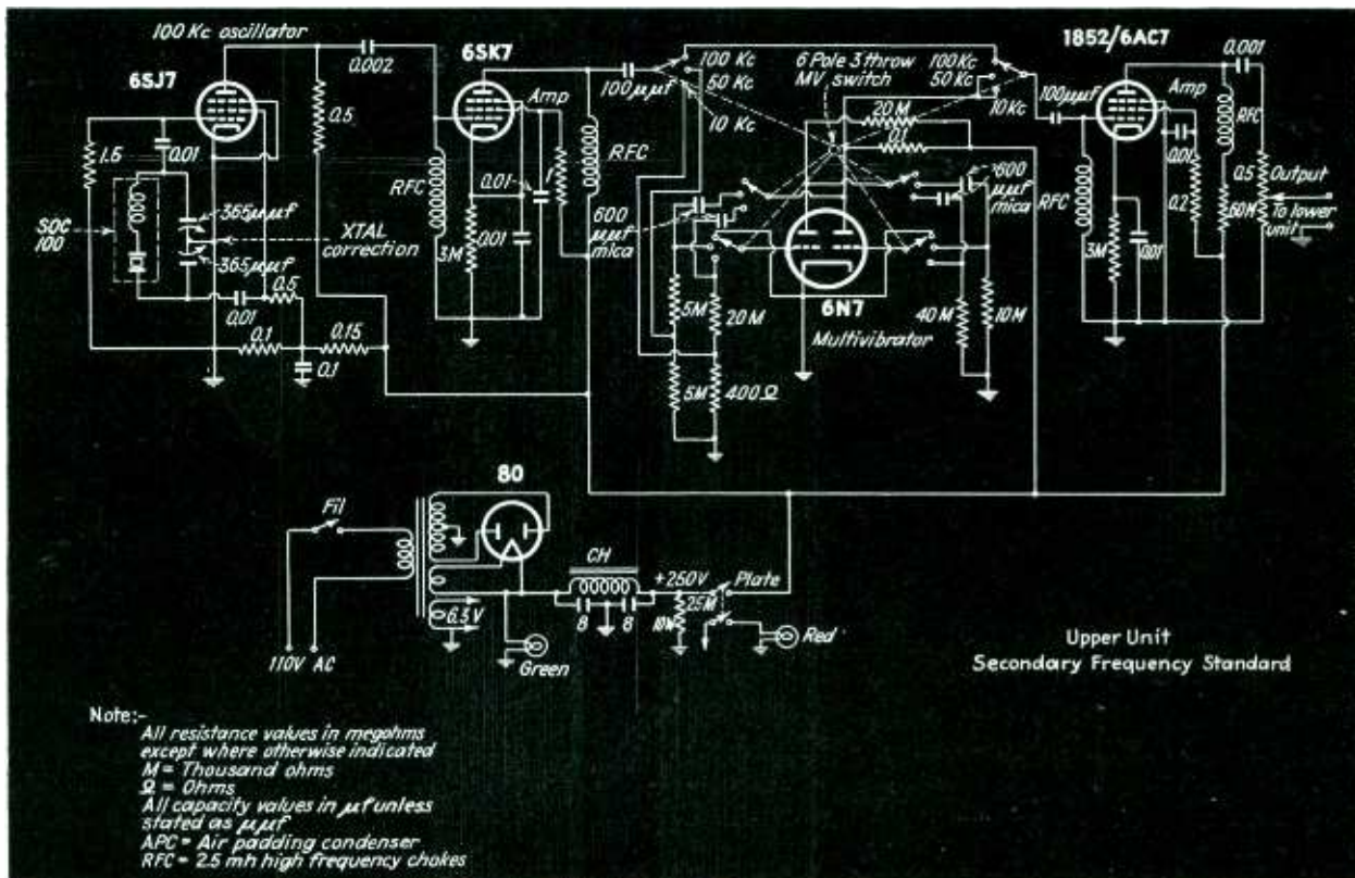
Circuit diagram of the secondary standard of frequency
