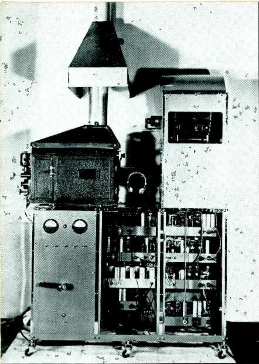
Fig. 7 Complete projector for theater use, based on the principles outlined in this article
