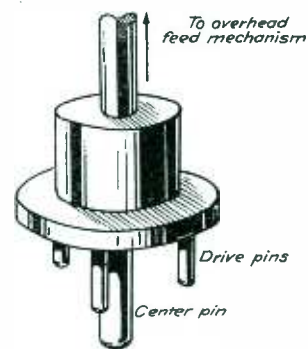
Fig. 3—Some recording machines have the drive pins attached to the flange as shown rather than to the turntable. A rubber pad raises the drive pins above the disc
