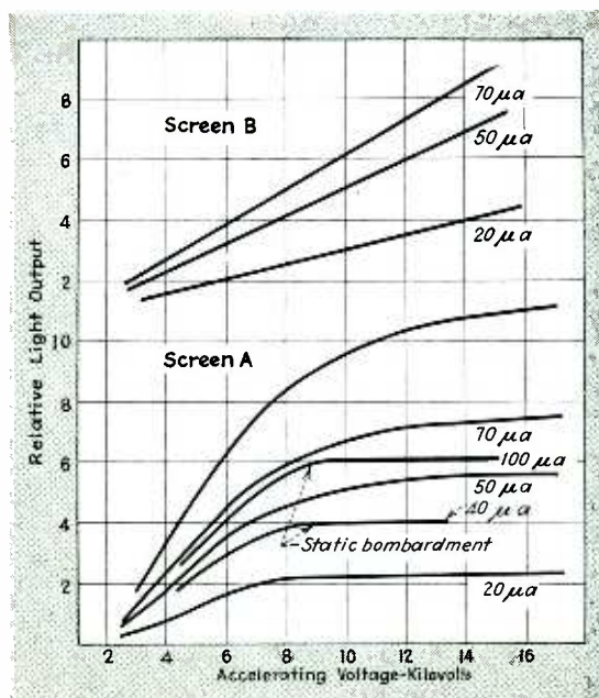
Fig. 7—Relative light output of willemite screens as a function of acceleration voltage
