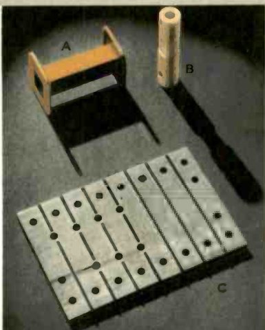
A. Square tube coll form sanded to size; flanges milled, sawed and broached. B. Insulating tube, sawed, drilled, reamed, and milled. C. Sawed, milled and drilled Terminal Panel.
