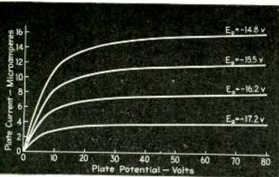
Fig. 3—Plate characteristics of the 6K7 tube. E_b = 6.3 v E_{c2} = 40 v E_{c3} = -6.5 v
