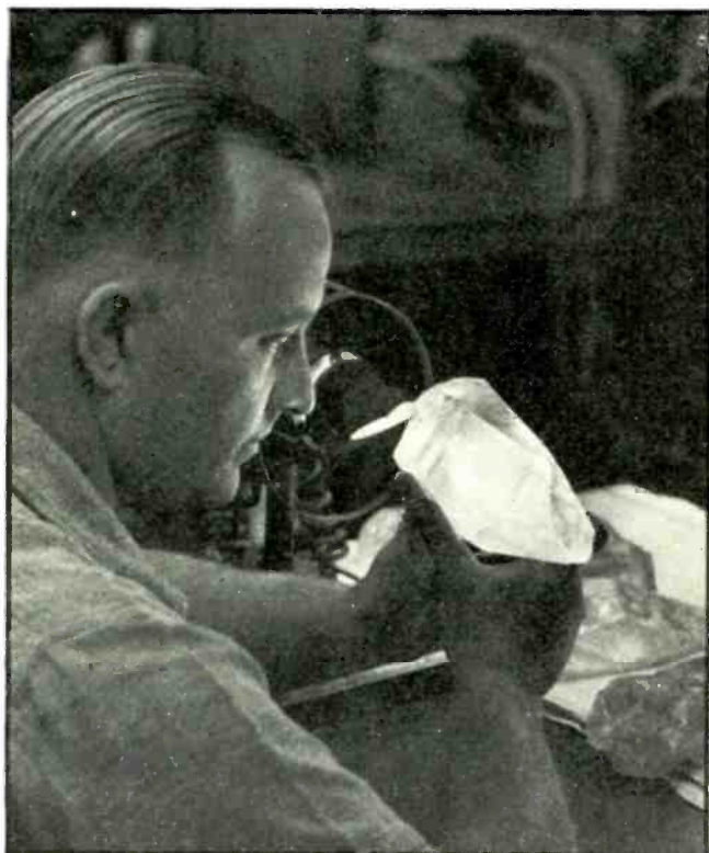
Raw Brazilian quartz crystals, averaging six inches in length and six pounds in weight, are subjected to arc-lamp examination for imperfections and "needles." The imperfections are marked on the raw quartz preliminary to cutting operations
