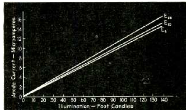
Fig. 2—Light-current characteristic of type VB phototube. The curve for 28 volts represents the current at saturation
