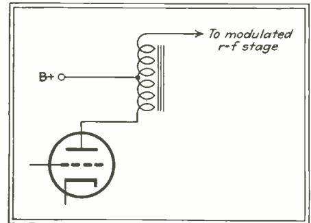
Fig. 4—D-c bucking arrangement to reduce core saturation point
