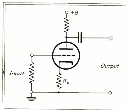
Fig. 1—Basic amplifier section of the voltmeter
