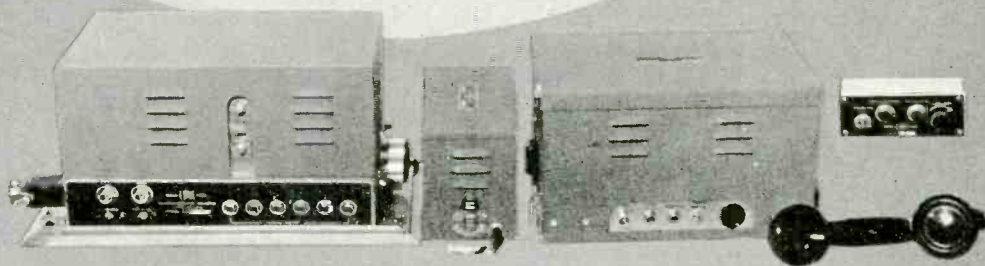
FMTR MOBILE ASSEMBLY Type 25 UFM 25/30 watt transmitter Type 11 UF receiver and power supply
