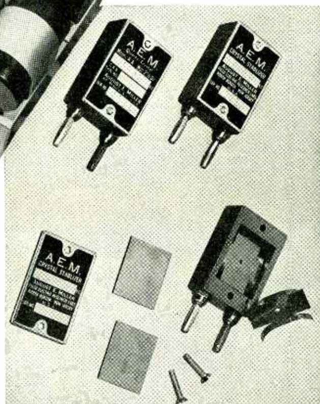
(Below) Monel plates, springs and screws as used in crystal stabilizers made by August E. Miller Co., 1922 Bergenwood Rd., North Bergen, N. J. At left is shown transmitter with stabilizers inserted on chassis.
