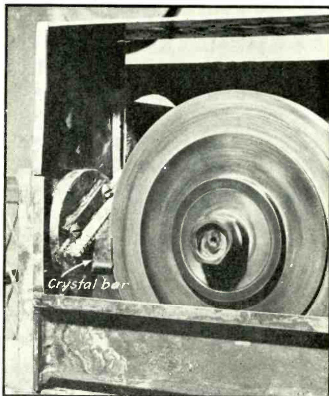
The raw quartz crystals are first cut into bars and then into thin slices called "blanks" at approximately the desired angle, with a gang-saw cutting machine using carborundum abrasive. Great care must be taken to maintain the correct angle
